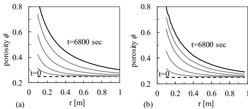
Figure 6.2 Spatial profiles of porosity at various times: (a) Results of Stavropoulou et al. 1998; (b) Results of Stavropoulou et al. [38]
