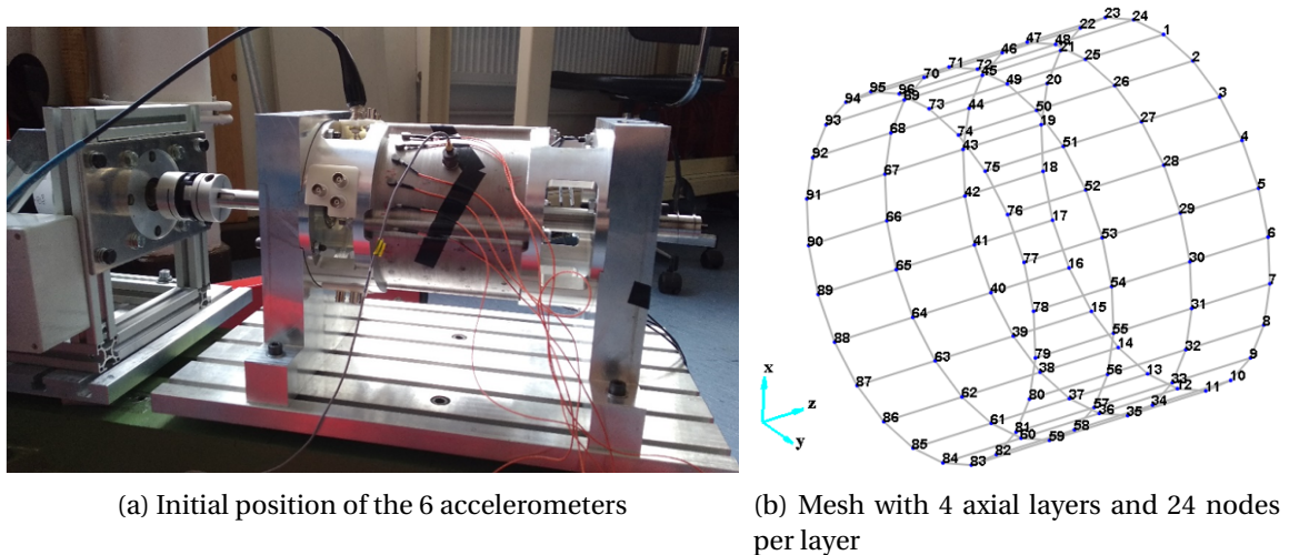
Figure 5.26 – ODS measurement setup with 6 roving accelerometers for a total of 96 nodes.
