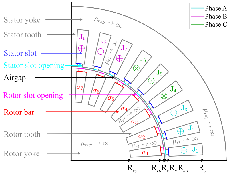
Figure 4.23 – SCIM 36s28r4p studied topology and assumptions
