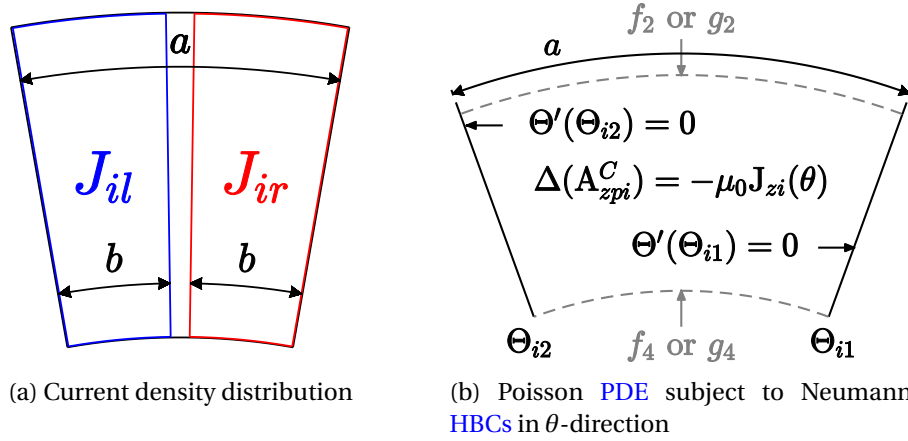
Figure 3.23 – Subdomain problem for slotted windings with double layer in \theta -direction.
