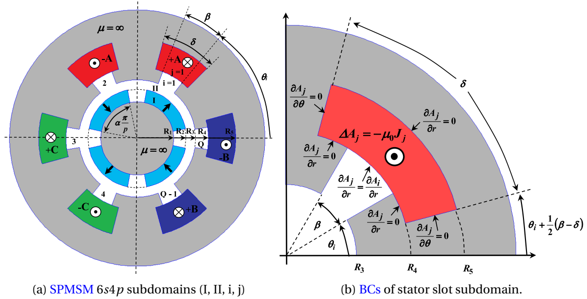
Figure 2.12 – Subdomain model of a SPMSM 6s4p (from Lubin et al. [2011a])
