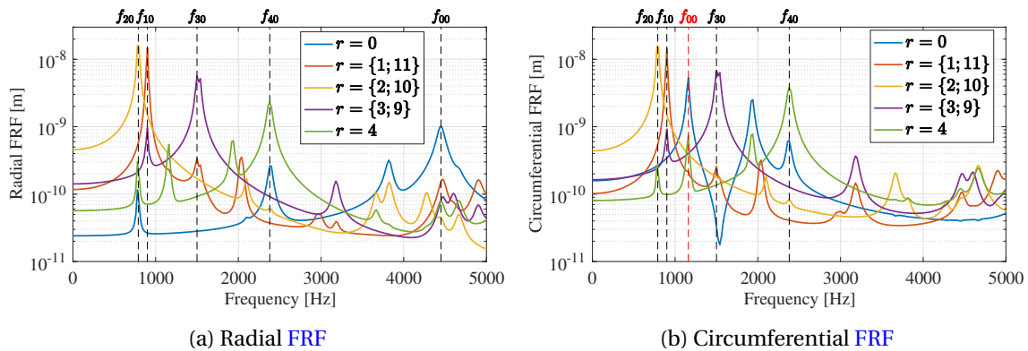
Figure 5.10 – Radial and circumferential FRFs obtained from FEA (MANATEE Optistruct).
