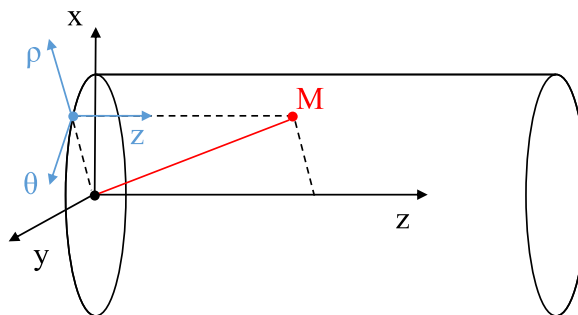
Figure A.1 – 3D cylindrical coordinate frame
