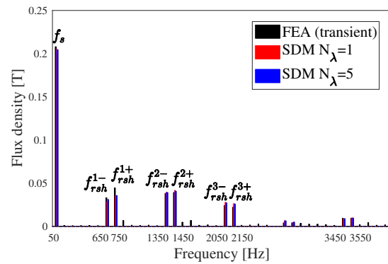
(d) Circumferential FFT over one mechanical period for \theta = 4^\circ
