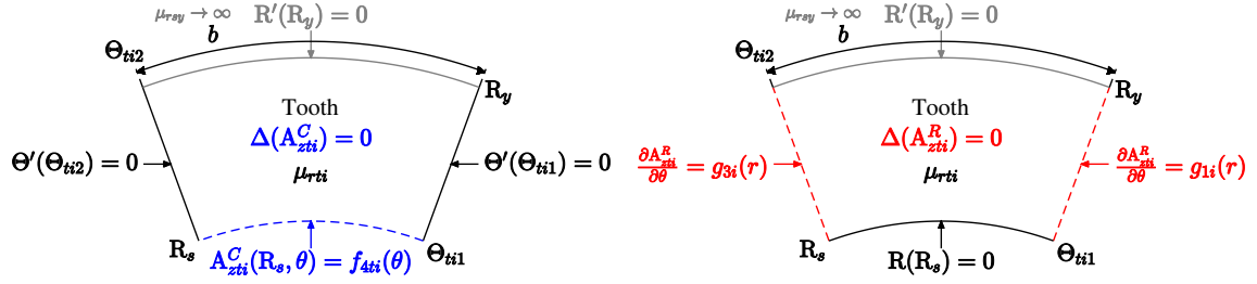
(a) Eigenvalue problem in \theta -direction with Neumann HBCs, where f_{zti} is given by Equation (4.52). (b) Eigenvalue problem in r -direction with Neumann HBCs, where g_{zi} , g_{3i} is given by Equations (4.58)-(4.59).
