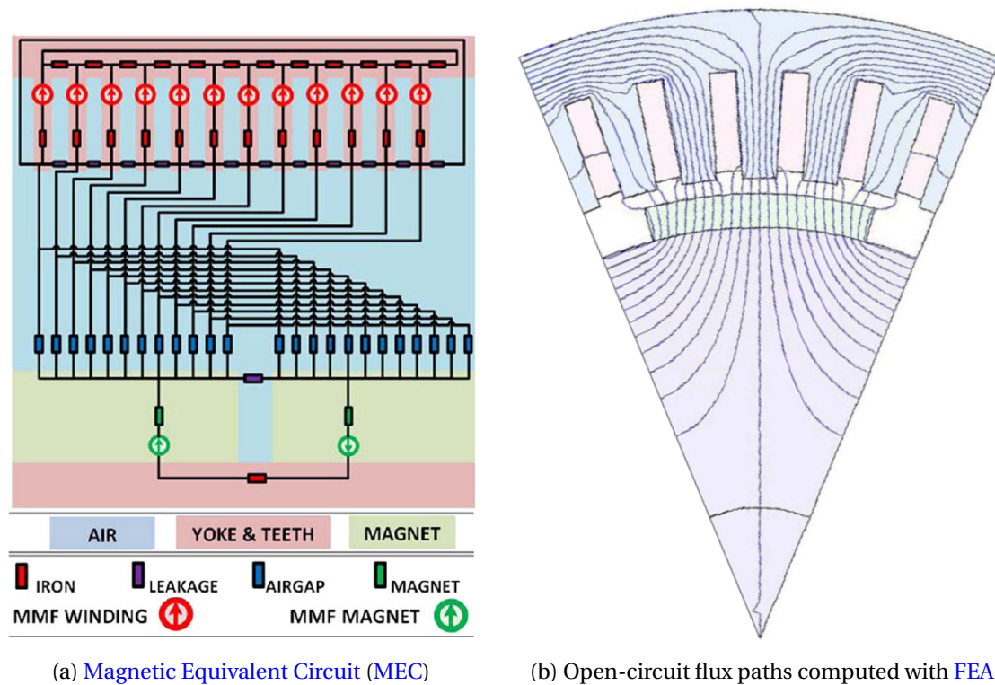
Figure 2.14 – Example of SPMSM Magnetic Equivalent Circuit (MEC) (from Bracikowski et al. [2012]).
