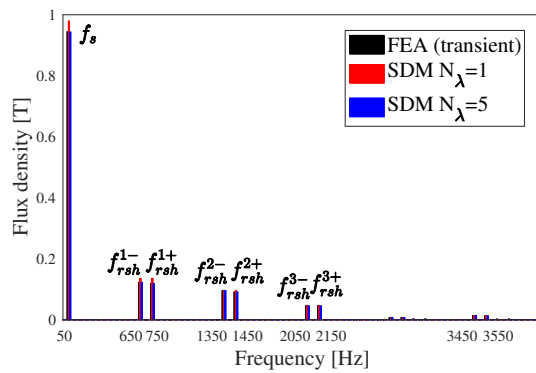
(c) Radial FFT over one mechanical period for \theta = 0^\circ
