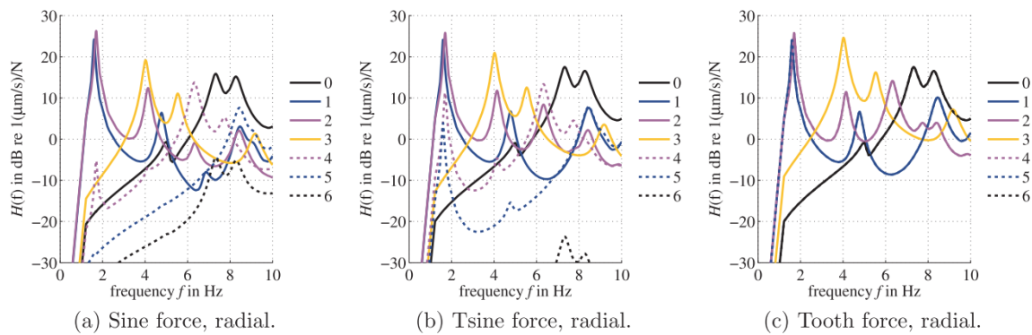
Figure 2.22 – Numerical radial FRFs with 3D FE structural model using three MST projections (from Boesing [2013]).
