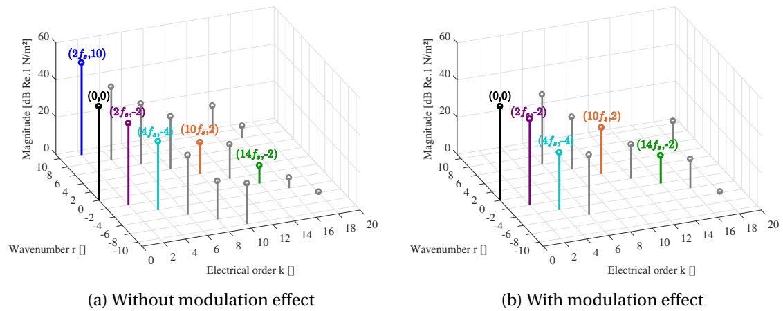
Figure 5.34 – Time and space harmonic content of radial airgap stress with and without slotting modulation effect assuming ideal rotor magnetization.
