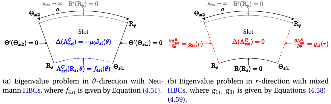
Figure 4.10 – Superposition principle for MVP PDE in stator slots subdomains assuming teeth finite permeability and yoke infinite permeability.
