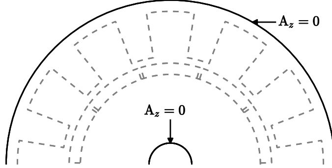
Figure 3.6 – Dirichlet HBCs applied on external boundaries of stator and rotor yokes, implying zero radial flux density at the interface.
