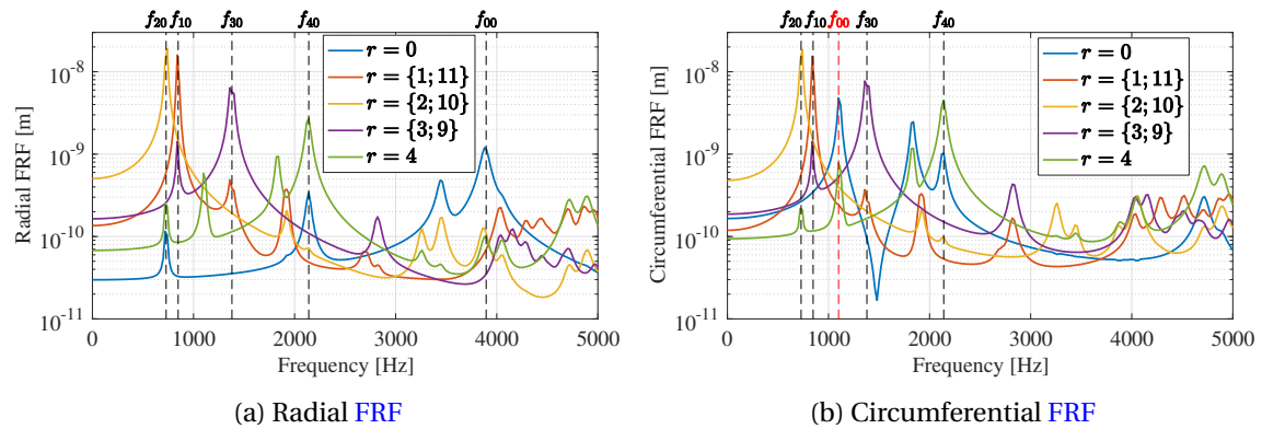
Figure 5.24 – Radial and circumferential FRFs obtained from FEA (MANATEE Optistruct) with fitted elastic properties (cf. Table 5.6).
