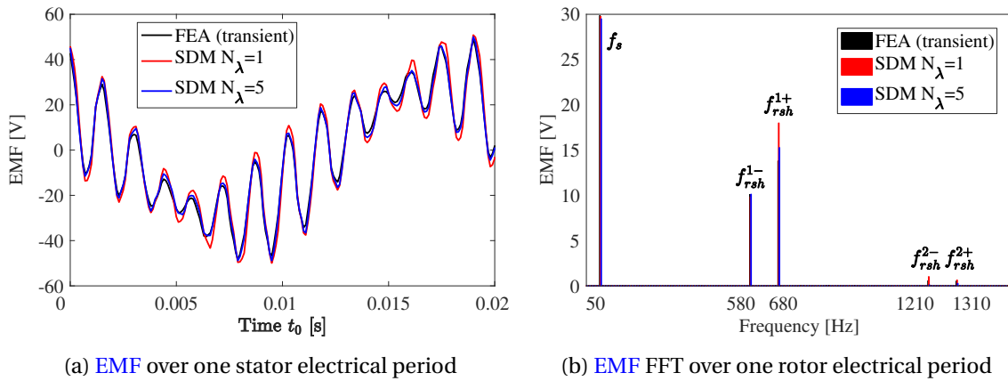
Figure 4.38 – EMF in Phase A over time and FFT for slip s = 10\% .
