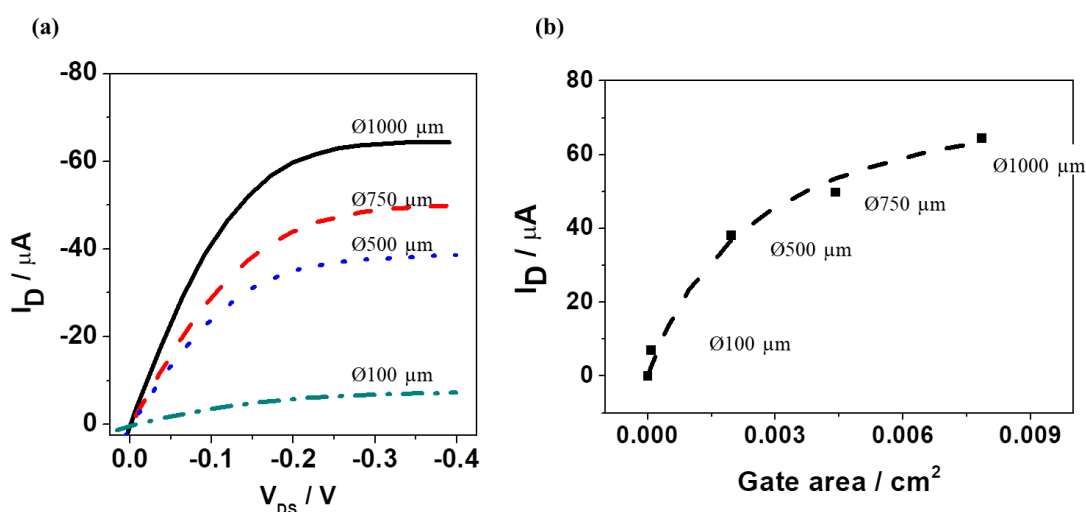
Figure 3. (a) Output curves of a DPP-DTT EGOFET for different gate diameters ( black solid curve: 1000 \mu\text{m} ; red dashed curve: 750 \mu\text{m} ; blue dotted curve: 500 \mu\text{m} ; green dash-dotted curve: 100 \mu\text{m} ). The drain potential was swept at 170 \text{mV s}^{-1} . V_{GS} = -0.4 V. L = 10 \mu\text{m} ; W = 10 mm. Electrolyte: air-saturated MilliQ water. (b) Solid square: Saturation current ( I_{Dsat} ) as a function of the gate area, extracted from Fig. 3a; Dotted line: fitting of I_D as a function of the gate area, for a fixed value C_{OSC/Elec} = 35 \pm 15 nF and a gate capacitance C_{Elec/Gate} = 40 \pm 7 \mu\text{F cm}^{-2} .
