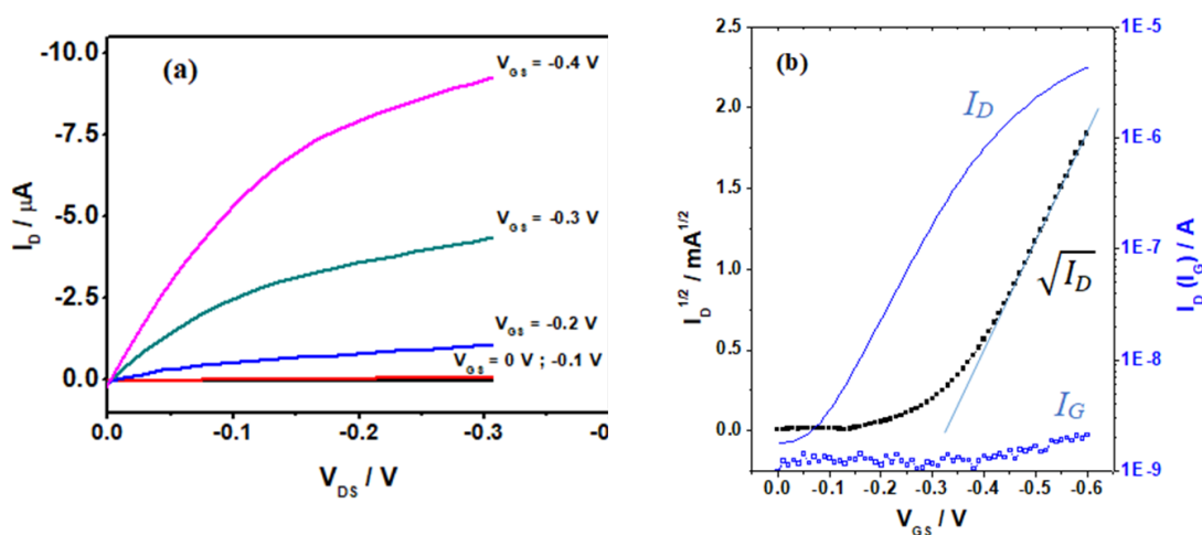
Figure 4. (a) Output curves of a DPP-DTT EGOFET (gate \Phi : 100 \mu\text{m} ) for various gate voltages from 0 \text{ V} down to -0.4 \text{ V} . The drain potential was swept at 170 \text{ mV s}^{-1} . (b) Corresponding transfer curve (solid line) obtained by sweeping the gate voltage from 0 \text{ V} down to -0.6 \text{ V} at a scan rate of 170 \text{ mV s}^{-1} at a fixed V_{DS} = -0.4 \text{ V} ; corresponding plot of \sqrt{I_D} = f(V_{GS}) (solid squares); corresponding plot of I_G = f(V_{GS}) (open squares). L = 10 \mu\text{m} ; W = 10 \text{ mm} . Electrolyte: air-saturated MilliQ water.
