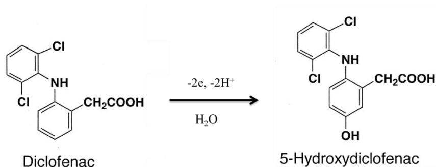
Figure II.7. Oxidation mechanism of DCF
