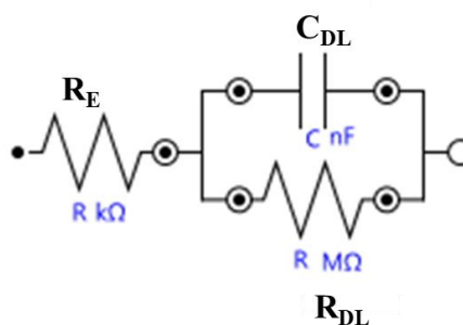
Figures SI-3. The equivalent circuit used for fitting the EIS spectra of the modified gates
