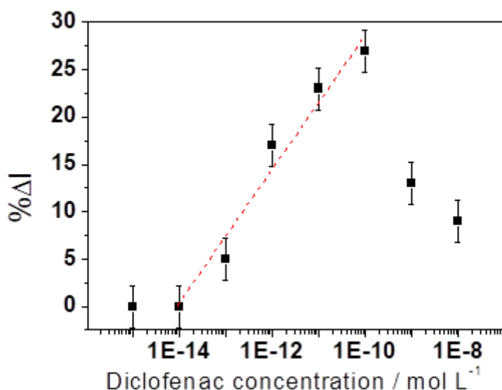
Figure 6. Calibration curve corresponding to the relative current change percentage ( 100 \times \Delta I / I_0 ) measured at -0.45 V vs SCE, after addition of DCF, for concentrations from 10^{-15} M up to 10^{-8} M in PBS. \Delta I = I_{\text{after displacement}} - I_{\text{before displacement}} and I_0 = I_{\text{before displacement}} .
