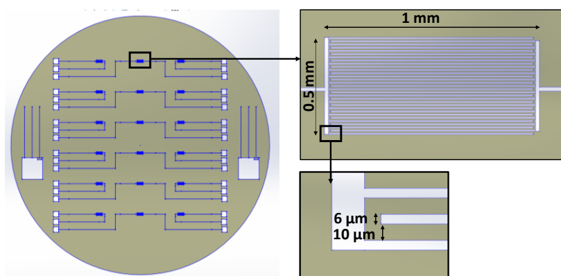
Scheme SI-1. View of (left) a 2 inches Si wafer onto which 18 transistors (interdigitated source and drain) are lithographed and (right), details of the device dimensions, including the digit width (6 \mu\text{m} ) and the channel length (10 \mu\text{m} ). The total channel width is 30000 \mu\text{m} .
