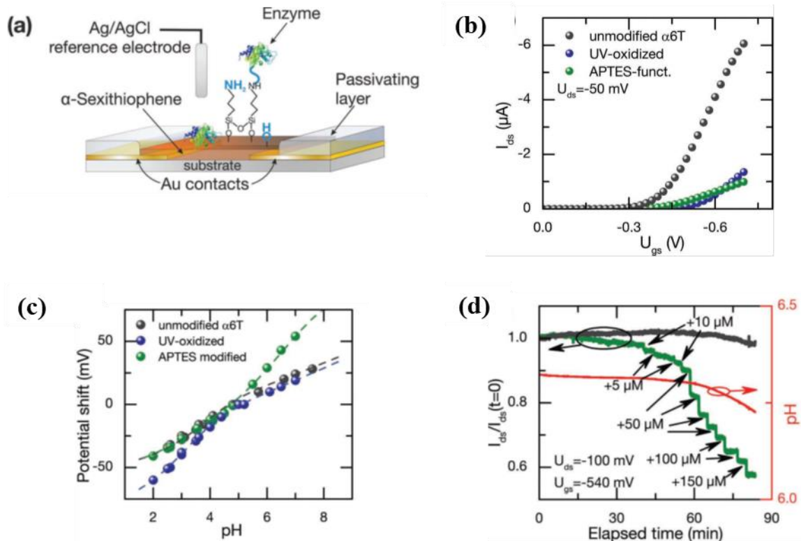
Figure I.24. The EGOFET described by Buth et al. (2012): (a) Schematic drawing of the transistor architecture and the different functionalizations investigated. (b) Transfer curves of untreated, oxidized and APTES-functionalized transistors, measured at pH 5. (c) Threshold voltage shift of untreated, APTES-functionalized and UV-oxidized \alpha 6T as a function of pH. (d) I_D versus time, during a penicillin titration in PBS buffer. The green line corresponds to the response of a device functionalized with APTES and penicillinase, while the grey line depicts the I_D response of an untreated \alpha 6T (141) .
