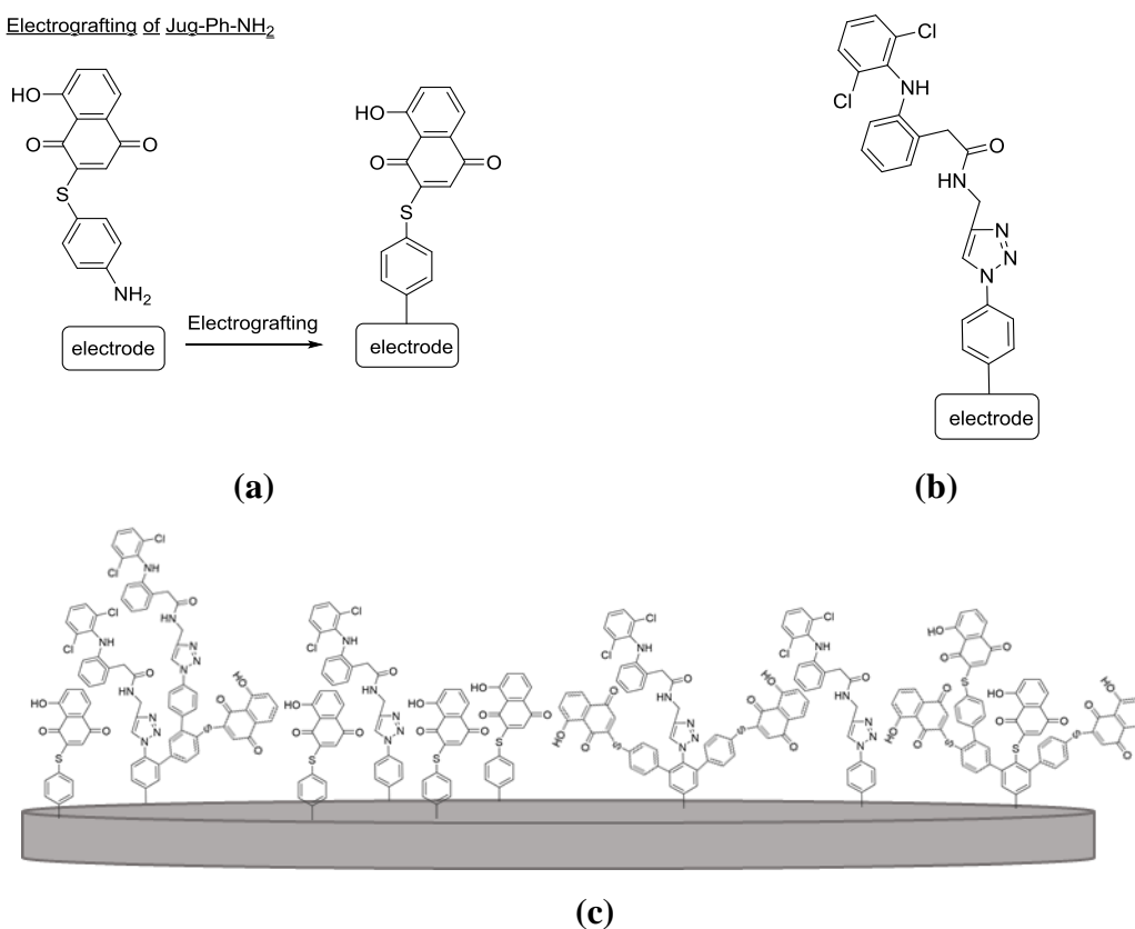
Figure S13. Principle of electrografting of (a) the redox probe E-Probe and (b) the molecular probes DCF-Probe on glassy carbon (GC) electrodes. In-situ formation of the corresponding diazonium salts is not shown in this figure. (c) Possible grafting route.
