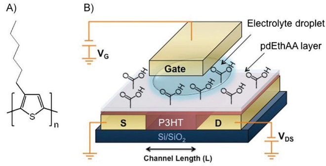
Figure I.26. P3HT organic semiconductor: (A) Chemical structure. (B) Schematic view of an electrolyte gated organic field-effect transistor with the pdEthAA coating deposited by PE-CVD on the P3HT layer (151) .
