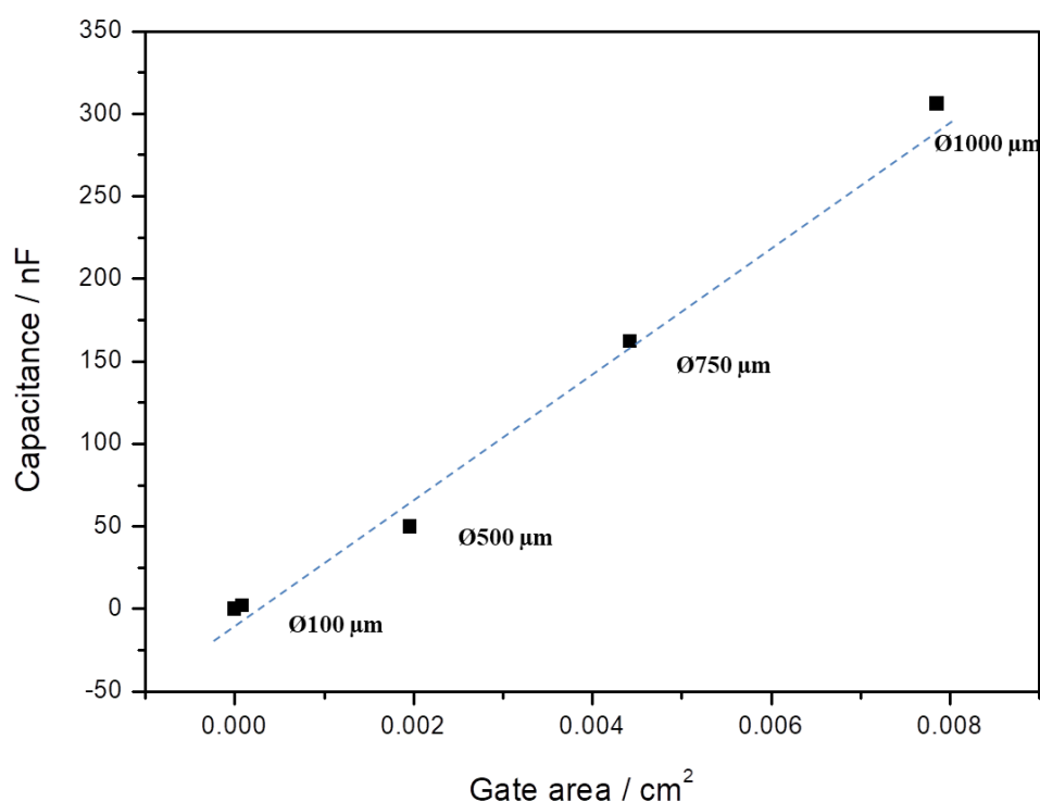
Figure SI-5. (black squares) Capacitances of the bare gold gate electrodes as a function of their area. (blue dotted line) Expected linear behavior. Capacitances were measured by EIS in a three-electrode electrochemical cell with PBS as electrolyte.
