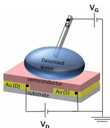
Figure I.17. Scheme of the first water-gated EGOFET. The semiconductor was rubrene and the gate a platinum wire (109) .
