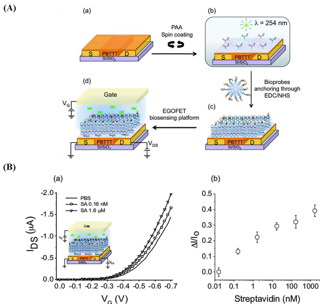
Figure I.31. pBTTT-based EGOFET for protein (streptavidin) detection: (A) Schematic illustration of the fabrication process of an EGOFET biosensor. (a) after deposition of pBTTT on the substrate; (b) poly(acrylic acid) coating spin-coated and cross-linked ; (c) biotinylated phospholipids anchored on the PAA coating; (d) EGOFET configuration comprising a gold gate electrode and a droplet of PBS as dielectric. (B) (a) I_{DS} – V_G transfer curves in PBS, pH 7.4 (line), and streptavidin solutions at concentrations of 0.16 nM (circles) and 1.6 \mu M (triangles) in PBS; (b) relative response of the EGOFET as a function of the streptavidin concentration (155) .
