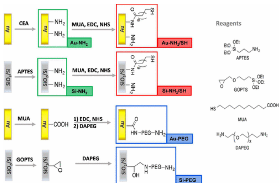
Figure II.8. Surface functionalization strategies for immobilization of AuNPs on gold and silicon substrates (19) .
