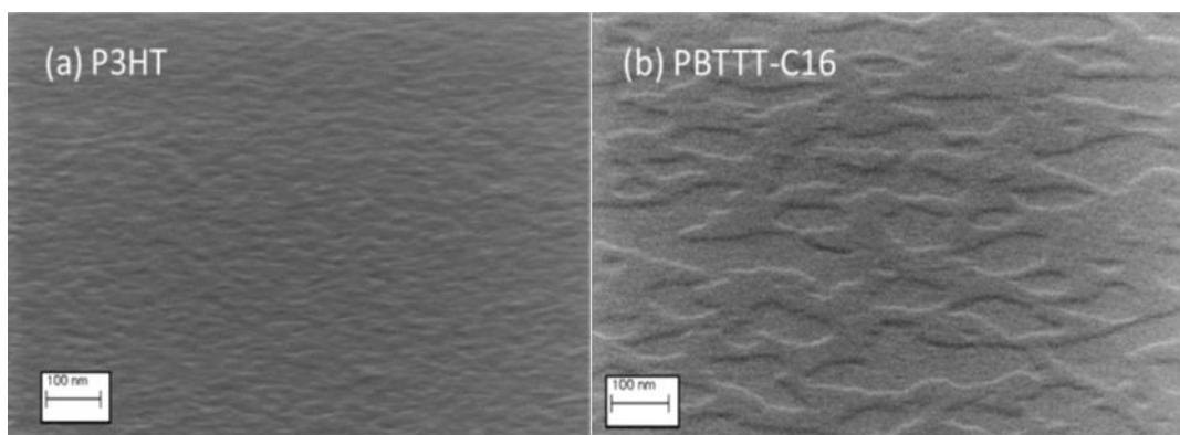
Figure I.20. Lamellar structure of P3HT(a), pBTTT-C16 (b), normal or parallel to the substrate (133) .
