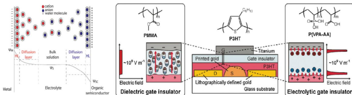
Figure I.16. Illustration of the compact and diffuse layers corresponding to an OFET and an EGOFET, respectively (96) .
