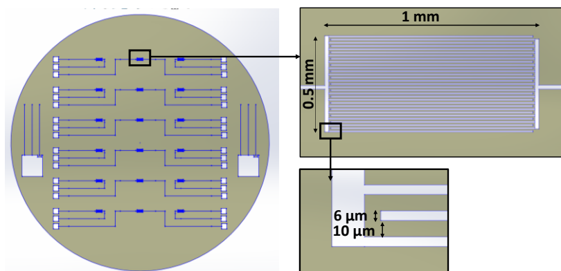
Scheme SI-1. View of (left) a Si wafer onto which 18 transistors (interdigitated source and drain) are lithographed and (right) details of the device dimensions, including the digit width ( 6\ \mu\text{m} ) and channel length ( 10\ \mu\text{m} ). The total channel width is 10000\ \mu\text{m} .
