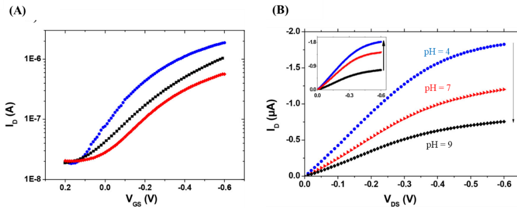
Figure IV.7. Electrical characteristics of an EGFET with a hydrogel-modified gate electrode: (A) Transfer curves ( V_{DS} = -0.6 V) of a (●) bare Au-gated, (■) BrBD-functionalized, and (♦) AA-functionalized EGFET. In all cases, the electrolyte was PBS. (B) Output curves ( V_{GS} = -0.6 V) of a PAA-functionalized EGFET at different pH (6) .
