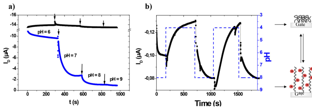
Figure IV.8. Plots of I_D for an EGFET with a hydrogel-modified gate electrode, versus time: (a) ( V_{GS} = V_{DS} = -0.4 V) performed using a (black line) bare gate electrode and (blue line) a PAA-functionalized gate for successive pH jumps (values indicated on the graph); each arrow indicates injection of NaOH. (b) pH was abruptly varied from 8 to 4 and then back to 8 (twice) (6) .
