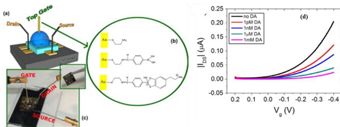
Figure III.10. EGOFET for dopamine sensing: (a) Scheme of the EGOFET device. (b) Gate functionalization with (1) CA, (2) BA and (3) dopamine. (c) Picture of the device. (d) Transfer curves acquired in the linear regime, for various dopamine concentrations (29) .
