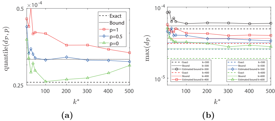
Figure 3.5: The discrepancy \| \mathbf{r}(\mathbf{u}_r(\mu); \mu) \|_{U'}^2 - (\| \mathbf{r}(\mathbf{u}_r(\mu); \mu) \|_{U'}^{\Theta^*})^2 \|^{1/2} between the residual error and the sketched error estimator with \Theta , and the upper bound of this value computed with (3.62). (a) The exact discrepancy for \Theta with k = 500 rows, the upper bound (3.62) of this discrepancy taking \| \cdot \|_{U'}^{\Theta^*} = \| \cdot \|_{U'} , and quantiles of probabilities p = 1, 0.5 and 0 (i.e., the observed maximum, median and minimum) over 20 realizations of the (probabilistic) upper bound (3.62) versus the size of \Theta^* . (b) The exact discrepancy, the upper bound (3.62) taking \| \cdot \|_{U'}^{\Theta^*} = \| \cdot \|_{U'} , and the maximum of 20 realizations of the (probabilistic) upper bound (3.62) versus the number of rows k^* of \Theta^* for varying sizes k of \Theta .
