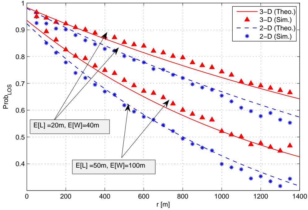
Figure 4.4: Probability of LOS: 2-D modeling vs. 3-D modeling with different E[L] and E[W] .
