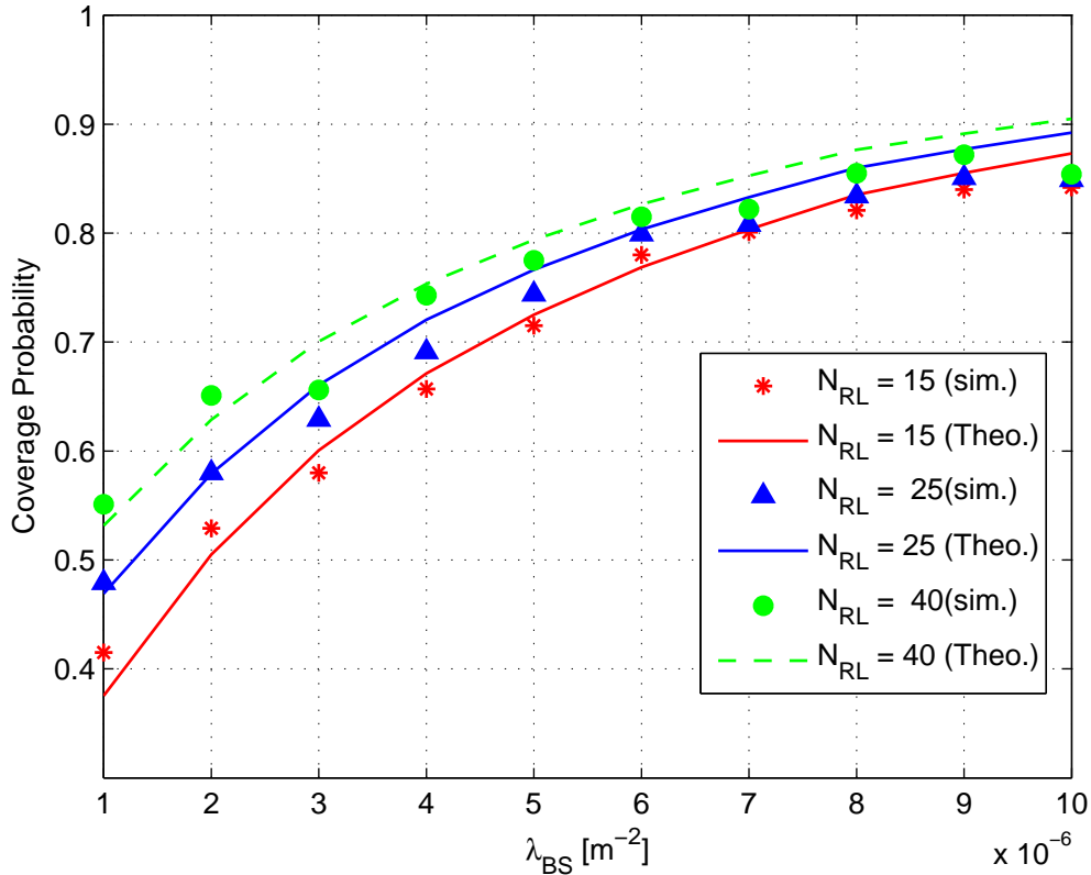
Figure 6.3: successful transmission probability of the min/max based scheme vs. \lambda_{BS} for different values of N_{RL} .
