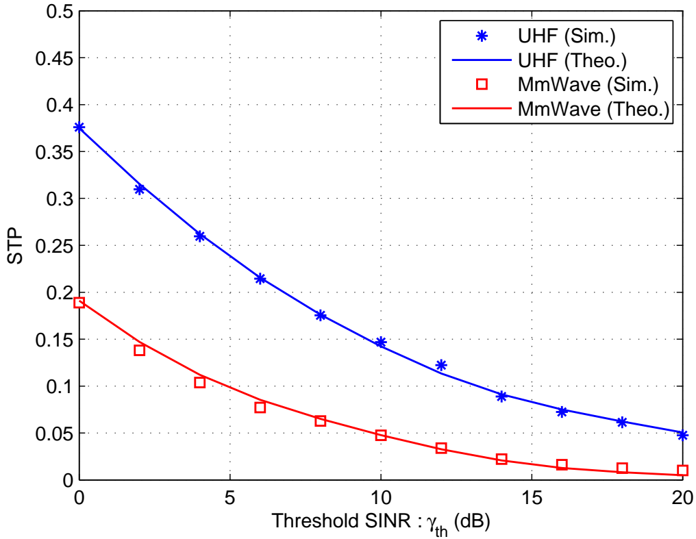
Figure 3.4: Average successful transmission probability vs. \gamma_{\text{th}} for different values of \alpha , and \eta = 0.3 .
