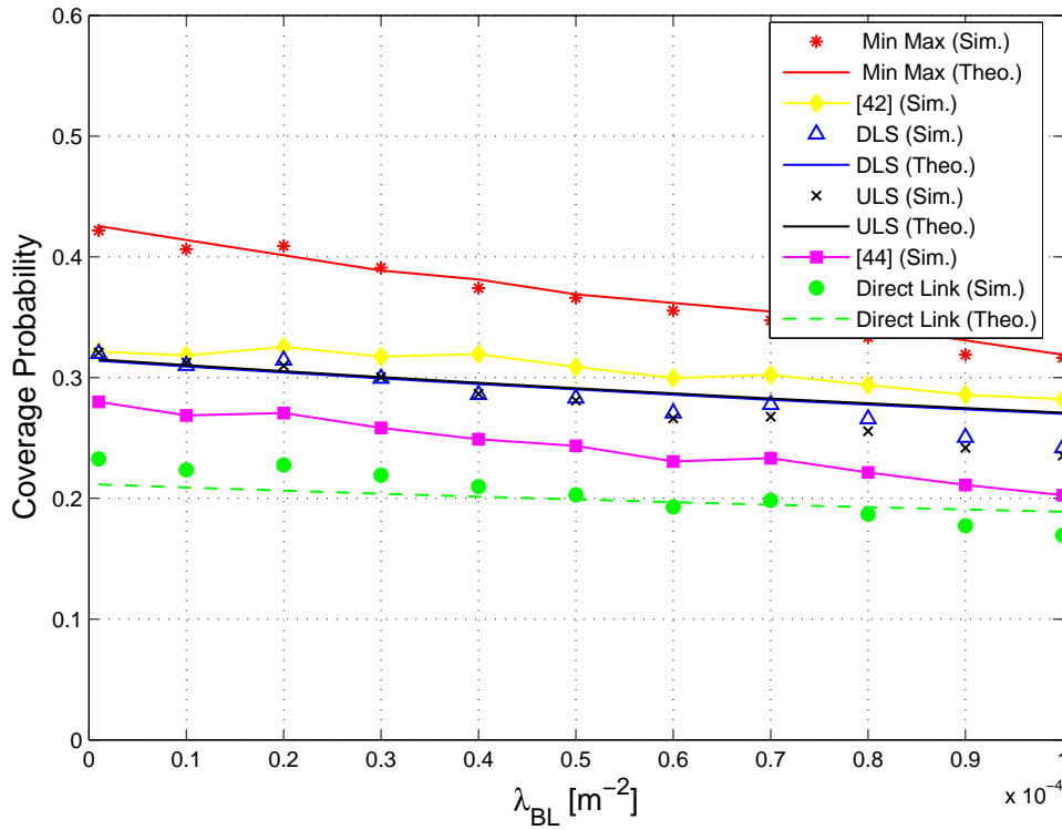
Figure 6.4: successful transmission probability of different schemes vs. \lambda_{BL} for N_{RL} = 15 .
