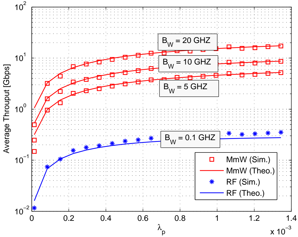
Figure 3.5: Average throughput vs. the total density of cells \lambda_p for different values of B_w , and \eta = 0.1 .
