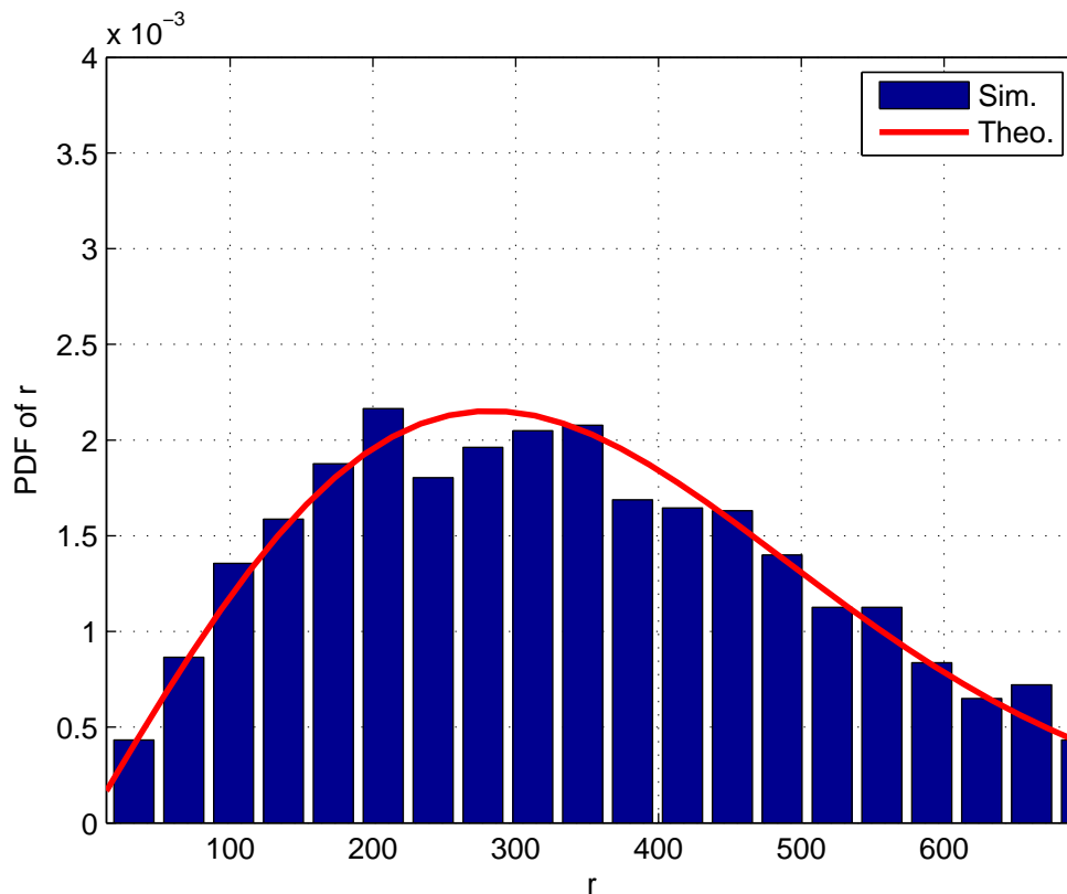
Figure 2.9: Histogram for simulating the PDF of the distance to the strongest BS as compared to the PDF expression of the distance to nearest one
