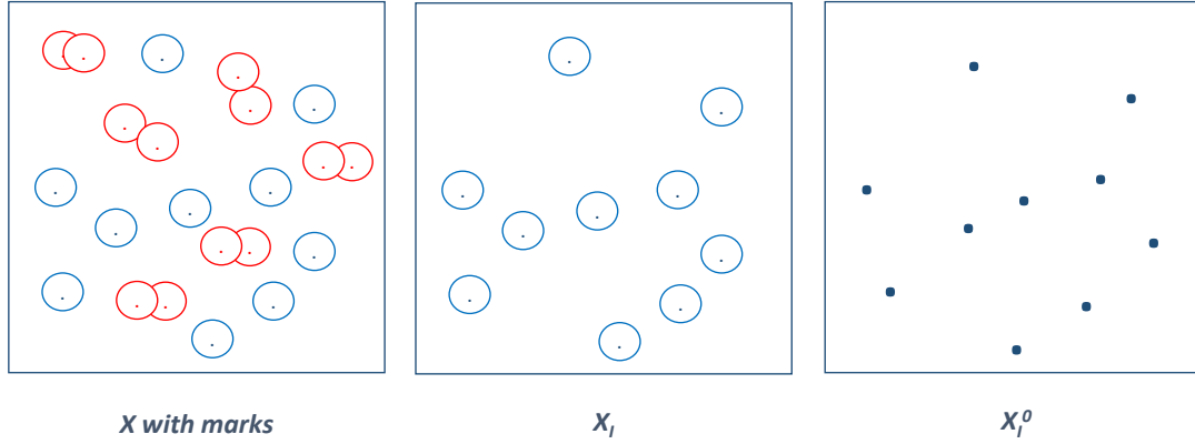
Figure 2.1: MHCP of type I
