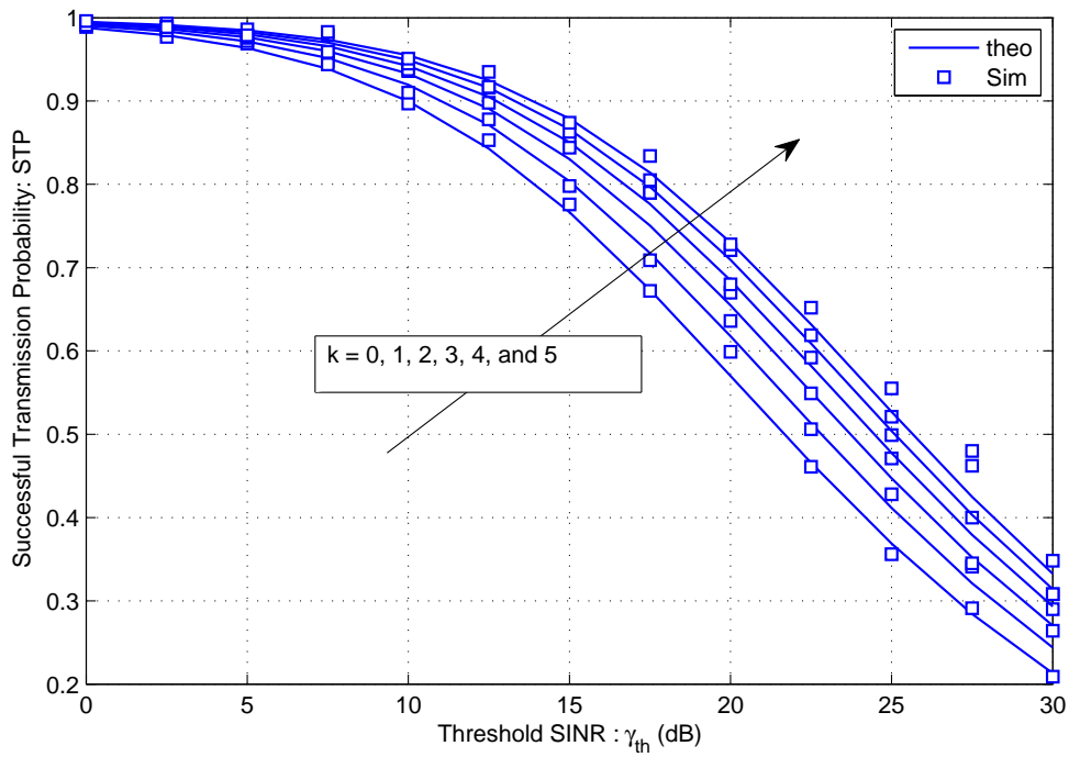
Figure 5.1: Average successful transmission probability vs. \gamma_{th} with different values of time slots k .
