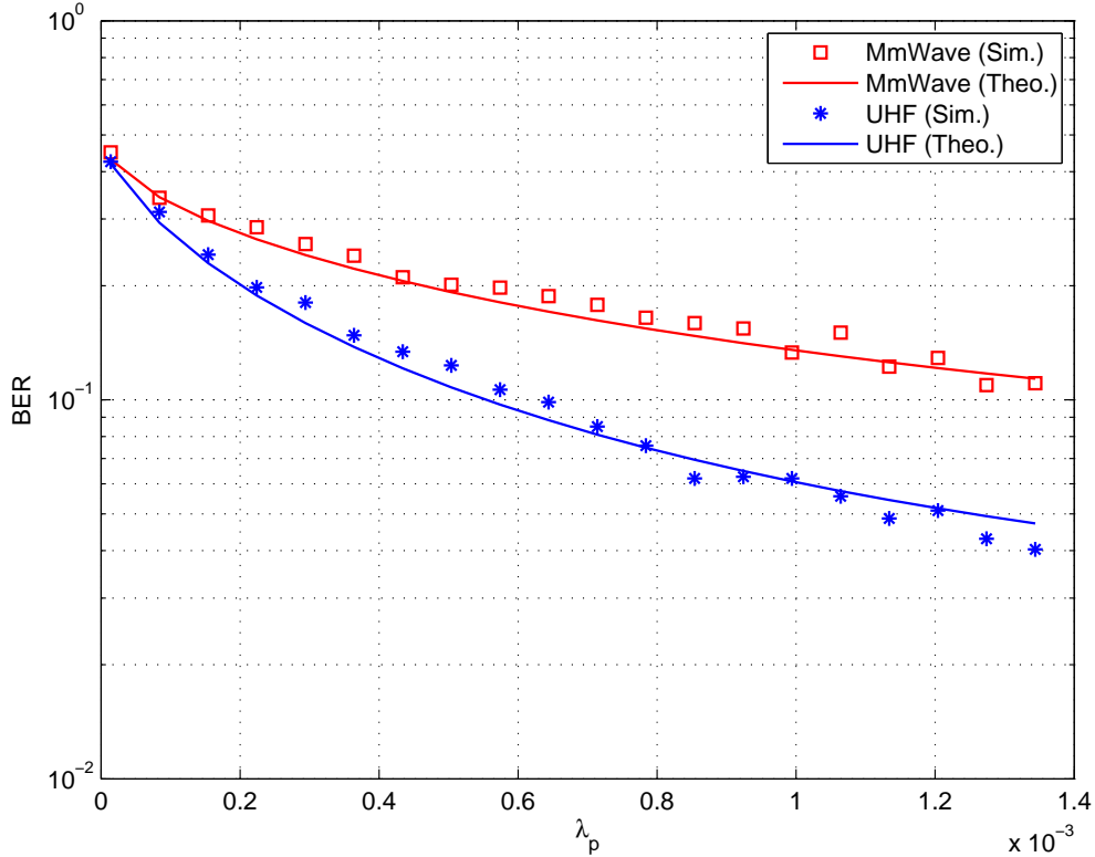
Figure 3.6: Average BER vs. \lambda_p with \eta = 0.1 .
