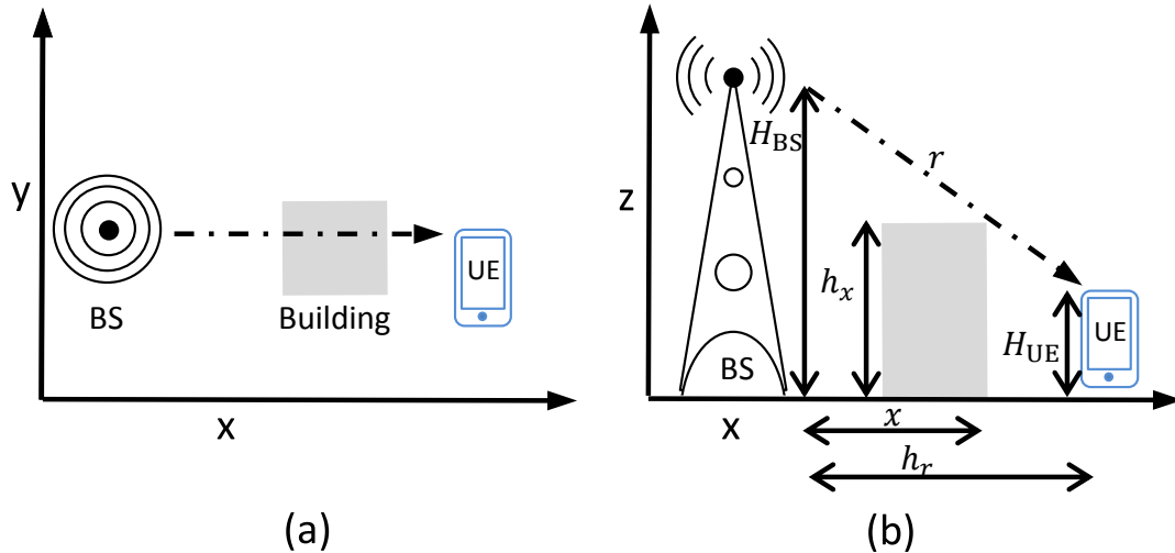
Figure 4.2: LOS: a) X-Y modeling, and b) X-Z modeling
