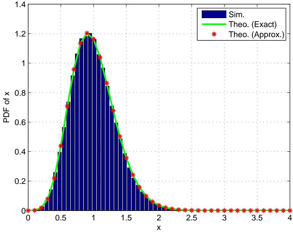
Figure 4.5: Empirical PDF of the Rice channel gain squared amplitude as compared to the exact and approximate expressions in (4.12) and (4.13), respectively, with K_{\text{Rice}} [dB] = 12 dB.
