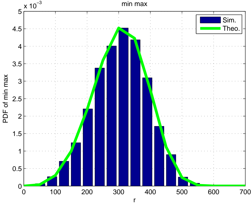
Figure 6.1: Theoretical and simulated PDFs of the corresponding distance within the proposed min/max scheme
