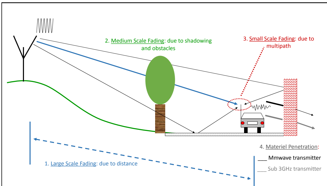
Figure 2.3: The wireless channel response components [70].
