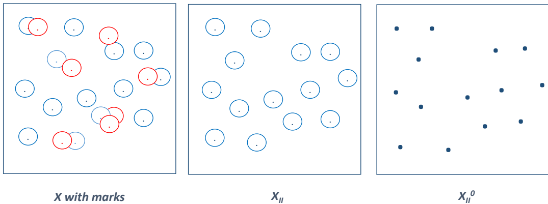
Figure 2.2: MHCP of type II
