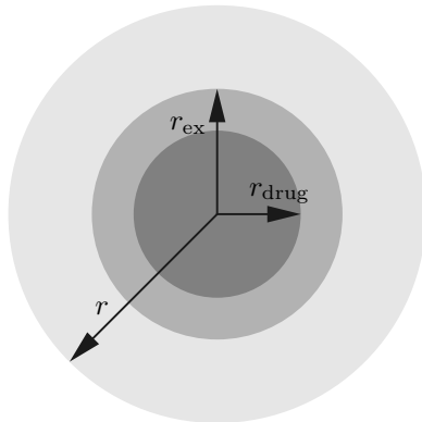
Figure 3.2 – Equivalent radii in a droplet
