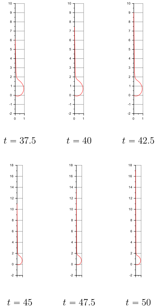
Figure 4.2 – Droplet evolution
