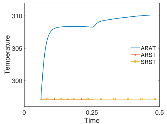
Figure 3.10 – Radius and temperature evolution of a particular droplet which deposits, comparison in the three models.
