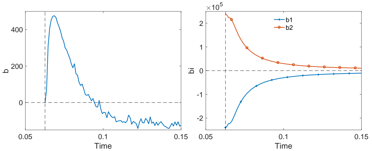
Figure 3.11 – Order of magnitude of each thermal effect b_1 and b_2 for a given particle.
