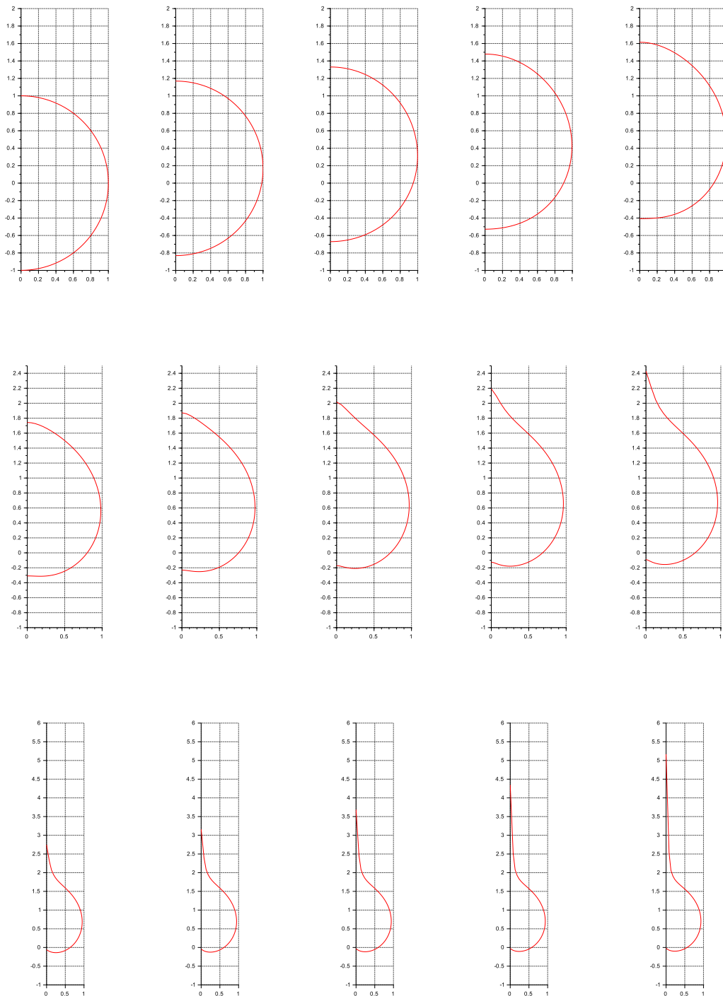
Figure 4.1 – Droplet evolution for t = 0, 2.5, \dots, 35
