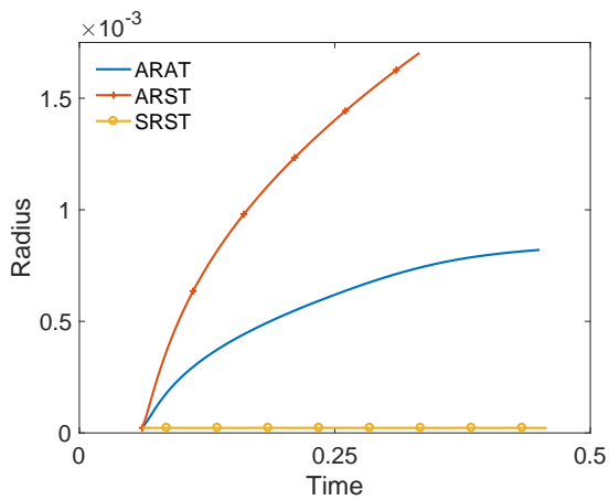
Figure 3.9 – Radius and temperature evolution of a particular droplet which goes out through the right branch, comparison in the three models.
