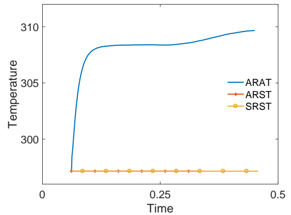
Figure 3.9 – Radius and temperature evolution of a particular droplet which goes out through the right branch, comparison in the three models.
