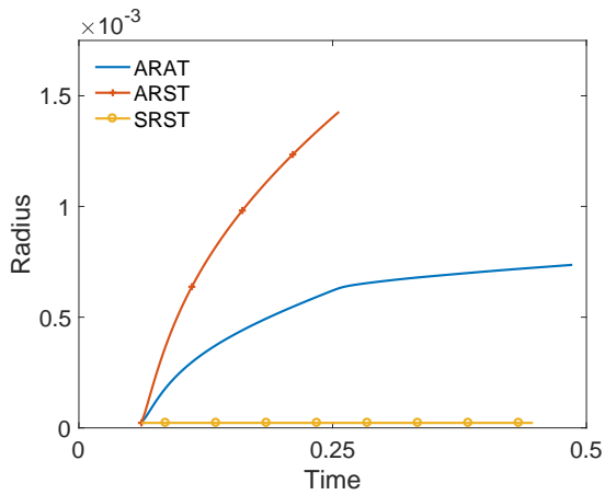
Figure 3.8 – Radius and temperature evolution of a particular droplet which goes out through the left branch, comparison in the three models.
