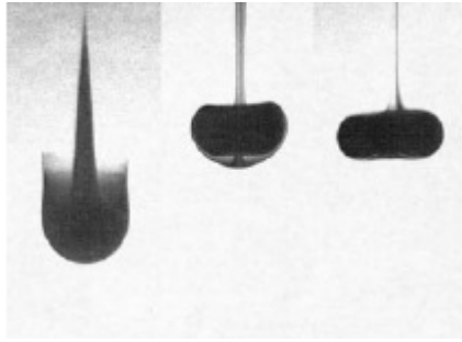
Figure 1 – Torus formation [55, Figure 2]
