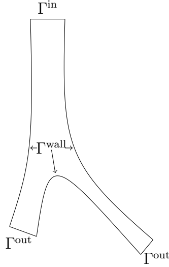
Figure 3.1 – Domain \Omega
