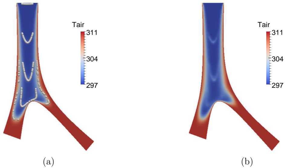
Figure 3.5 – Local effects of the aerosol on the air temperature, here at time 0.25 + \Delta t (in seconds).
