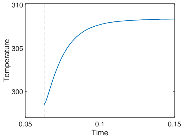
Figure 3.12 – Temperature evolution of the chosen particle in Figure 3.11.
