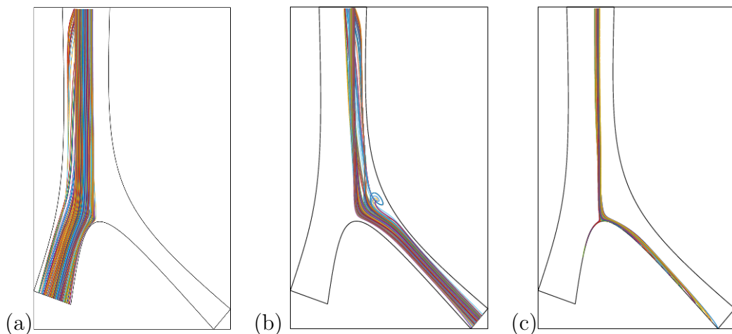
Figure 3.6 – Particle trajectories (a) towards the left branch, (b) towards the right branch, (c) deposition.
