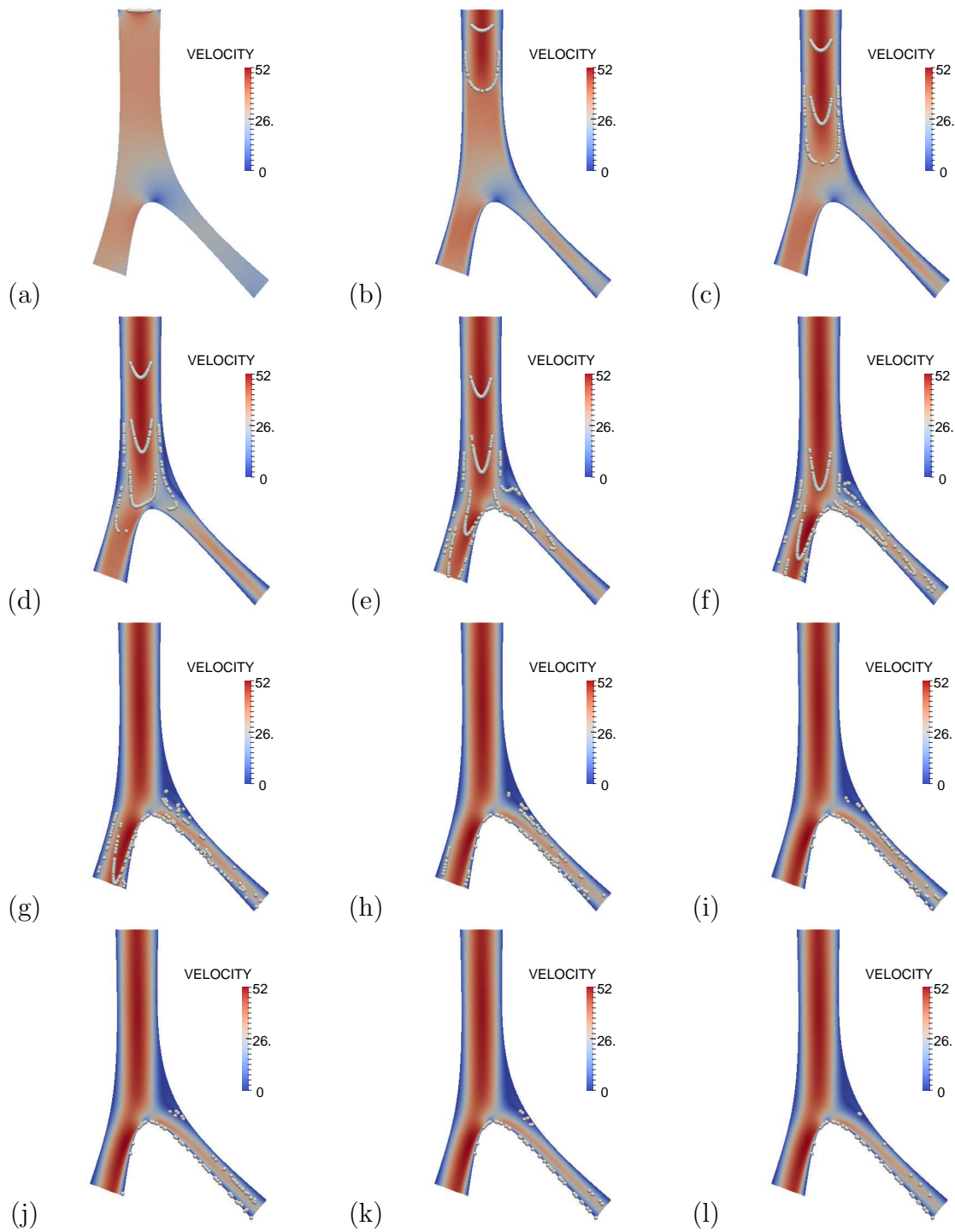
Figure 3.3 – Dynamics of the particles with the air velocity, at time t = 0.00, 0.08, 0.16, \dots, 0.80 s and at final time \tau = 1 s.
