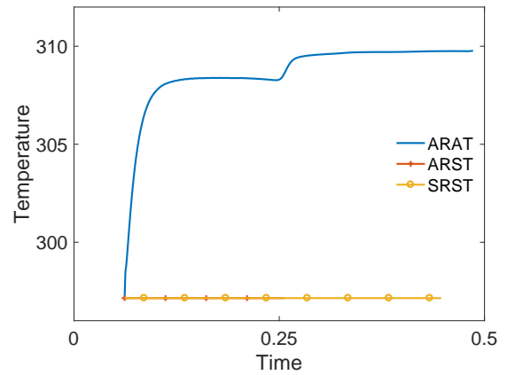
Figure 3.8 – Radius and temperature evolution of a particular droplet which goes out through the left branch, comparison in the three models.
