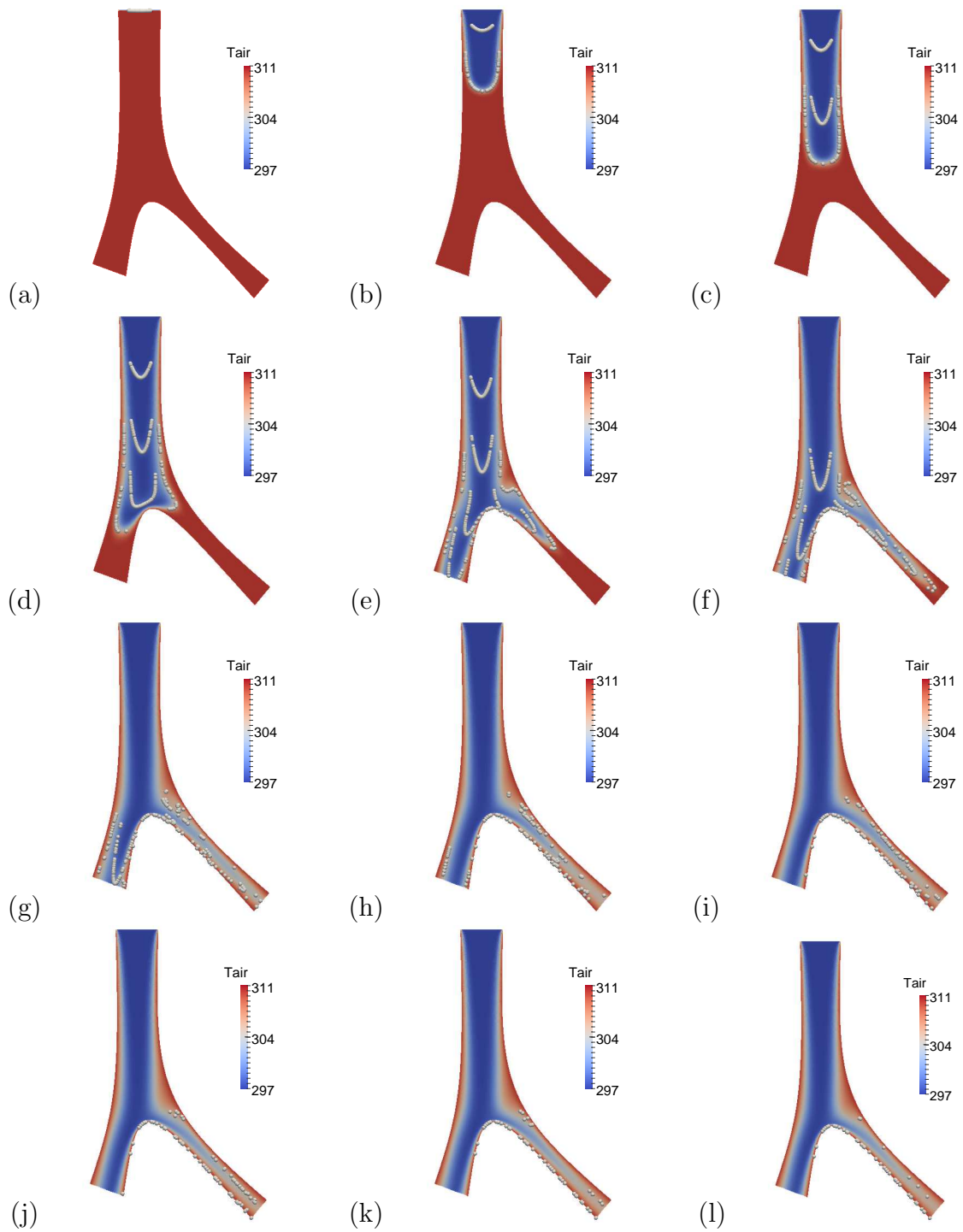
Figure 3.4 – Dynamics of the particles with the air temperature, at time t = 0.00, 0.08, 0.16, \dots, 0.80 s and at final time \tau = 1 s.
