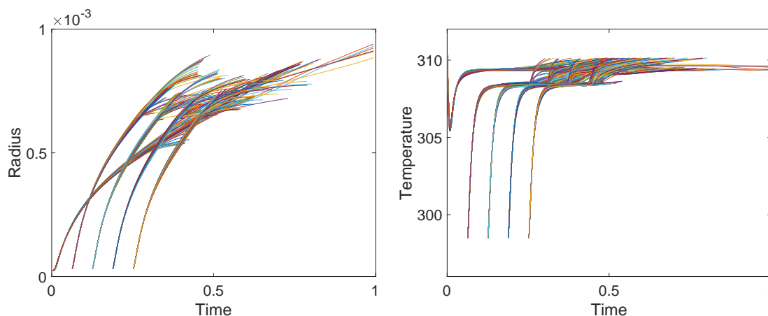
Figure 3.7 – Radius and temperature evolution of all the particles with respect to time.
