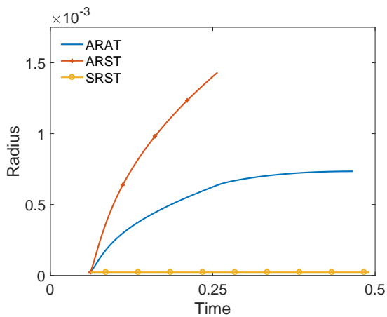
Figure 3.10 – Radius and temperature evolution of a particular droplet which deposits, comparison in the three models.
