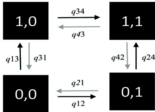
Figure 3. Diagram of the four transitional states of the correlated evolution between two traits \{x, y\} . A given ecological trait and susceptibility to acquire Mycobacterium ulcerans ( y ) hereafter called MU. Transition rate parameters ( q ) describe the transitions between states of correlated evolution ( \{0,0\} , \{0,1\} , \{1,0\} , \{1,1\} ). While considering back (grey arrows) and forward transitions (black arrows) of the correlated evolution, we examined evidence that the ecological trait evolved faster than host susceptibility to acquire MU ( q_{13} > q_{12} ), and susceptibility to acquire MU was facilitated by the ecological trait ( q_{34} > q_{24} ).
