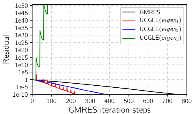
(d) Spectral Distribution VIII: matrix size = 2000, m_g = 20 , d = 10 , lsa = 10 , freq = 1 .
