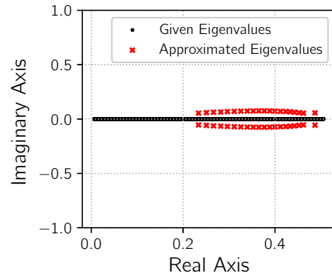
(a) Spectral Distribution V: matrix size = 2000, m_g = 10 , d = 10 , lsa = 10 , freq = 1 .
