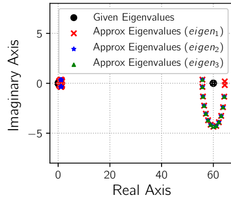
(c) Spectral Distribution VII: matrix size = 2000, m_g = 20 , d = 10 , lsa = 10 , freq = 1 .
