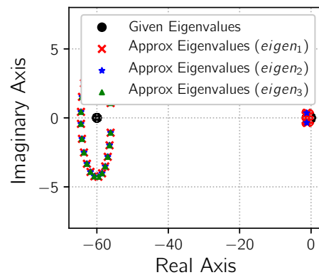
(d) Spectral Distribution VIII: matrix size = 2000, m_g = 20 , d = 10 , lsa = 10 , freq = 1 .
