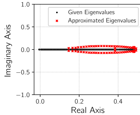
(b) Spectral Distribution VI: matrix size = 2000, m_g = 50 , lsa = 10 , freq = 1 .
