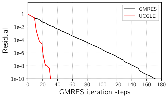
(a) Spectral Distribution V: matrix size = 2000, m_g = 10 , d = 10 , lsa = 10 , freq = 1 .
