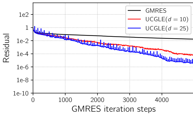
(b) Spectral Distribution VI: matrix size = 2000, m_g = 50 , lsa = 10 , freq = 1 .
