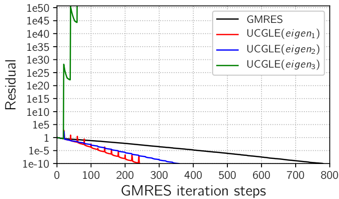
(c) Spectral Distribution VII: matrix size = 2000, m_g = 20 , d = 10 , lsa = 10 , freq = 1 .
