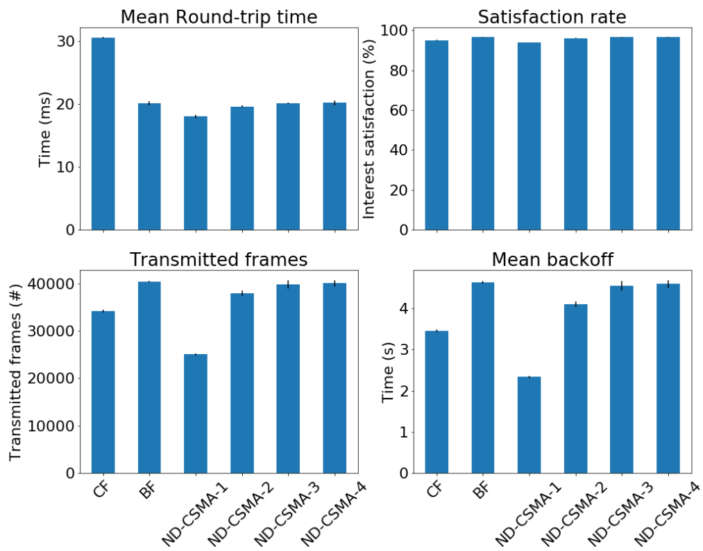
Figure 5.25: ND-CSMA evaluation
