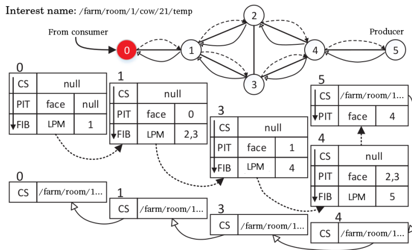
Figure 2.4: NDN communication process illustration
