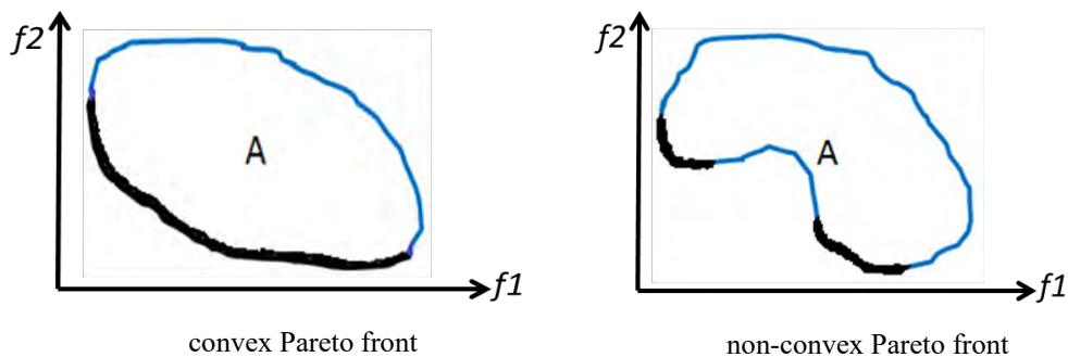
Figure 2.2 Pareto front for a bi-objective problem
