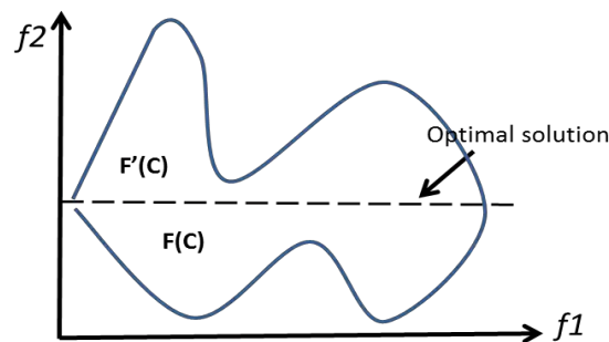
Figure 2.4 \epsilon -constraint method
