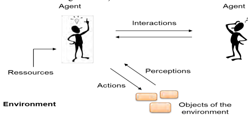
Figure 2.12 Multi-agent System
