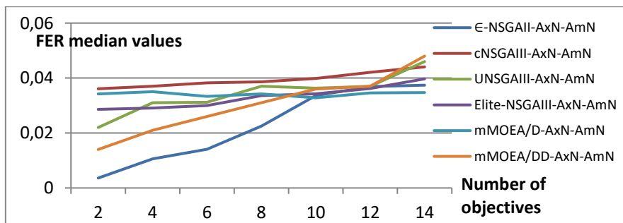
Figure 4.15 Average FER rates for different number of objectives
