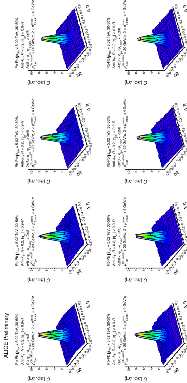
Figure 77: Near-side jet-hadron correlation functions w.r.t VOC event plane for p_{T,trigger} > 20 GeV/c, 2 < p_{T,assoc}^{assoc} < 4 GeV/c.
