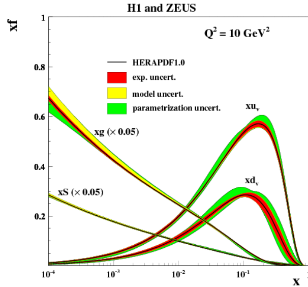
Figure 4: The Parton Distribution Functions from HERAPDF1.0 at Q^2 = 10 \text{ GeV}^2 [3].
