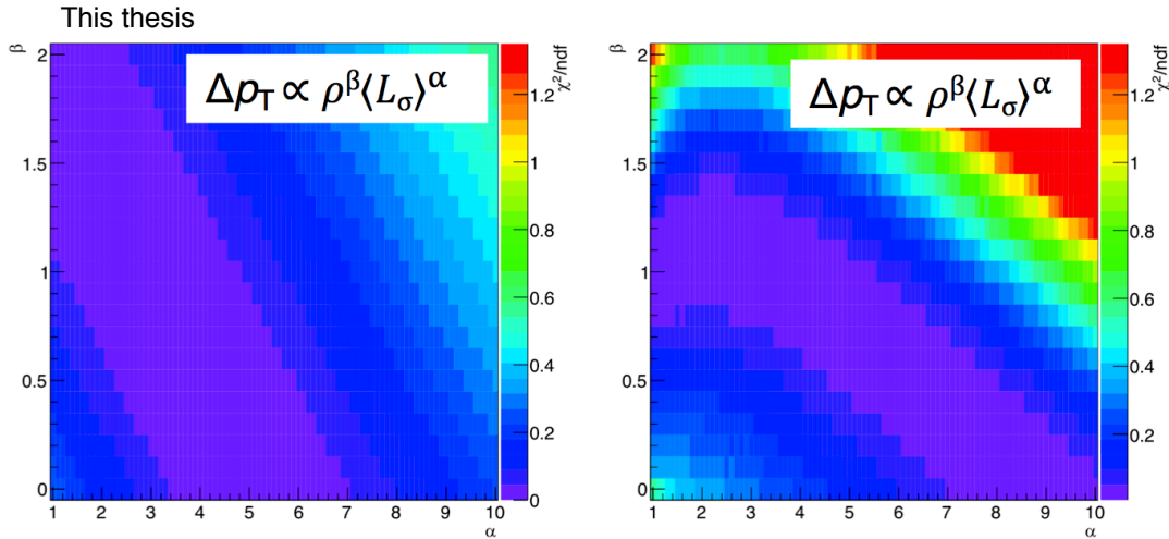
Figure 112: The reduced chi-square as a function of the exponent of \langle L_\sigma \rangle ( \alpha ) and of \rho ( \beta ) for \Delta p_T (derived from R=0.2 jet R_{AA} ) fit (left) and for jet v_2 (right).
