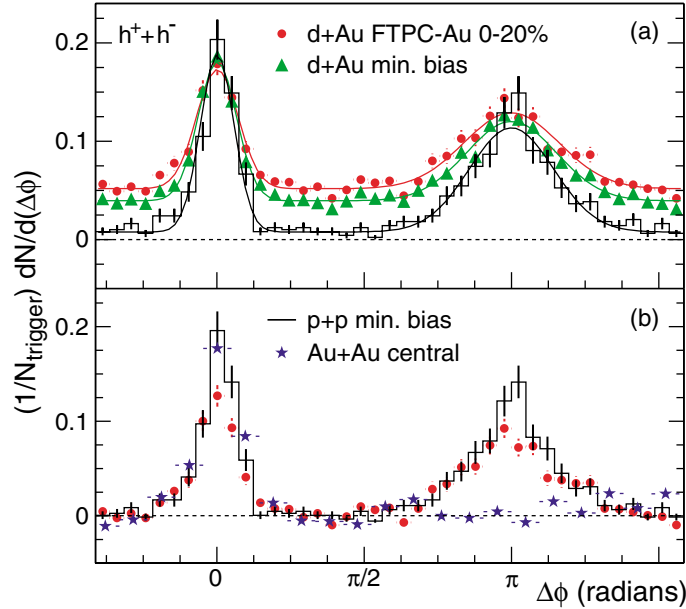
Figure 17: Two-particle correlations in pp, d+Au and Au+Au collisions at \sqrt{s_{NN}} = 200\text{GeV} for 4 < p_T^{trig} < 6\text{ GeV} and 2 < p_T^{assoc} < p_T^{trig} [12].
