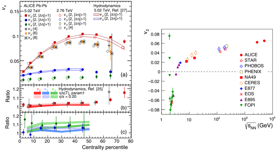
Figure 25: The experimental results of anisotropic flow coefficients ( v_n ) [19] Left: (a) Anisotropic flow coefficients v_n integrated over 0.2 < p_T < 5.0 GeV/ c , as a function of event centrality for the two-particle and multi-particle cumulant methods. (b),(c) are the ratios to the various hydrodynamic calculations. "Ref. [25]" and "Ref. [27]" in the figure correspond to Ref. [20],[21] respectively in the bibliography. Right: Comparison of the integrated elliptic flow results from various experiments at various collision center-of-mass energies.
