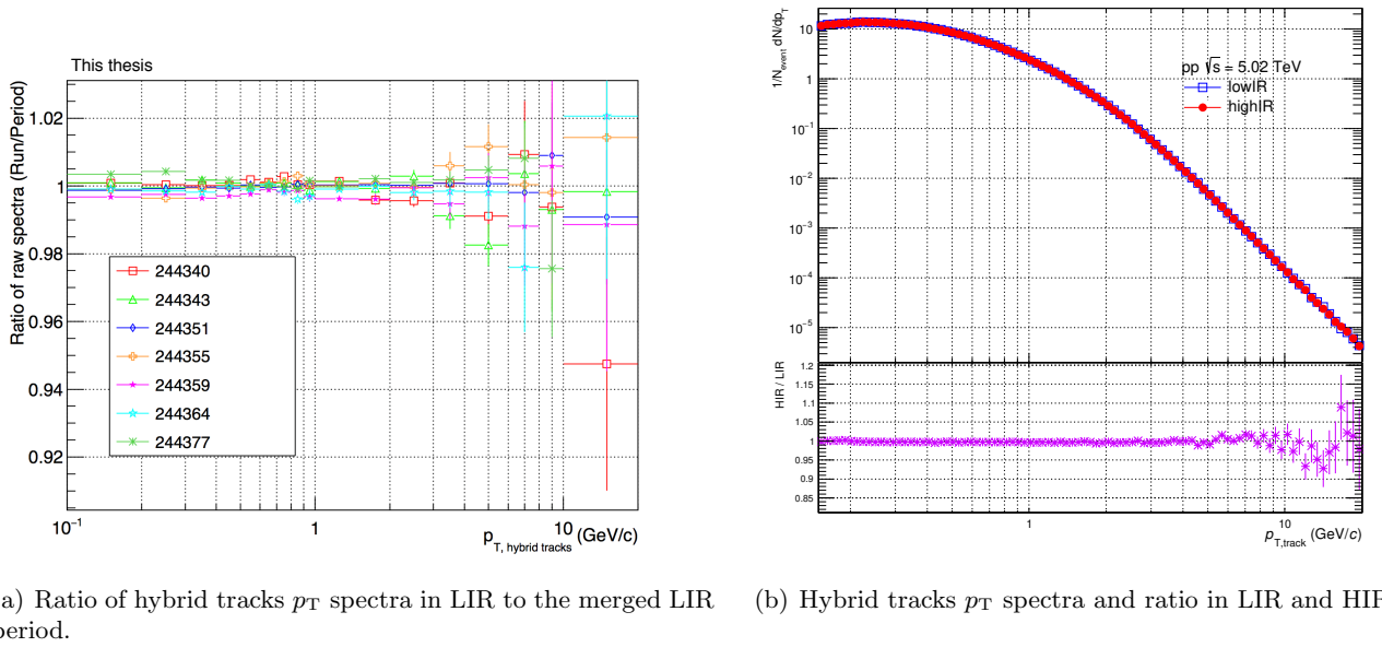
Figure 119: Validation of hybrid tracks p_T spectra per data collection period.
