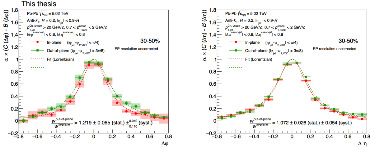
Figure 113: Near-side jet-hadron correlations for in-plane jets ( |\Delta\phi(\phi_{\text{jet}}-\psi_2)| < \pi/4 , Red) and out-of-plane jets ( |\Delta\phi(\phi_{\text{jet}}-\psi_2)| > 3\pi/8 , Green). p_{T,\text{jet}}^{\text{ch,det}} > 20 \text{ GeV}/c . 0.7 < p_{T,\text{track}}^{\text{assoc}} < 2 \text{ GeV}/c . \alpha is selected so that the fit function height is 1.
