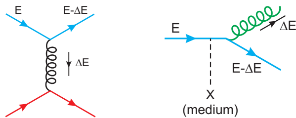
Figure 13: Left: Feynman diagram of collisional parton energy loss. Right: Feynman diagram of radiative parton energy loss. [2]
