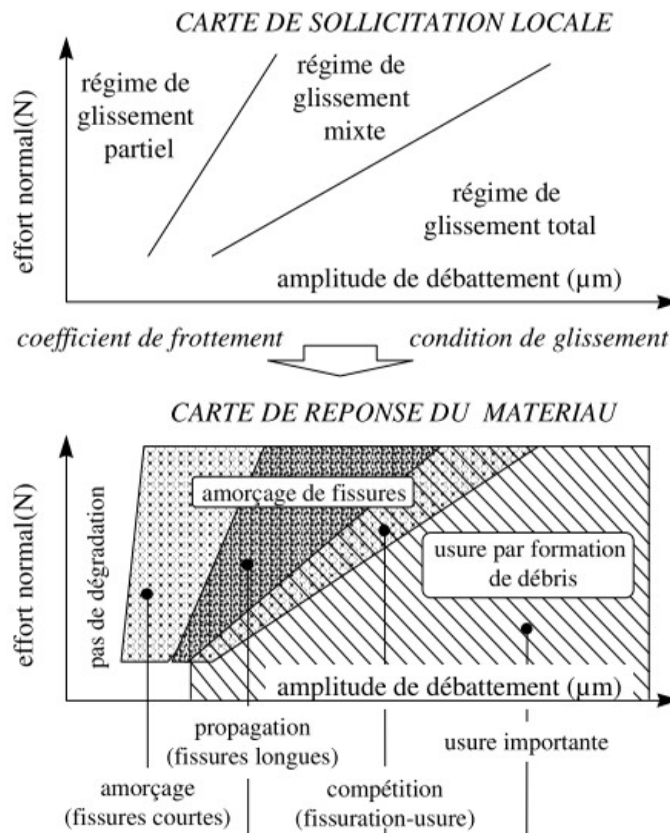
FIGURE 1.8 – Illustration des cartes de fretting [11]
