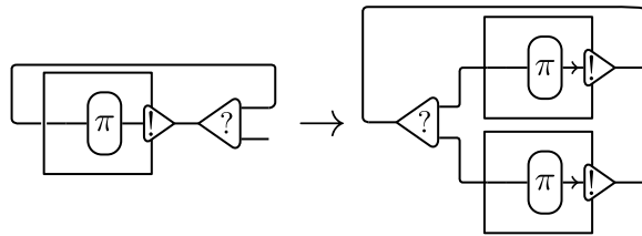
Figure 2.3: Self replicating pattern using a box
