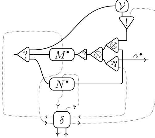
Figure 5.7: Translation of M N
