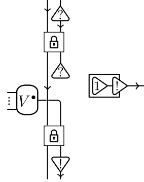
Figure 5.10: Encoding of \text{set}(r, V)
