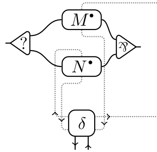
Figure 5.8: Translation of parallel
