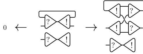
Figure 2.4: Counter example for (T_1)
