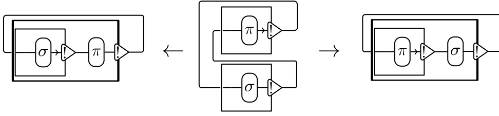
Figure 2.1: Example of non-confluence
