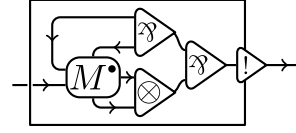
Figure 5.6: Translation of \lambda x.M
