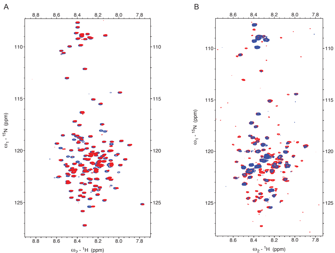
Figure 4.13. Superposition of the ^1\text{H} - ^{15}\text{N} HSQC spectrum of isolated Ntail alone (in blue) and the mixture of labelled Ntail and unlabelled N-rings (in red) (A), of labelled N-rings alone (in blue) and with Ntail (in red) (B).
