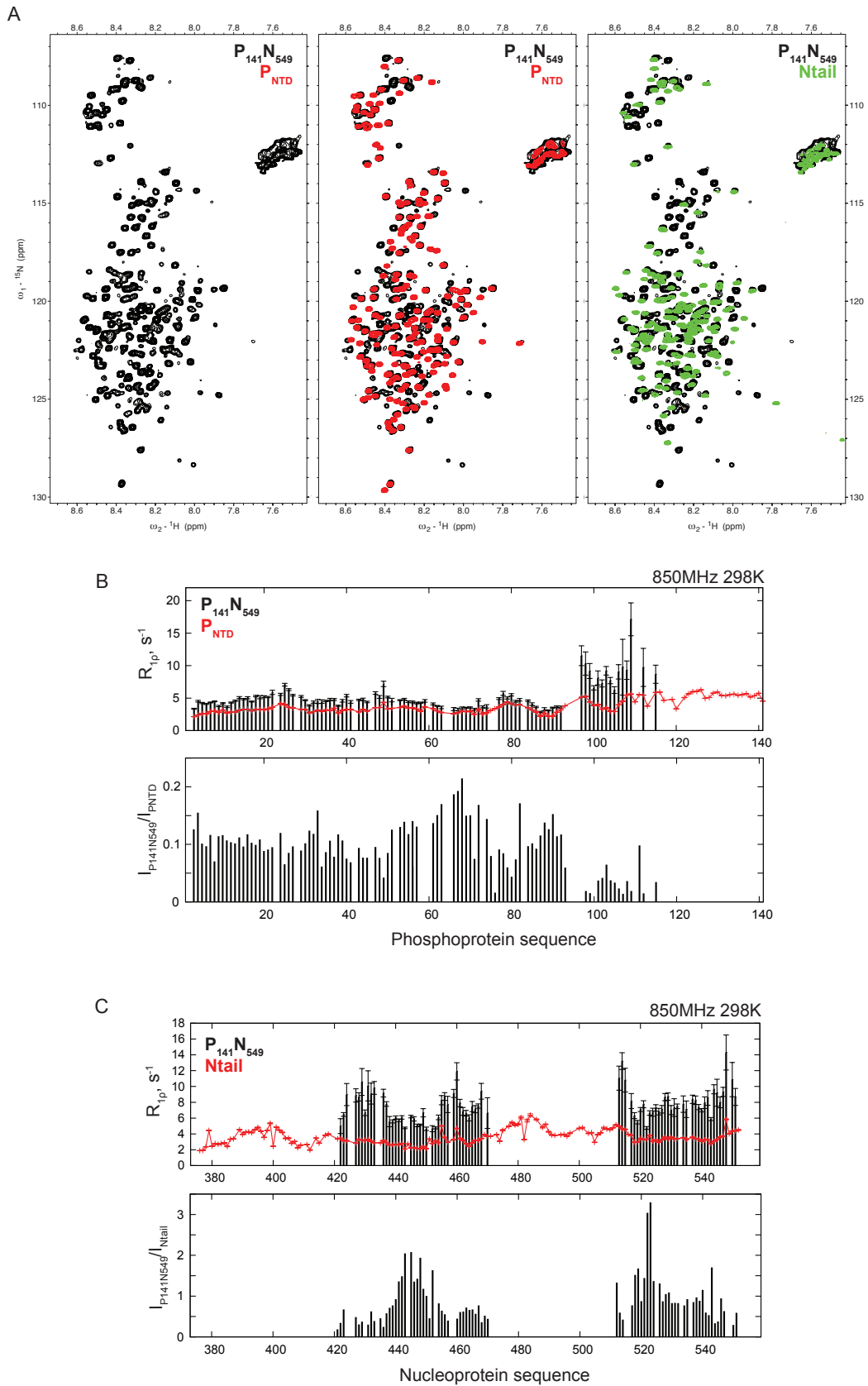
Figure 6.2. Spectrum of P_{141}N_{549} alone (in black) and overlaid with P_{NTD} (in red) and Ntail (in green) (A). Intensity ratio calculated from P_{NTD} or Ntail over P_{141}N_{549} and R_{1p} profile of N^{\circ}P compared to Ntail and P_{NTD} measured at the same temperature and magnetic field (B, C).
