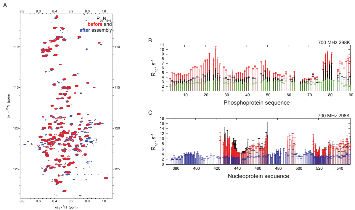
Figure 6.10. 2D ^1\text{H} - ^{15}\text{N} HSQC spectrum of \text{P}_{90}\text{N}_{549} before (in red) and after (in blue) assembly with PolyA6 RNA, arrows indicate peaks that also appeared during the addition of \text{P}_{\text{NTD}} to \text{P}_{65}\text{N}_{549} (A). Numbers indicate the disappeared (2, 3, 4) and appeared (1) residues. The R_{1p} profile of N o P P (B) and N (C) before (in red) and after (in black) addition of RNA compared to \text{P}_{\text{NTD}} (in green) and N alone (in blue) measured at the same magnetic field.
