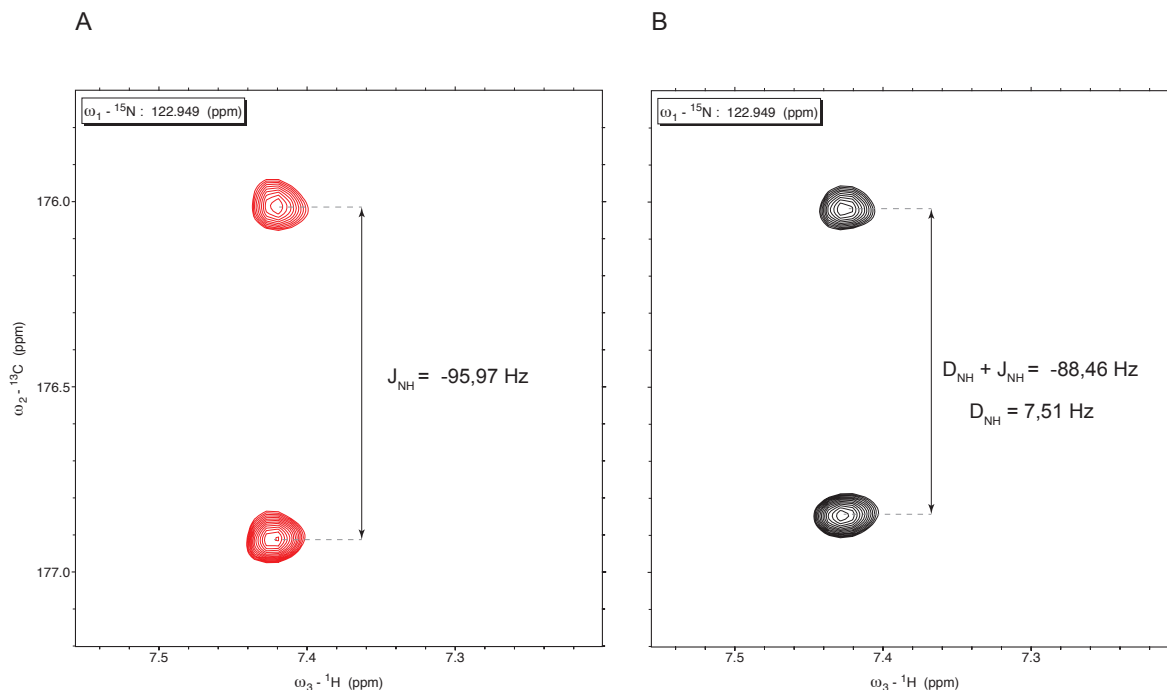
Figure 2.17. The extraction of RDC from ^1J_{\text{NH}} of MuV P CTD . ^{15}\text{N} slices of two 3D spectra are compared, in absence (A) and presence (B) of anisotropic medium with further calculation of dipolar coupling constant for particular protein residue (B).
