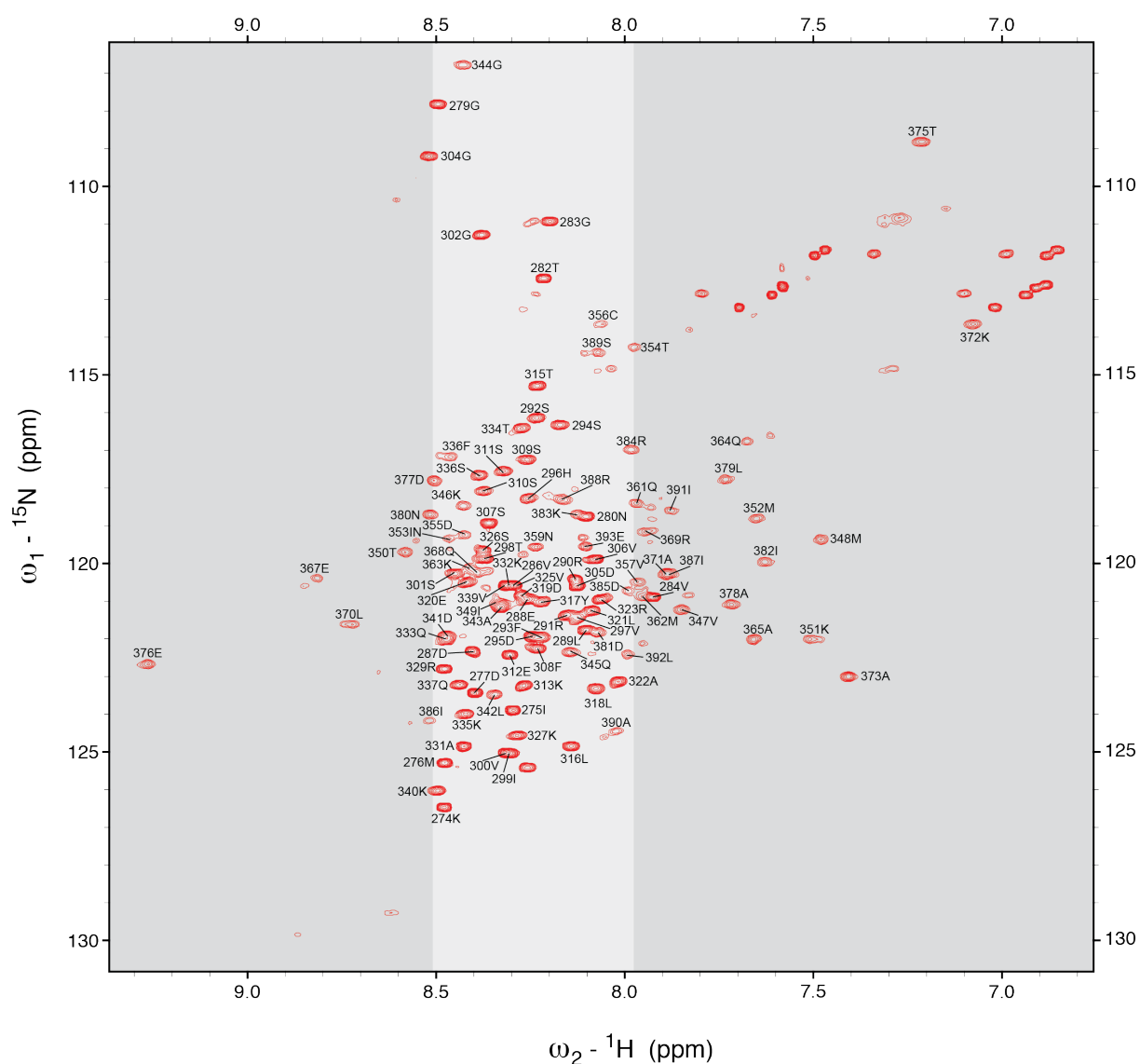
Figure 5.7. Protein residue spectral assignments of P CTD recorded at 25°C and 700 MHz in 50 mM Na-phosphates, 500 mM NaCl, 2 mM DTT pH 6. The cross-peak distribution in terms of
