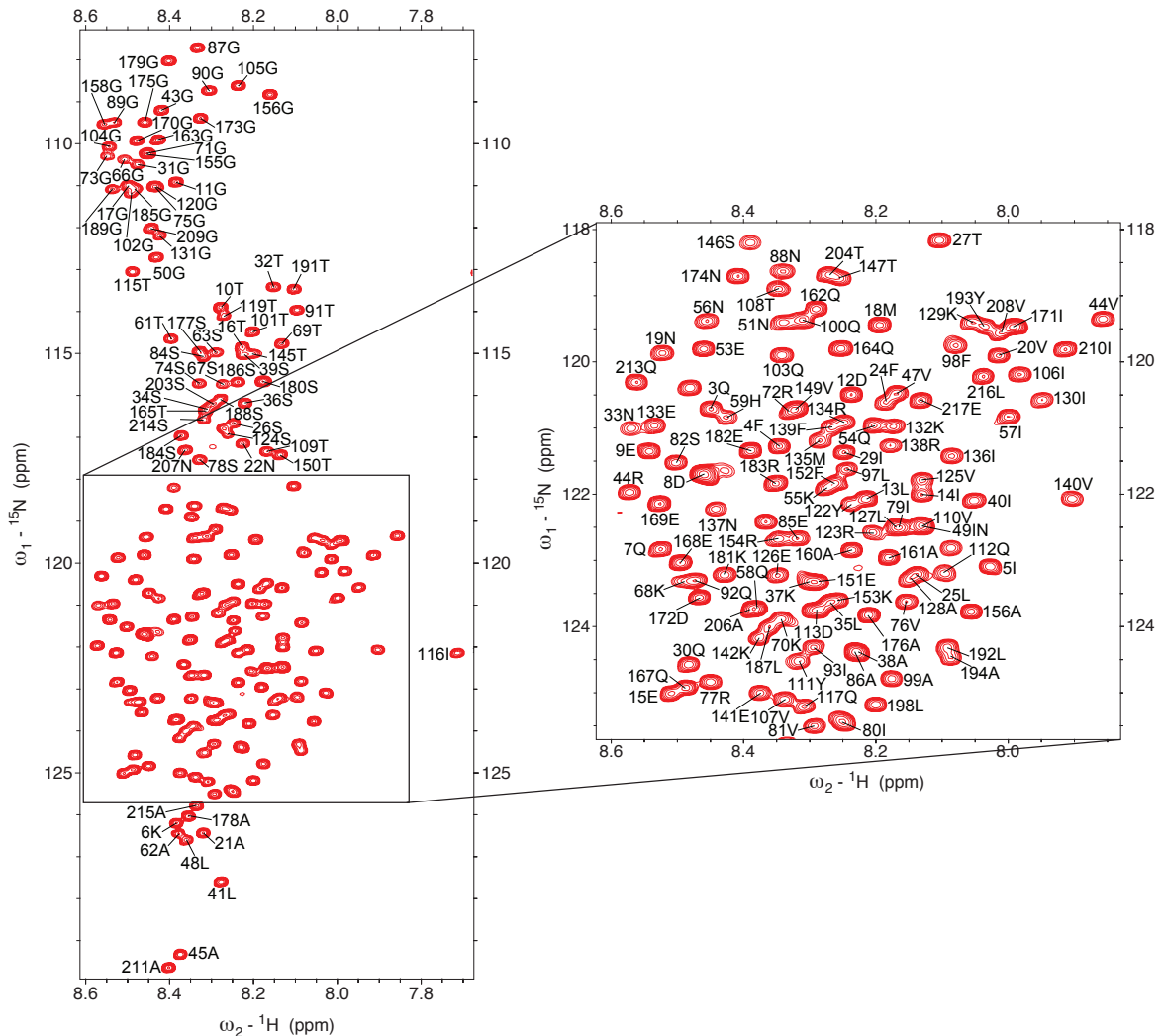
Figure 5.2. Residue specific assignment of P_{NTD} displayed on ^1\text{H} - ^{15}\text{N} HSQC spectrum at 25^\circ\text{C} and 850 MHz in 50 mM Na-phosphates, 500 mM NaCl, 2 mM DTT pH6. Peaks from glutamines, arginines and asparagines side chains are not shown.
