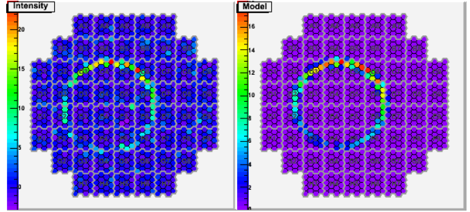
Figure 1.5: Comparison between muon rings observed by H.E.S.S. (left) and an analytical model (right). The figure is taken from Chalme-Calvet et al. (2014) .
