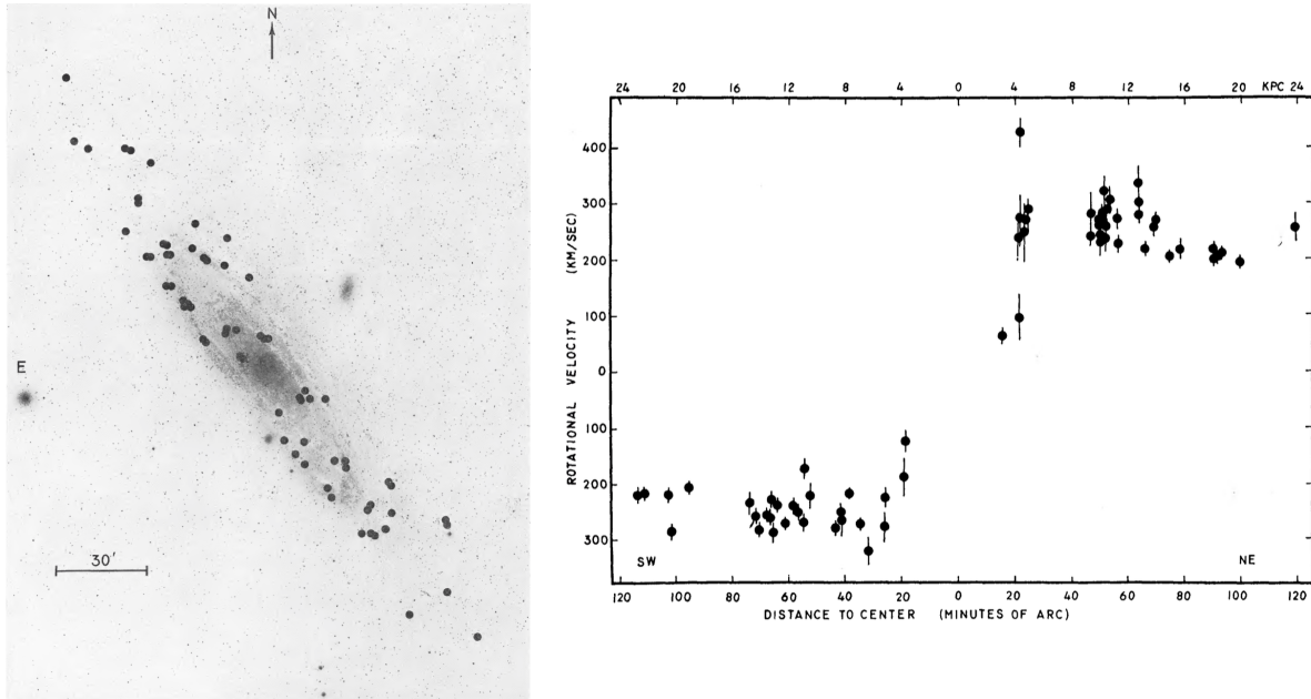
Figure 2.2: Photography of Andromeda galaxy (left) and its corresponding rotation curve (right). Each point on the galaxy photography corresponds to a measurement of rotation velocity at a given distance to the galaxy center on the rotation curve plot. Figures taken from Rubin & Ford (1970).
