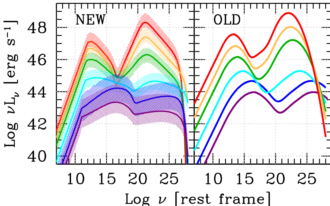
Figure 3.4: Revised (left) and initial (right) blazar sequences. The difference between the two sequences comes from the SEDs categorization in luminosity: the initial one uses radio luminosity while the revised one uses \gamma -ray luminosity. The equivalent energy range for the x-axis goes from 4.7 \cdot 10^{-8} eV to 470 TeV. Figure taken from Ghisellini et al. (2017) .
