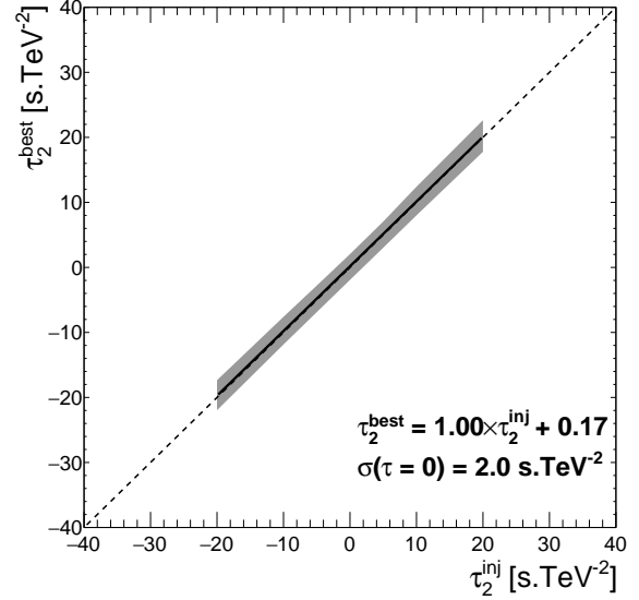
(b) Quadratic LIV effect (n=2).
