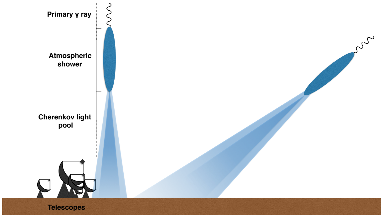
Figure 7.1: Illustration of the high zenith angle observation. The incoming \gamma ray with high ZA produce a larger and fainter Cherenkov light pool than the one with small ZA angle.
