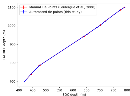
Figure 6. Comparison of the manual tie points between TALDICE and EDC derived by Loulergue et al. (2008) (red) and the same points recreated from the synchronization in this study (blue). The uncertainties estimated by eye (Loulergue et al., 2008) and by calculating the standard deviation of the ensemble of fits (this study) are shown as error bars.
