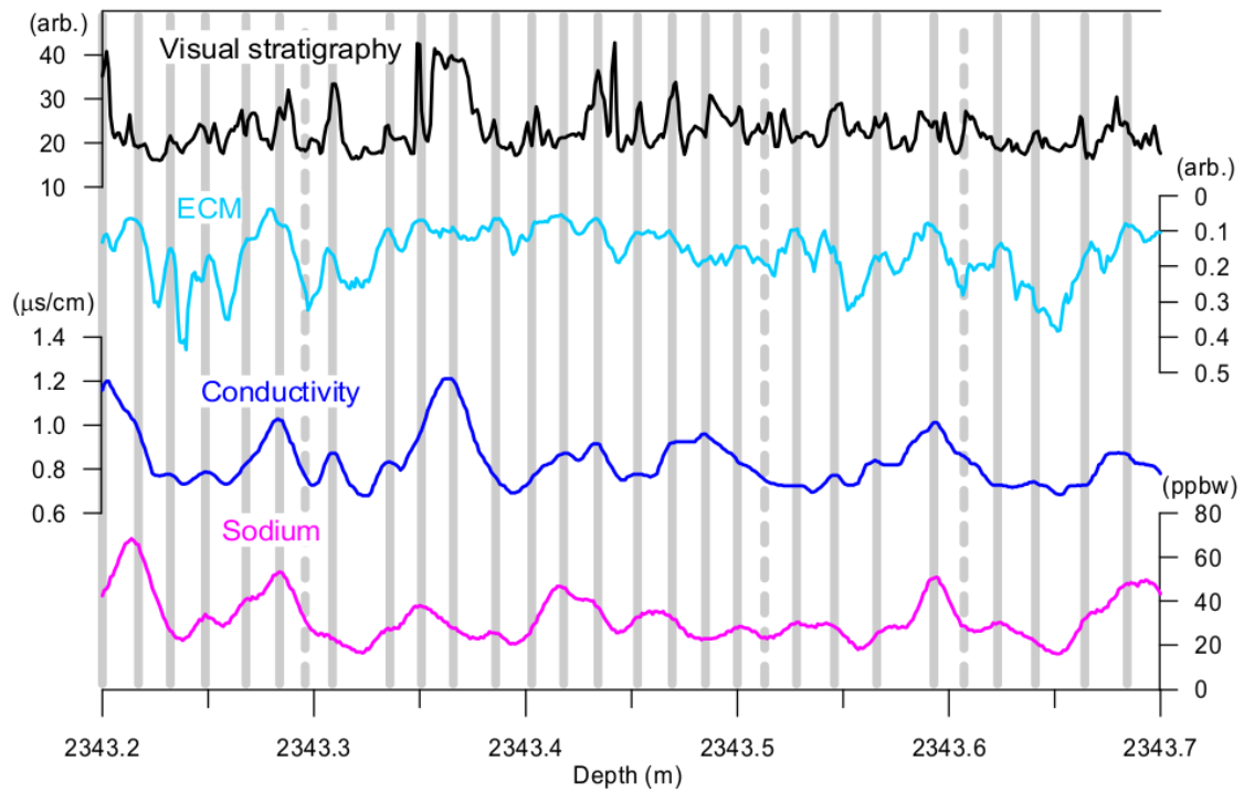
Figure 2: Example of annual layer counting from GICC05, within Greenland Interstadial 14 (54-49 kyr BP). The records are visual stratigraphy grey scale, ECM, conductivity, and \text{Na}^+ concentration. (Uncertain) Annual layers are indicated by (dashed) grey vertical bars. Units of the grey scale and the ECM profiles are arbitrary but comparable to those in Fig. 2. The counting of this section is mostly based on the conductivity and \text{Na}^+ profiles because the other records are known to have multiple peaks within an annual layer during milder climatic periods. Figure from Svensson et al. [2008].
