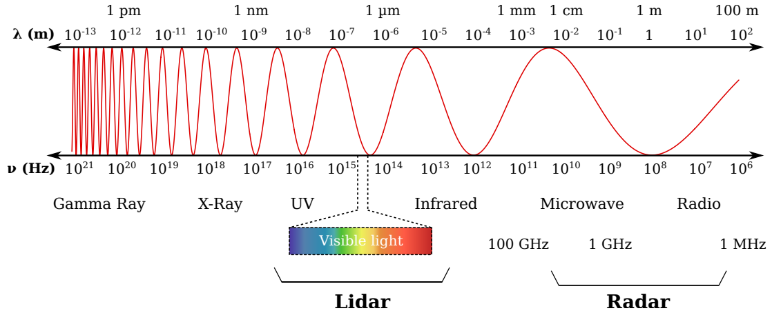
Figure 1.1: Electromagnetic spectrum.
