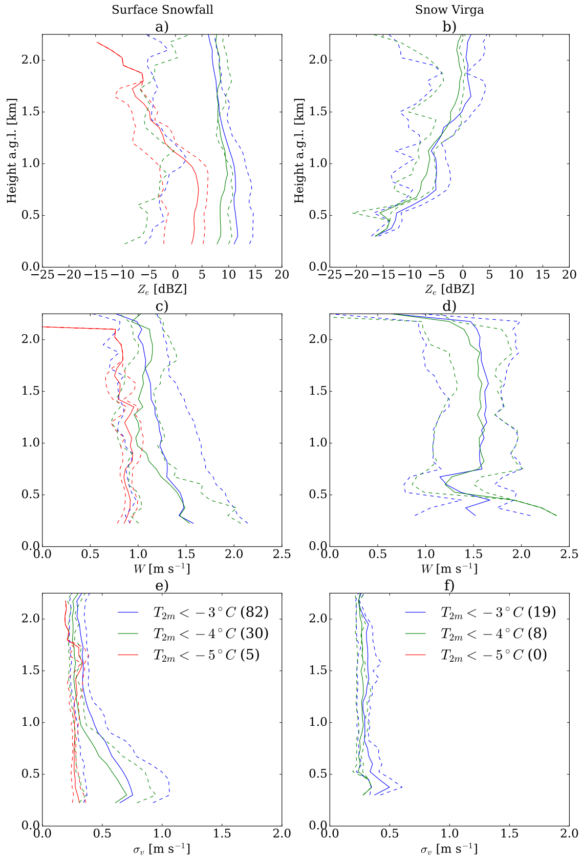
Figure E.1: Vertical profiles of Doppler moments using different thresholds on the temperature: <-3 , <-4 and <-5^\circ\text{C} . a and b correspond to Z_e , c and d to vertical velocity and e and f represent \sigma_v . In the legend, the number inside the parentheses indicates the total of snow or virga profiles for the given threshold.
