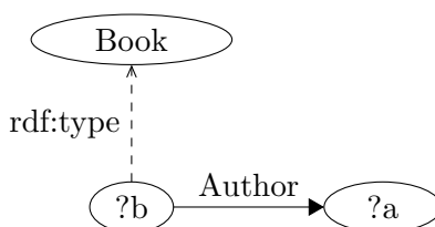
FIGURE 1.7 – Patron de graphe SPARQL
