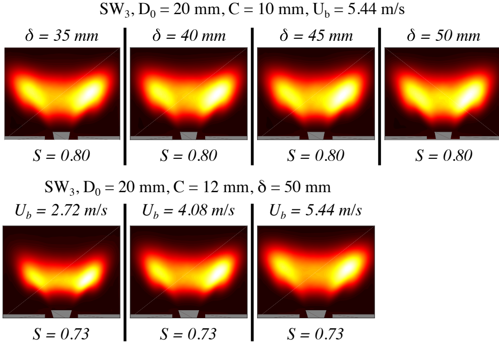
Figure 4.8: OH^* flame light distribution for different configurations tested. First line: effect of the distance \delta between swirler exit and combustor backplane. Second line: effect of the injection velocity U_b . The swirl number is fixed in each line. The colorscale is the same as the one used in Fig. 4.7.
