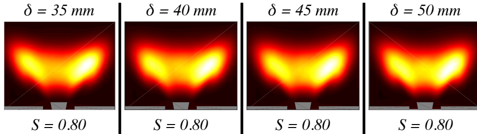
Figure 6.4: OH^* flame light distribution for the geometrical configuration featuring SW_3 , D_o = 20 mm, C = 10 mm, \delta = 35 - 50 mm. The bulk flow velocity is U_b = 5.44 m/s and the equivalence ratio is \phi = 0.82 . The colorscale is the same as the one used in Fig. 6.2.
