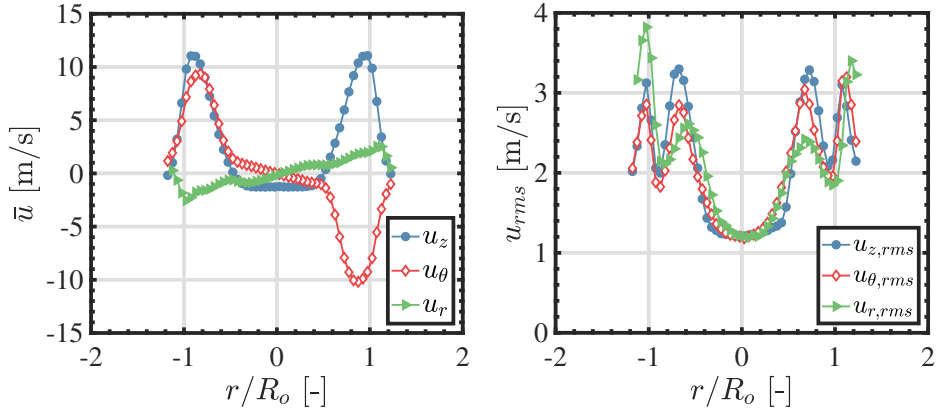
Figure 2.5: Mean \bar{u} and root mean square u_{rms} values of the axial, azimuthal and radial velocity components for steady operating conditions, measured by LDV at a distance of 1.5 mm from the top cone of the central rod. Measurements refer to a geometrical configuration with SW_3 , D_o = 20 mm and C = 10 mm and to a bulk flow velocity U_b = 5.44 m/s.
