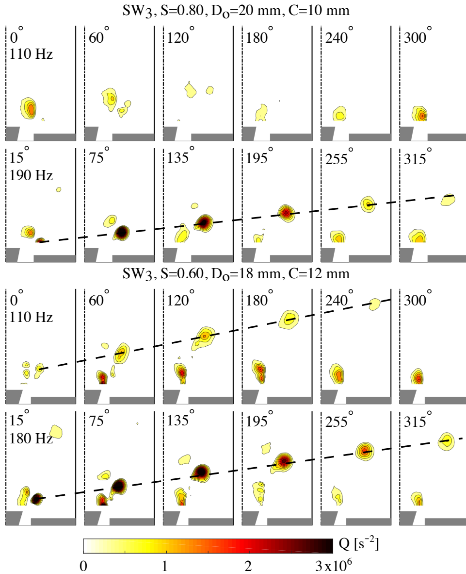
Figure 7.7: Q criterion contours deduced from PIV data in cold flow conditions for a forcing level u'/\bar{u} = 0.30 RMS. The same colorbar, set from 0 to 3 \cdot 10^6 s -2 , is applied to all figures. Only positive values of Q are retained. The indicated phase angle is referred to the signal measured by the hot wire HW.
