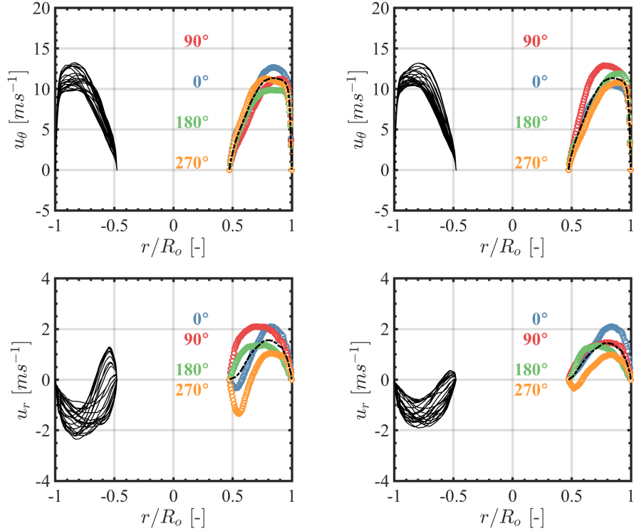
Figure 7.18: Azimuthal (top) and radial (bottom) velocity profiles at the burner outlet section AS_{56\text{mm}} ( D_o = 20 mm) at frequencies corresponding to a minimum ( f = 120 Hz, left) and to a maximum FTF gain value ( f = 190 Hz, right). The profiles at 24 phases in the cycle are shown for negatives r/R_o values. Four characteristic phases are shown for positives r/R_o values. The average profile is also superposed as a dashed-dotted line.
