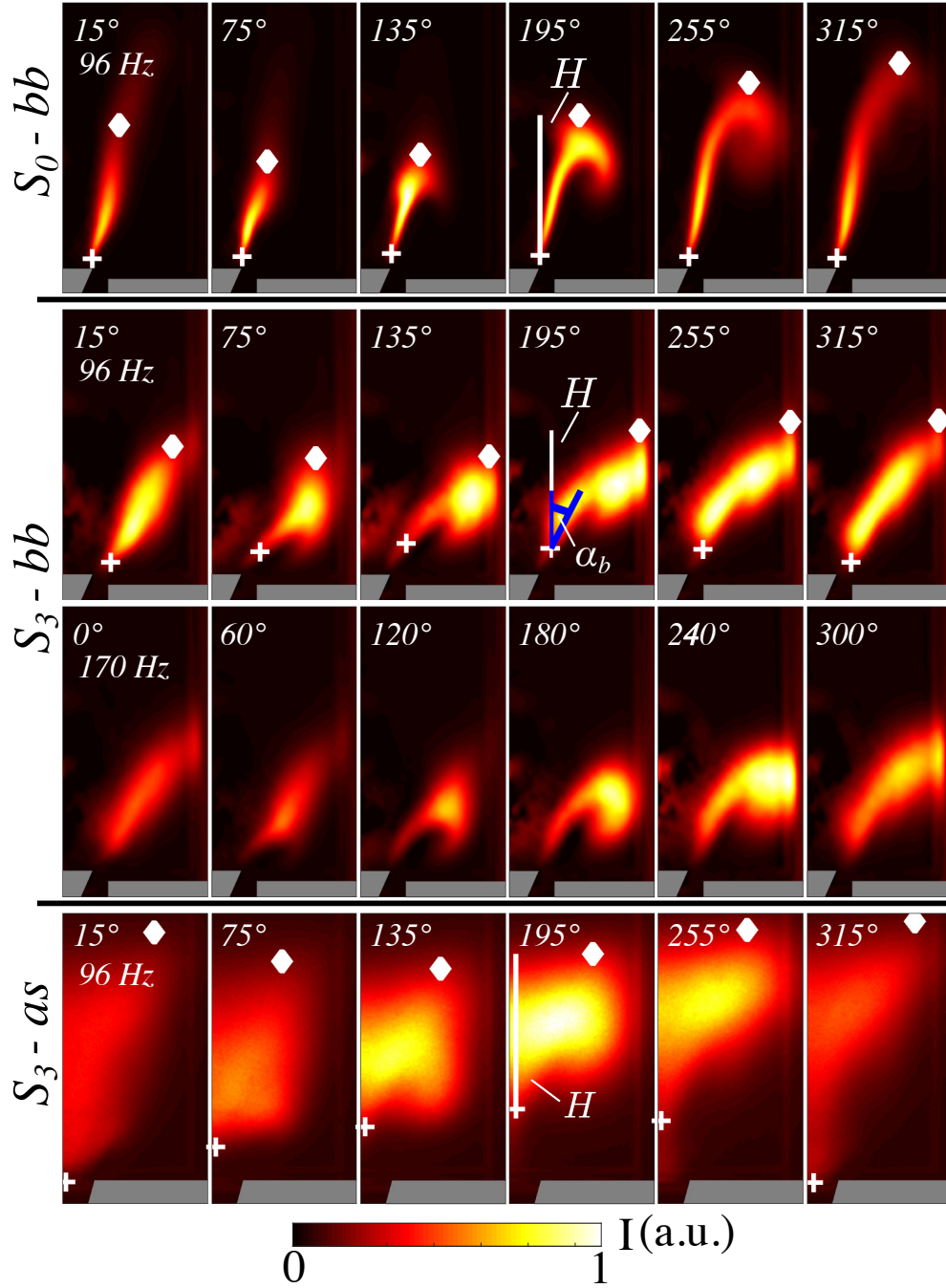
Figure 9.3: OH^* intensity phase averaged images at a forcing level u'/\bar{u} = 0.30 RMS. \dagger : flame root position. \diamond : flame tip position.
