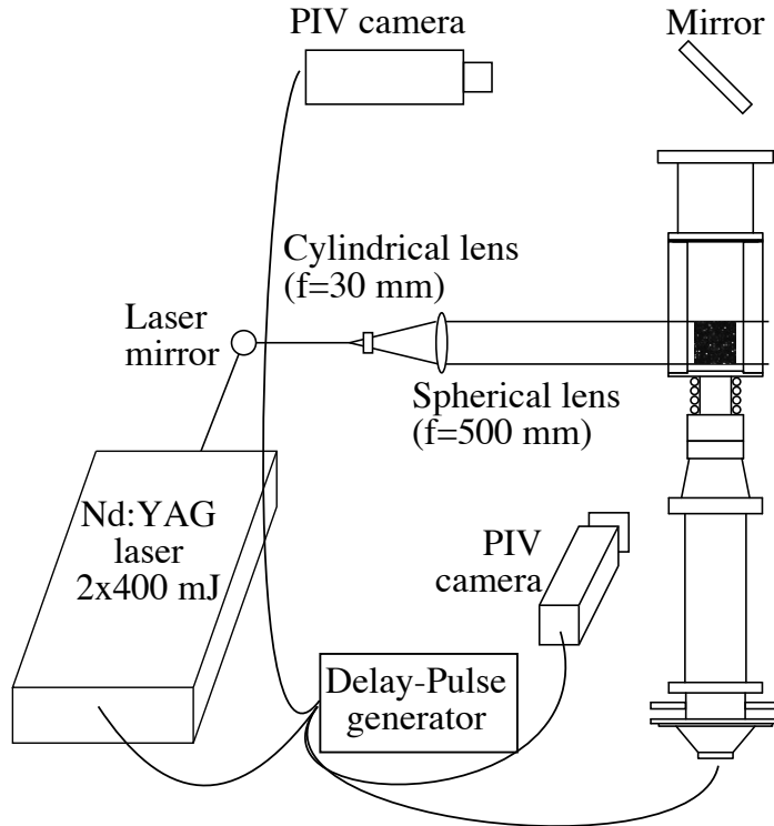
Figure 2.6: PIV setup
