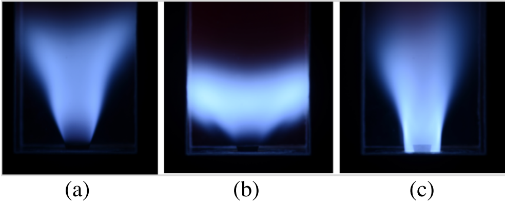
Figure 4.2: Swirl number effect on flame stabilization. (a) SW_1 , D_o = 18 mm, C = 14 mm, S = 0.48^* , elongated flame close to blow off. (b) SW_3 , D_o = 20 mm, C = 12 mm, S = 0.73 , well-stabilized flame. (c) SW_3 , D_o = 22 mm, C = 10 mm, S = 0.86^* , flash back. The equivalence ratio \phi = 0.82 , the bulk flow velocity U_b = 5.44 m/s at the hot-wire location and the distance \delta = 50 mm, are fixed.
