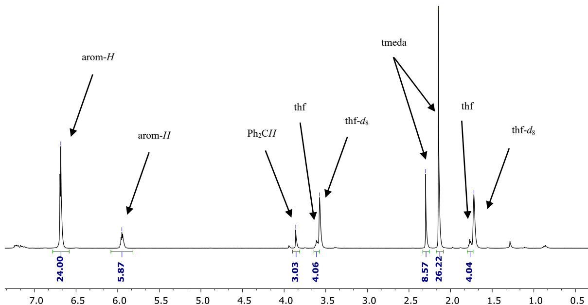
Figure 5.13. Spectre RMN ^1\text{H} (298 K, \text{thf-}d_8 , 500 MHz) du complexe [\text{Li}(\text{tmeda})_2]^+.\text{Ca}(\text{CHPh}_2)_3(\text{thf})^- ( 19 ).
