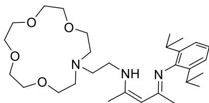
{BDI crown }H
