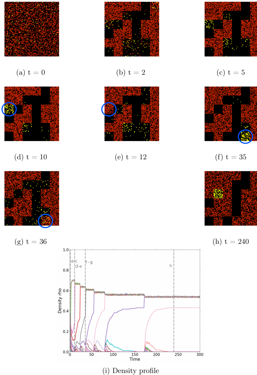
Figure 2.3 – Evolution of the city for p = 0.03, Q = 36 and H = 225 . Panels (a-h) show the occupation of the different neighborhoods at different times. Egoists are represented in red, altruists in yellow, empty sites in black. (a) initial; (b) first steps; (c) usual segregation; (d-e): first invasion and altruist escape from the block surrounded in blue; (f-g): final invasion of the block surrounded in blue; (h): stationary state. In panel (i), each continuous line represents the evolution of the density of a single neighborhood. Vertical dashed lines show the times corresponding to panels (a-h).
