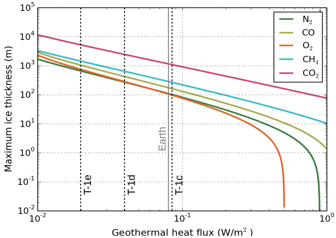
Figure 4.8: Maximum nightside thickness of various types of ice ( N_2 , CO , O_2 , CH_4 and CO_2 ) - assuming that it is limited by basal melting - as a function of the geothermal heat flux. It is assumed here that the entire atmosphere has collapsed at the cold points of the planet and that the surface temperature at the top of the glacier is controlled by the geothermal heat flux. As a reference, vertical dashed lines indicate the average surface tidal heat flux on TRAPPIST-1 planets derived from Table 4.2, for a tidal dissipation equal to that of the Earth. We also added (vertical solid gray line) the average geothermal heat flux on Earth, to give the reader a rough sense of the amplitude of the radiogenic heating on TRAPPIST-1 planets. These quantities can be numerically converted in term of global equivalent surface pressure when multiplied by a factor \frac{\rho g}{2} . The thermodynamical and rheological properties of the ices were taken from https://encyclopedia.airliquide.com , http://webbook.nist.gov , Roder (1978); Schmitt et al. (1997); Fray and Schmitt (2009); Trowbridge et al. (2016), and Umurhan et al. (2017). Missing rheological data were mimicked on N_2 .
