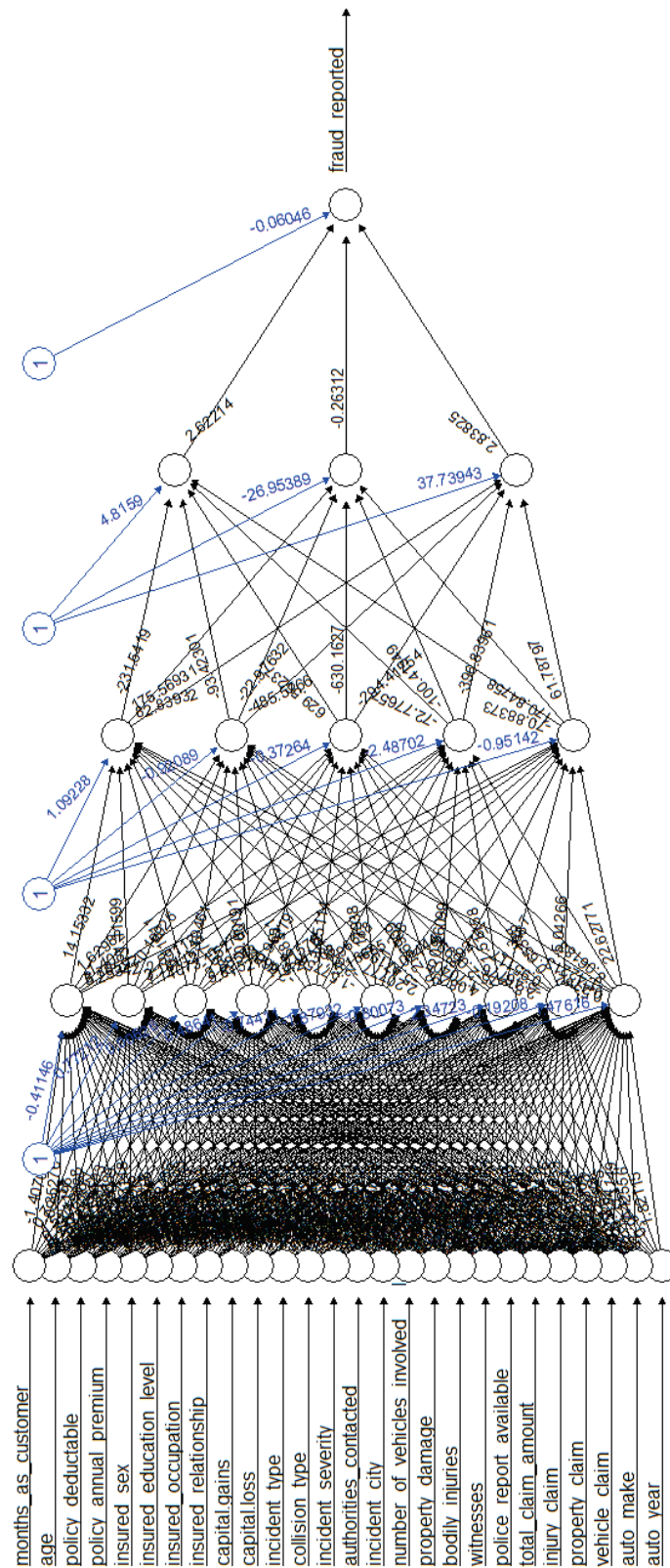
Fig. 5.23 ANN architecture
