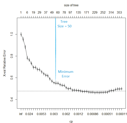
Fig. 5.22 Trees errors
