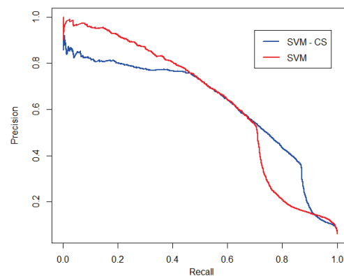
Fig. 2.6 PR curves for SVM methods
