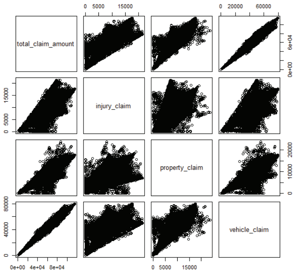
Fig. B.2 Pairs of scatter plot of variables with high VIF - case study 3
