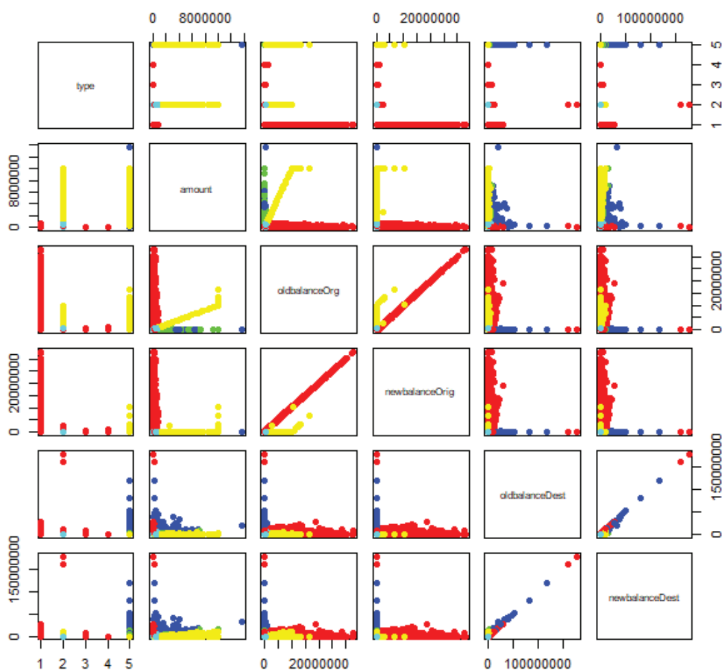
Fig. 5.13 Pairs of the explanatory variables scatter plots colored by the clusters - case study 2
