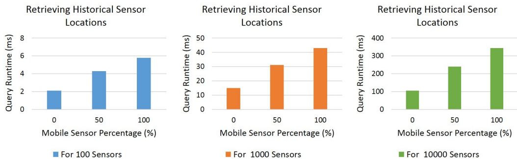
FIGURE 2.21: Mobility impact on previous location retrieval
