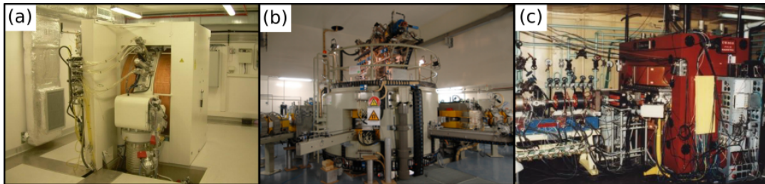
FIGURE 3.1: Photos of the cyclotrons employed in this work: (a) GE PETtrace in Heavy Ion Laboratory, (b) C70 in ARRONAX, (c) C30 in National Centre for Nuclear Research.
