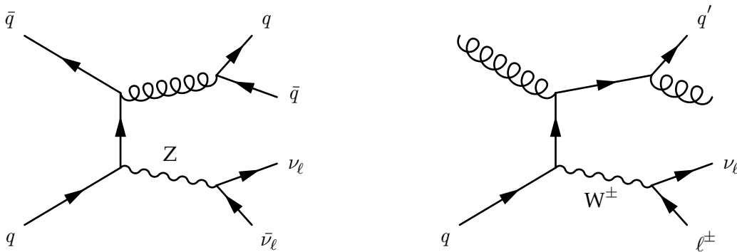
FIGURE 5.3: Example Feynman diagrams for the V +jets background.
