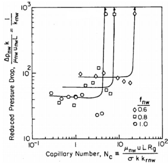
Figure 1-10: The sudden increase in reduced pressure drop across the medium, at a significant capillary number after which foam has generated, for three different liquid fractional flows. Taken from Ransohoff and Radke (1988).
