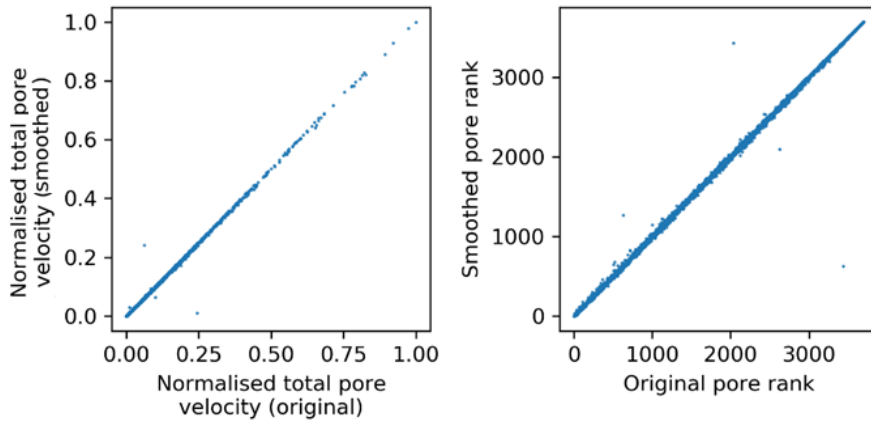
Figure 2-27: Comparison of pore pixel totals and corresponding ranks in smoothed versus unsmoothed images of the flow map. The units of the plot on the left are normalized to 1 for clarity, but by a same factor in both cases (conserved total intensity of Gaussian filter).
