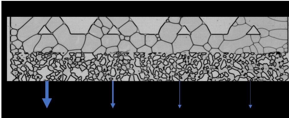
Figure 3-25: Foam dryness gradient over the model inlet for experiment A4, and the effects on the flow distribution that this causes.
