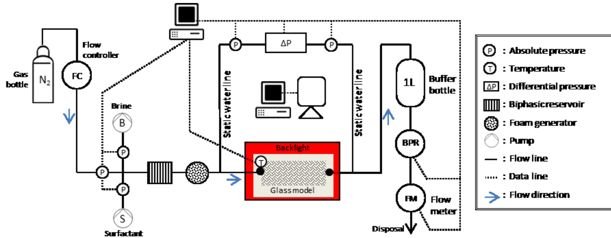
Figure 2-3: Experimental Setup
