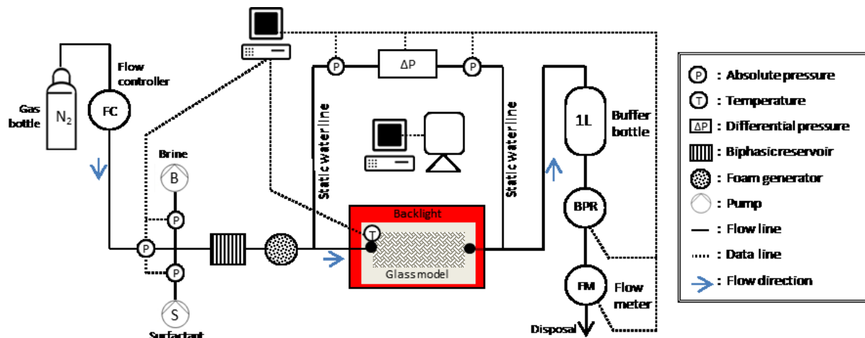
Figure 2-3: Experimental Setup
