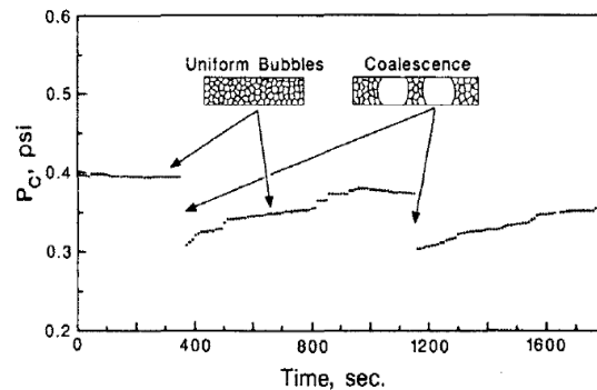
Figure 1-19: Capillary pressure adaptation via bubble coalesce, creating heterogeneity of bubble distribution. Taken from Khatib et al. (1988).
