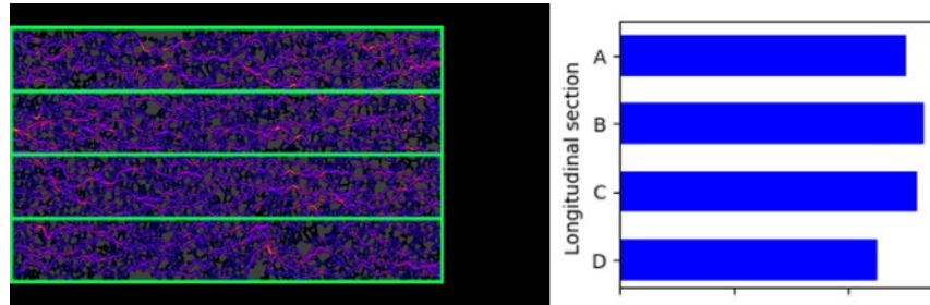
Figure 2-19: Box analysis principle, flow is integrated in each longitudinal box.
