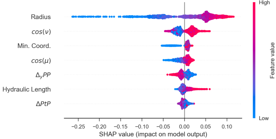
Figure 4-23 : SHAP values obtained for each feature and sample in the test set for the lower activity throat classification. We note that the most important features shown here exhibit small differences with the features shown on the left bar plot of Figure 4-22, owing to the differences in total feature importance calculation.
