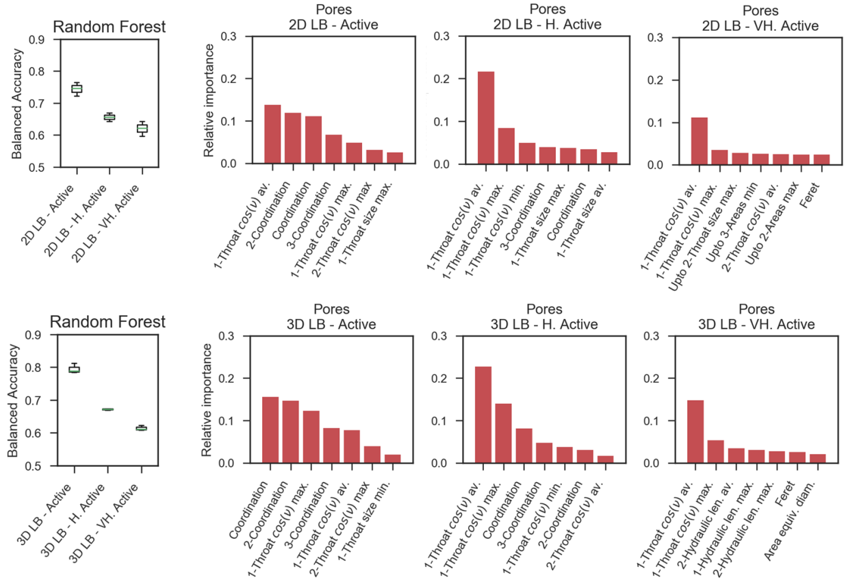
Figure 4-20: Achieved balanced accuracy and feature importance for the pore classification predictions of the two numerical flow maps. Top row: 2D numerical flow map results. Bottom: 3D numerical flow map results.
