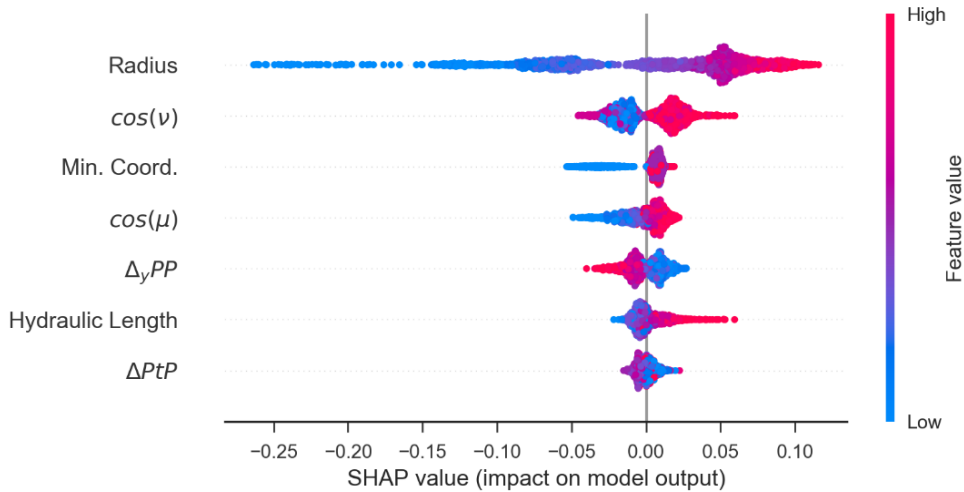
Figure 4-23: SHAP values obtained for each feature and sample in the test set for the lower activity throat classification. We note that the most important features shown here exhibit small differences with the features shown on the left bar plot of Figure 4-22, owing to the differences in total feature importance calculation.
