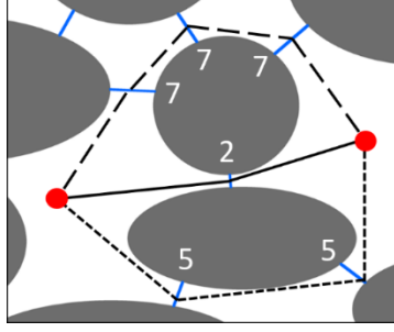
Figure 5-3: Motivational example. Optimal paths for different values of \alpha in a schematic example. Porous space is shown in white between gray solid obstacles. Throats are shown in blue. Multiple paths link the sources and destination pores, shown in red. Throat size values are given in white, next to the relevant throats. For \alpha = 0 the path shown by full black line is optimal, for \alpha = 1 the path shown by the thinly dashed path is optimal, for \alpha = 2 the path shown by thickly dashed line is optimal.
