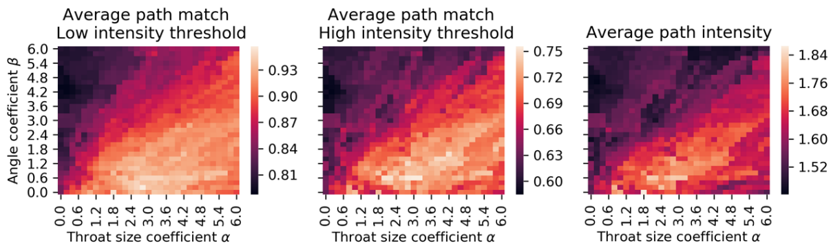
Figure 5-22: Model parameter optimization for the reversed flow experiment C1.
