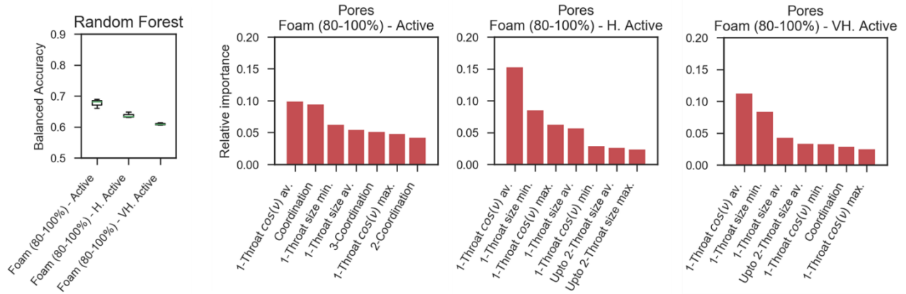
Figure 4-19: Achieved balanced accuracy and feature importance of pore activities for the top 20% bubble size flowmap of experiment A1.
