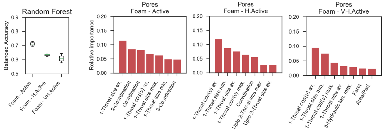
Figure 4-13: Feature importance for the classification of pore activities for all bubble sizes for experiment A1.
