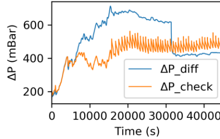
Figure 3-8. Time evolution of pressure drops for experiment A3, which uses the I1 injection method, (i.e. pressure measurement point on the micromodel central hole). The pressure drop value taken was calculated from the points taken after the discontinuity. The discontinuity was attributed to gas or bubbles in the outlet pressure line.
