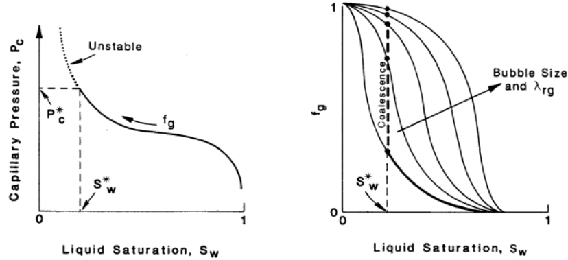
Figure 1-16: The attainment of the critical capillary pressure P_c^* at the critical saturation S_w^* (left) and the coalescence mechanism maintaining the critical liquid saturation at increasing gas fraction (right). Adapted from Khatib et al. (1988).
