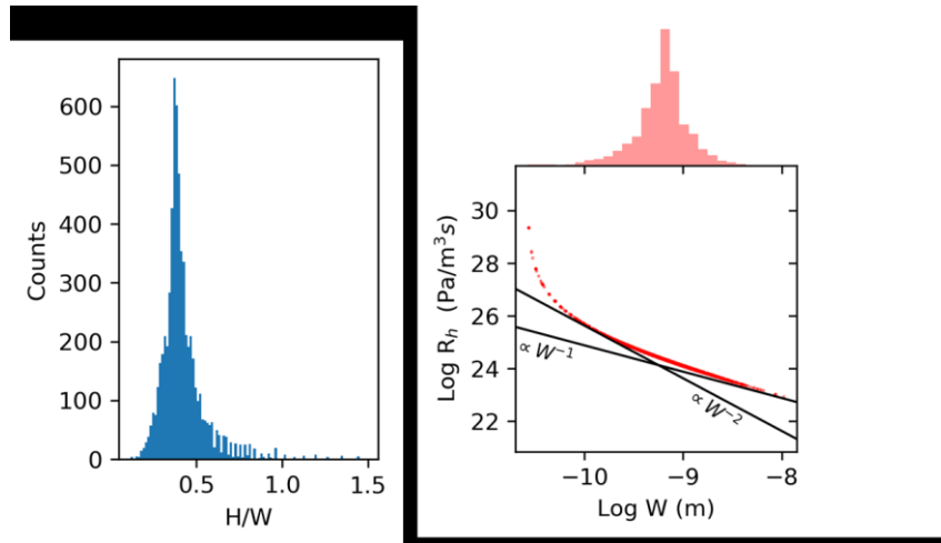
Figure 5-13: Aspect ratio H/W distribution (left) and distribution of hydraulic resistance (right).
