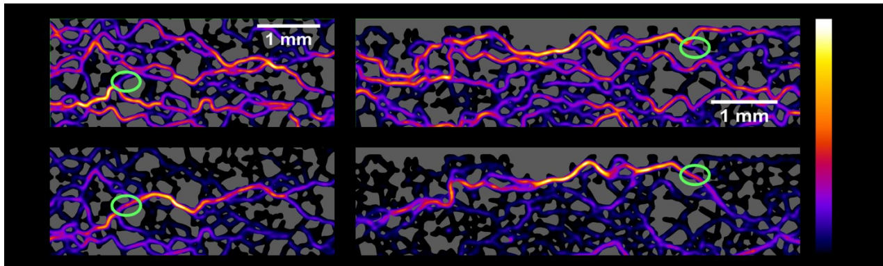
Figure 5-16: Comparison of flow maps for two areas of interest for each experiment. We observe flow path deviation perpendicular to pressure gradient in experiment 2, while access to these zones is denied by the presence of other flow paths in Experiment 1. We circle in green the exact access links that are crucial in keeping the flow in the straighter paths for the high-velocity experiment. Flow is from left to right in both examples. Note: colormap contrast has been forced in each example for clarity.
