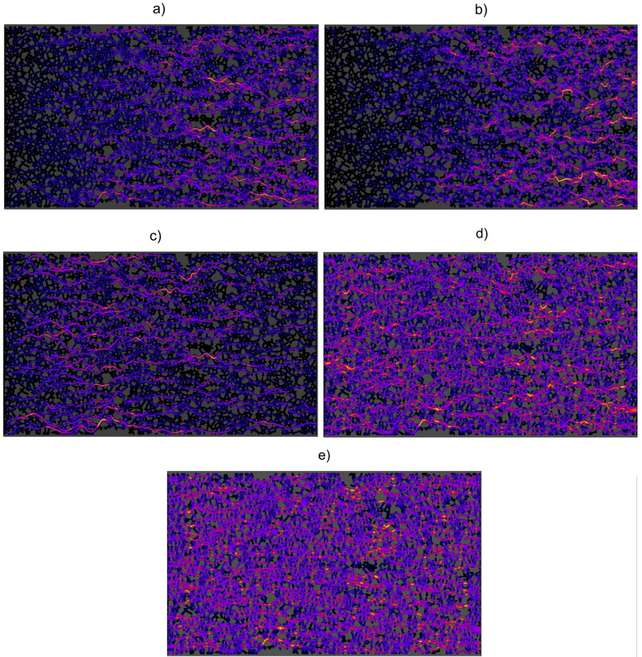
Figure 2-6: Different velocity maps using the same model. Injections are from left to right. a) Foam flow, all bubble sizes. b) Foam flow, smallest 20% of bubbles. c) Foam flow, largest 20% of bubbles. d) 2D Numerical Newtonian flow. e) 3D Numerical Newtonian flow.
