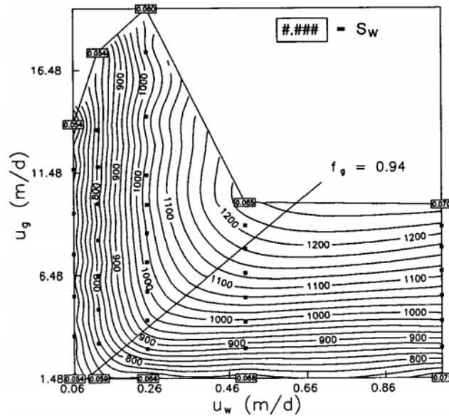
Figure 1-12: An example of the measured pressure differences over a series of injection rates for a two-inch sandpack. The high-quality or coalescence regime is visible in the top left side whereas the low-quality regime is in the bottom right side. The transition occurs at a foam quality of f_g = 0.94 .
