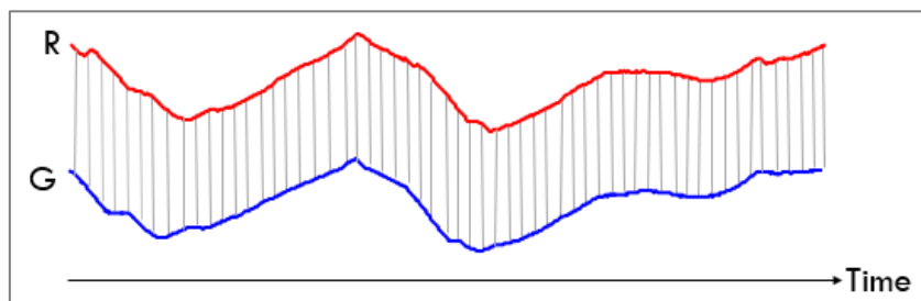
Figure 4.3: Warping between of two sequences
