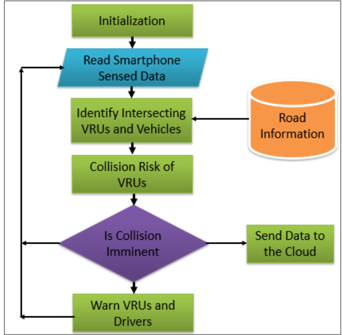
Figure 3.2: Flowchart of VRU collision prediction algorithm
