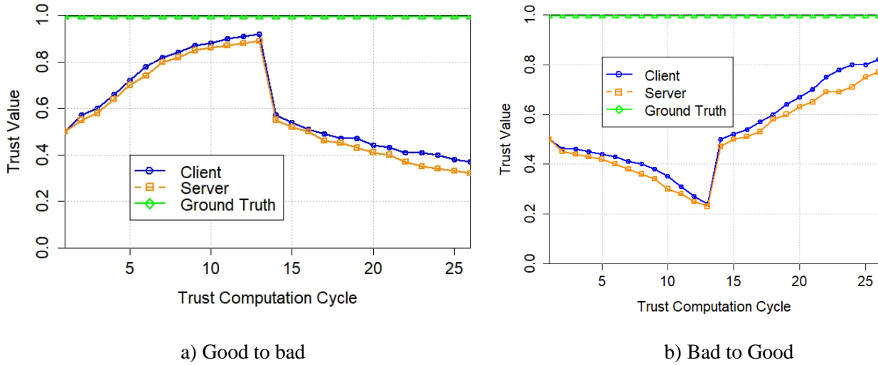
Figure 7.9: Change of behavior of nodes a) from Good to Bad and b) from Bad to Good
