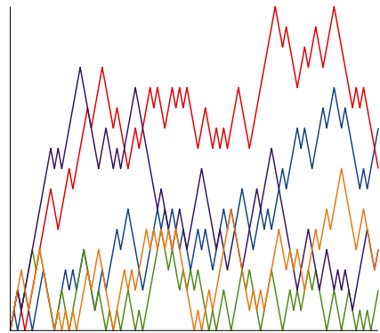
Five trajectories of Dyck 100 step walk
