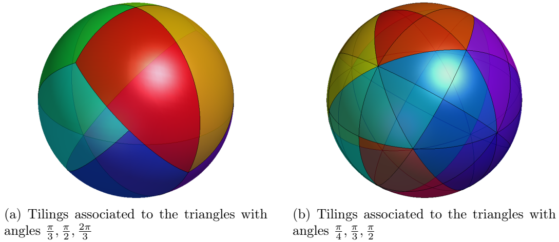
Figure 5.13 – Various tilings of the sphere. These triangles correspond to the lines 9 and 17 in Table 5.3
