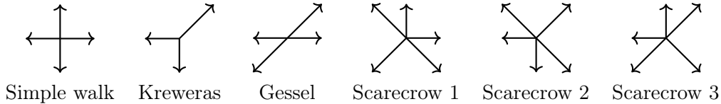
Figure 5.8 – Some 2D models. The three scarecrows are named after [34, Fig. 1]
