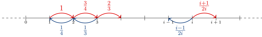
Figure 1.4 – Random walk (T_n)_{n \in \mathbb{N}} . This is a Doob transform of a simple random walk over \mathbb{N}
