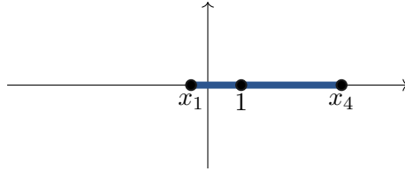
Figure 4.3 – Cut plane \mathbb{C} \setminus [x_1, x_4]
