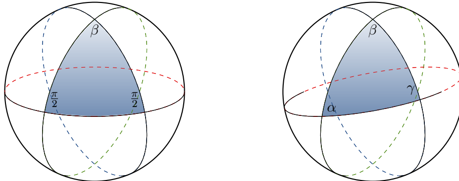
(a) A particular spherical triangle with two right angles (these triangles will eventually correspond to Hadamard models)
