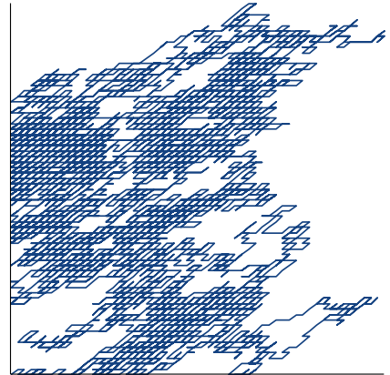
A Gessel 10,000 step walk in the quarter plane
