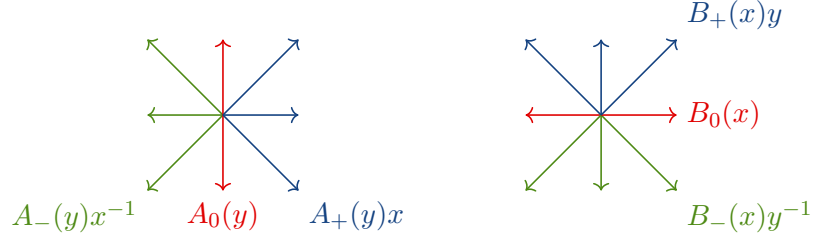
Figure 2.1 – Decomposition of the inventory polynomial (2.4)
