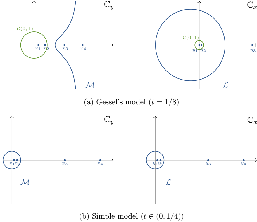
Figure 2.6 – The curves \mathcal{L} and \mathcal{M} for two models
