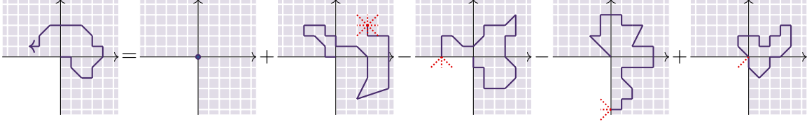
Figure 2.4 – Different ways to end in the three-quadrant (example of the king walk) Illustration of the functional equation (2.10) for the example of the king walk. The right-hand side describes the different ways to end in the three-quadrant making sure to remove the walks going out of the three-quadrant
