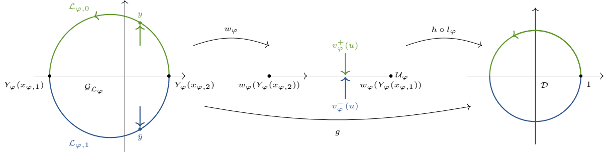
Figure 3.9 – Conformal gluings from \mathcal{G}_{\mathcal{L}_\varphi} to \mathbb{C} \setminus \mathcal{U}_\varphi and conformal mappings from \mathcal{G}_{\mathcal{L}_\varphi} to the unit disc \mathcal{D}
