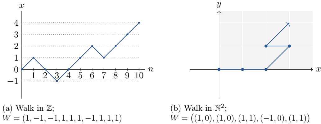
Figure 1.1 – Walks in various cones
