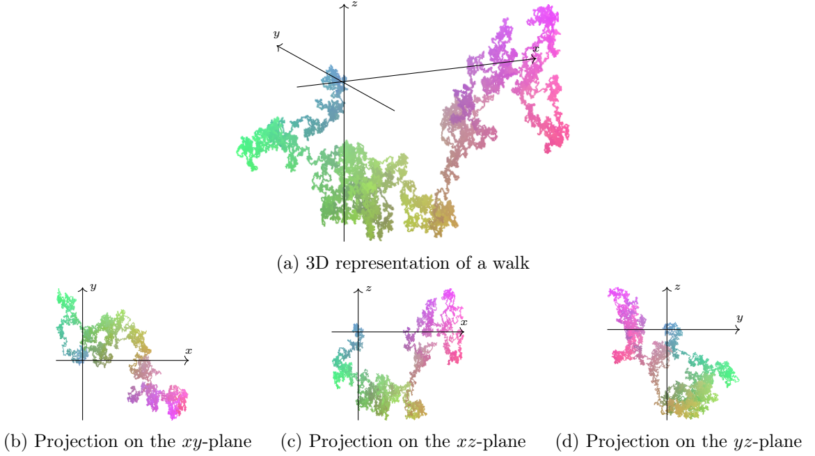
Figure 5.18 – A 3D walk avoiding the negative octant
