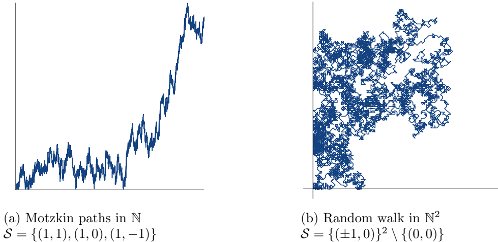
Figure 5.1 – Walks in \mathbb{N} and \mathbb{N}^2
