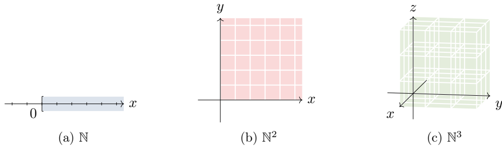
Figure 1.2 – Some cones of restriction
