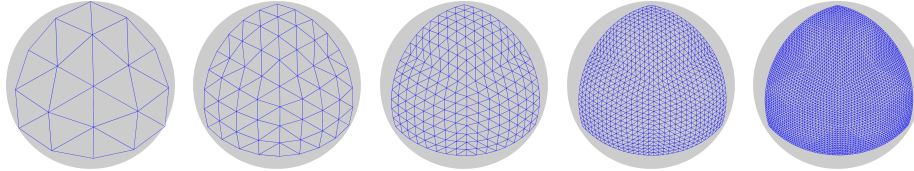
Figure 5.17 – Triangulation of a spherical triangle using successive refinements
