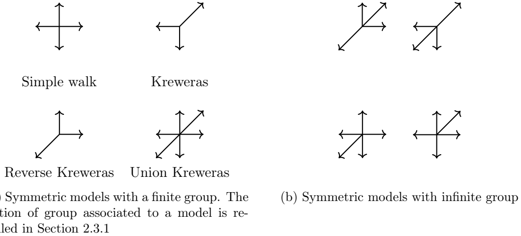
Figure 3.2 – Symmetric models with no jumps (-1, 1) and (1, -1)
