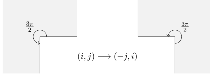
Figure 4.7 – Various cones of opening angle \frac{3\pi}{2} , see Remark 33. On the left the cone \{R \exp(is) : 0 \leq R < \infty, 0 \leq s \leq \frac{3\pi}{2}\} and the right the cone \{R \exp(is) : 0 \leq R < \infty, -\frac{\pi}{2} \leq s \leq \pi\}
