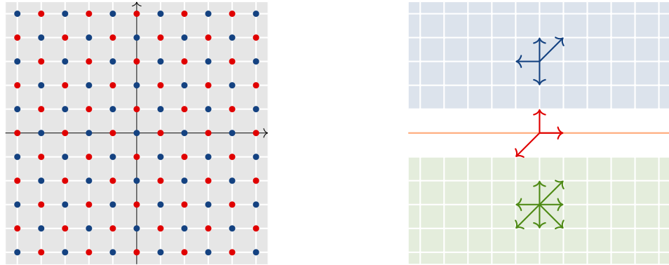
(a) An example of spatially inhomogeneous model studied in [35, 111, 45] (b) Block inhomogeneous model in the plane
