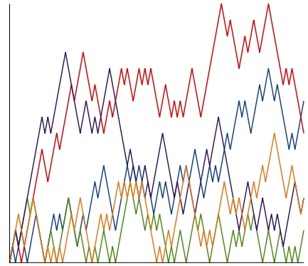
Five trajectories of Dyck 100 step walk
