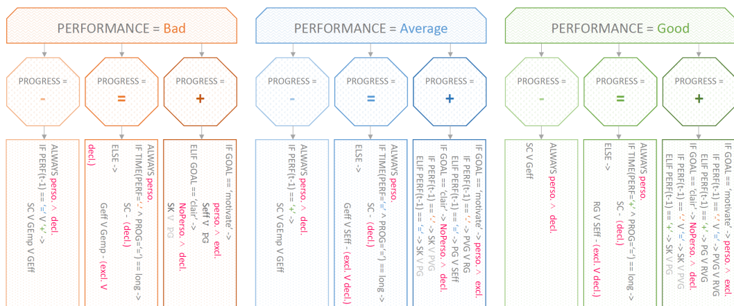
Figure 4.3: The rule tree corresponds to a set of rules that selects the interventions of PEANUT (i.e., type and mode of sentence) depending on users’ performance and progression (“-”=negative, “=”=neutral, “+”=positive). Type of sentences: “perso.” for personal, “NoPerso.” for non-personal ; Mode of the sentence: “decl.” for declarative, “excl.” for exclamatory. Interventions: “GEff” for general effort, “SEff” for support effort, “GEmp” for general empathy, “SK” for strategy keep, “SC” for strategy change, “RG” for results good, “RVG” for results very good, “PG” for progress good, “PVG” for progress very good. Moreover, the “^” sign represents the logical operator “and” and the “v” sign represents the logical operator “or”.
