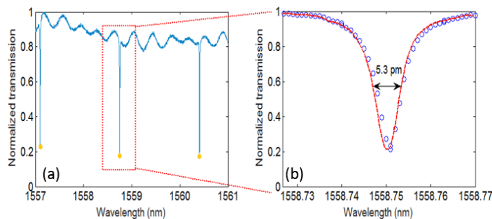
Figure 58-Normalized transmission of a 112-μm radius silicon nitride ring with a cross section of 1500 nm x740 nm. (the space between the ring and the bus waveguide is 300 nm)
