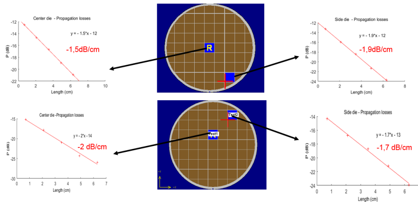
Figure 57- Cross-die and cross wafer propagation loss measurements with the automated prober via the cut-back method for the waveguide of 740 nm x 750 nm cross-section dimensions at 1550 nm and for TE polarized light.
