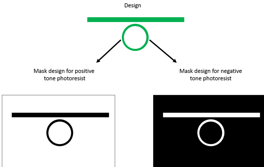
Figure 46- Intended design, mask design for positive and negative tone photoresist.
