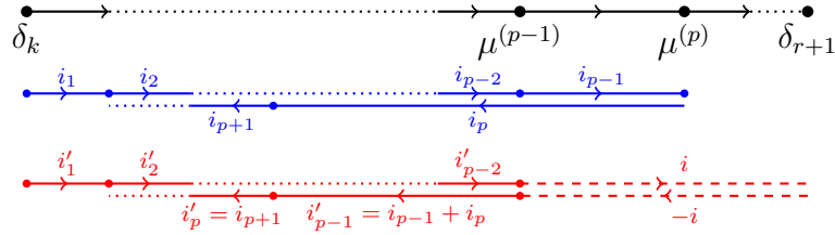
FIGURE 3.3 – \underline{i} = \text{ht}(\underline{\mu}) and \underline{i}' := \text{ht}(\underline{\mu}^{\#p}) for the case i_{p-1} + i_p < 0
