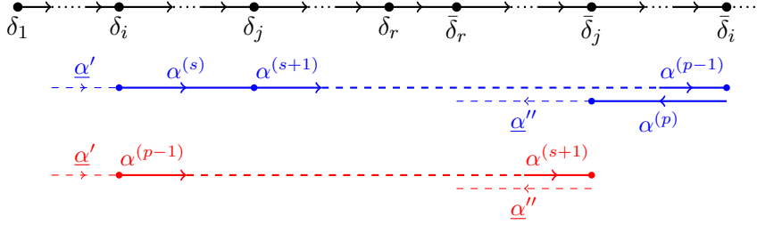
FIGURE 4.7 – The case for \alpha^{(p)} = \bar{\delta}_i - \bar{\delta}_j and \alpha^{(s)} = \delta_i - \delta_j .
