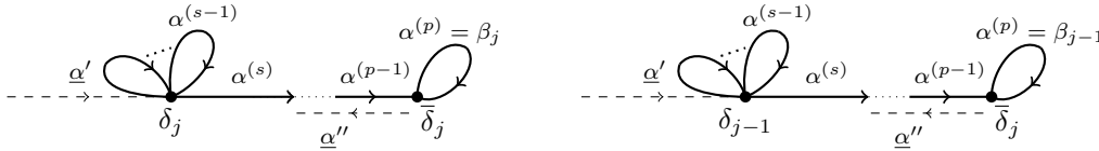
FIGURE 4.8 – Path in case p < q and \mu^{(p)} = \bar{\delta}_j
