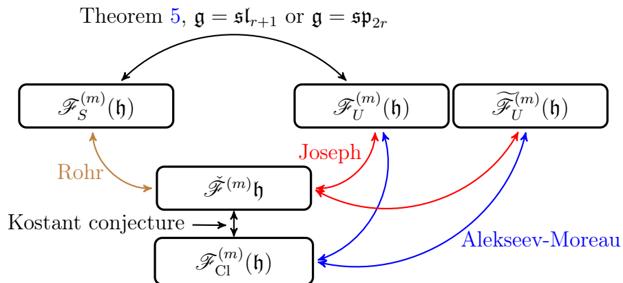
FIGURE 1 – Connections between several filtrations on the Cartan subalgebra \mathfrak{h} .
