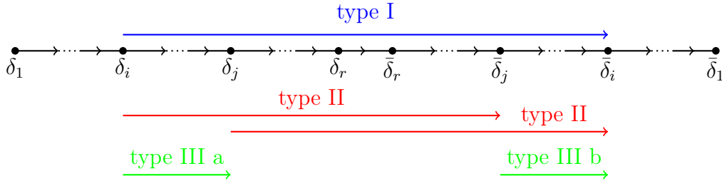
FIGURE 2.3 – The types of admissible triple (\alpha, \mu, \nu) in \mathfrak{g} = \mathfrak{sp}_{2r} .
