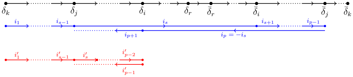
FIGURE 4.11 – \underline{i} = \text{ht}(\underline{\mu}) and \underline{i}' := \text{ht}(\underline{\mu}^{*1}) where \alpha^{(p)} = \bar{\delta}_j - \delta_i , \alpha^{(s)} = \delta_j - \bar{\delta}_i , j < i .
