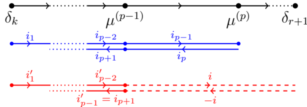
FIGURE 3.4 – \underline{i} = \text{ht}(\underline{\mu}) and \underline{i}' := \text{ht}(\underline{\mu}^{\#p}) for the case i_{p-1} + i_p = 0
