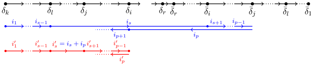
FIGURE 4.9 – \underline{i} = \text{ht}(\underline{\mu}) and \underline{i}' := \text{ht}(\underline{\mu}^{*1}) where \alpha^{(p)} = \bar{\delta}_j - \delta_i , \alpha^{(s)} = \delta_l - \bar{\delta}_i , l < j < i .
