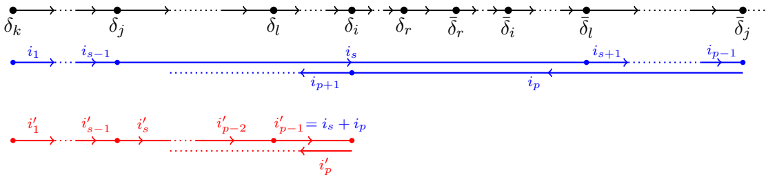
FIGURE 4.10 – \underline{i} = \text{ht}(\underline{\mu}) and \underline{i}' := \text{ht}(\underline{\mu}^{*1}) where \alpha^{(p)} = \bar{\delta}_j - \delta_i , \alpha^{(s)} = \delta_j - \bar{\delta}_l , j < l < i .
