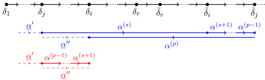
FIGURE 4.6 – The case for \alpha^{(p)} = \bar{\delta}_j - \delta_i and \alpha^{(s)} = \delta_j - \bar{\delta}_i .
