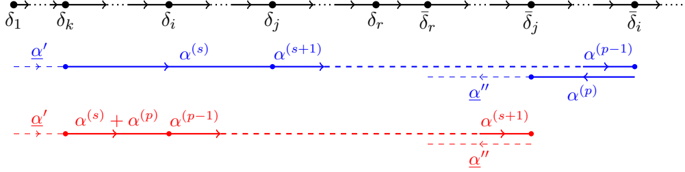
FIGURE 4.5 – The case for \alpha^{(p)} = \bar{\delta}_i - \bar{\delta}_j and \alpha^{(s)} = \delta_k - \delta_j .
