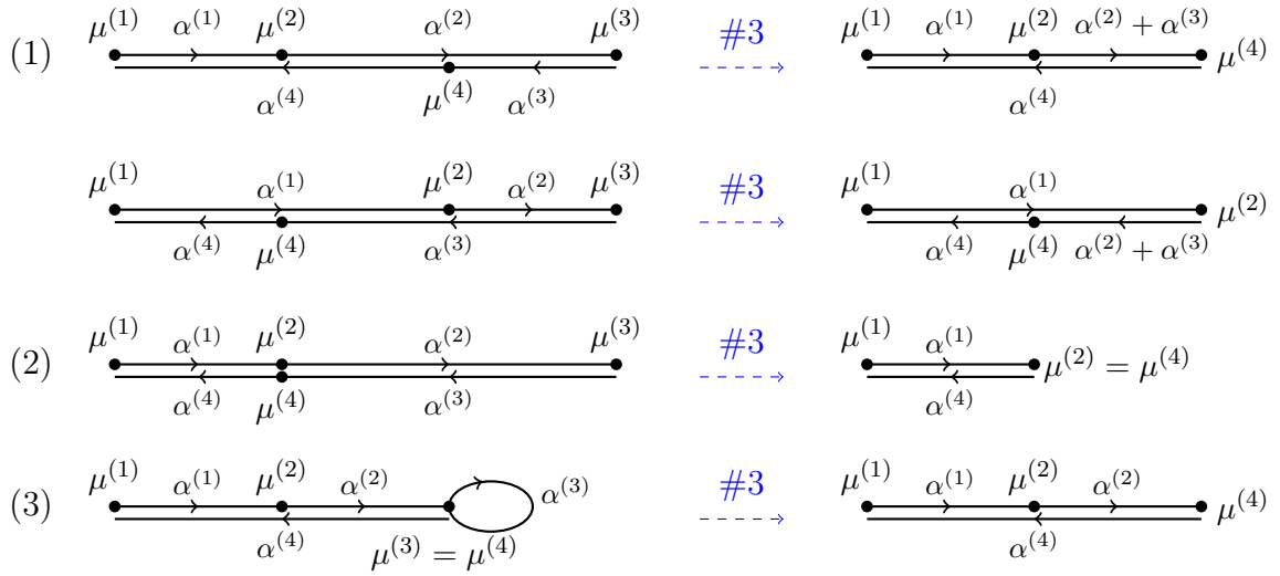
FIGURE 1.3 – Cutting the vertex \mu^{(3)}
