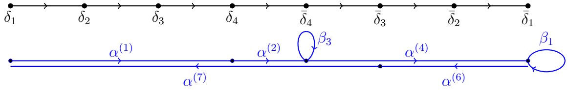
FIGURE 1.2 – An example of weighted path in \mathfrak{sp}_8 .
