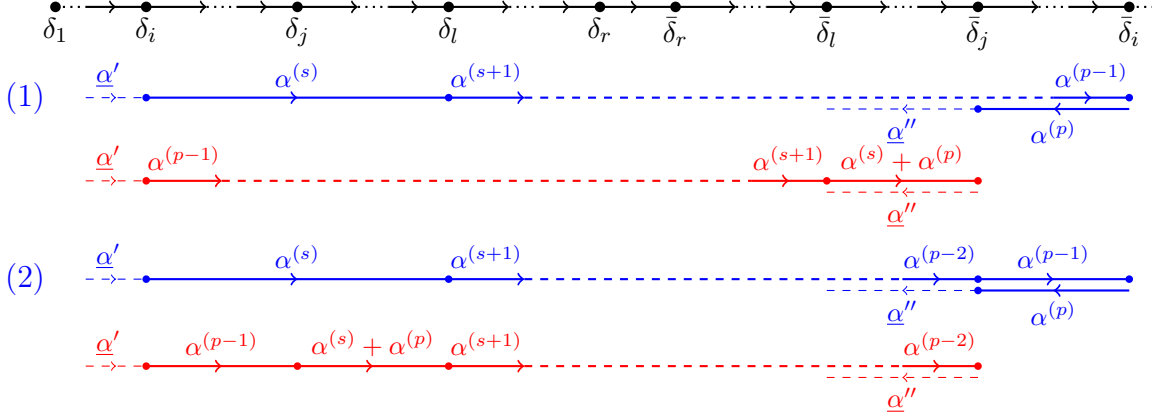
FIGURE 4.4 – The case for \alpha^{(p)} = \bar{\delta}_i - \bar{\delta}_j and \alpha^{(s)} = \delta_j - \delta_l .
