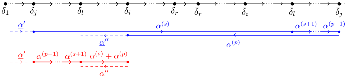
FIGURE 4.2 – The case for \alpha^{(p)} = \bar{\delta}_j - \delta_i and \alpha^{(s)} = \delta_j - \bar{\delta}_l .
