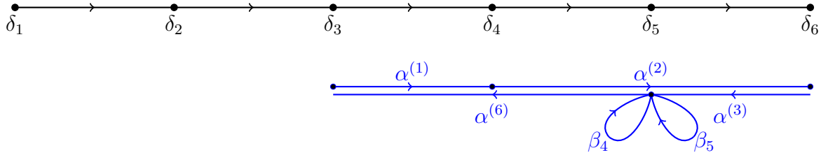
FIGURE 1.1 – An example of weighted path in \mathfrak{sl}_6 .
