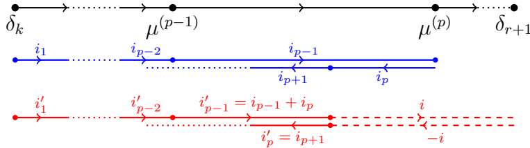
FIGURE 3.2 – \underline{i} = \text{ht}(\underline{\mu}) and \underline{i}' := \text{ht}(\underline{\mu}^{\#p}) for the case i_{p-1} + i_p > 0
