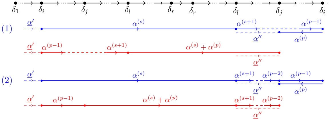
FIGURE 4.3 – The case for \alpha^{(p)} = \bar{\delta}_i - \bar{\delta}_j and \alpha^{(s)} = \delta_i - \bar{\delta}_l .
