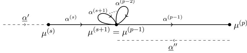
FIGURE 3.1 – Path in case (2) (b)
