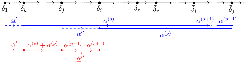
FIGURE 4.1 – The case for \alpha^{(p)} = \bar{\delta}_j - \delta_i and \alpha^{(s)} = \delta_k - \bar{\delta}_i .
