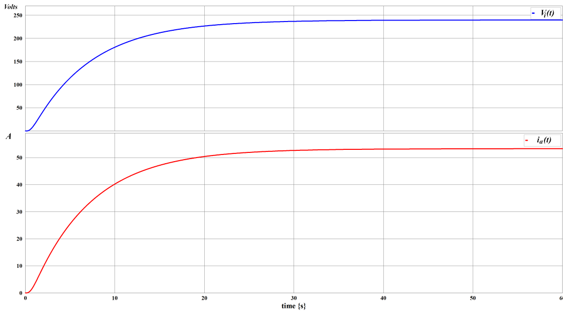
Figure 5.13 – Voltage and current applied to the Load.
