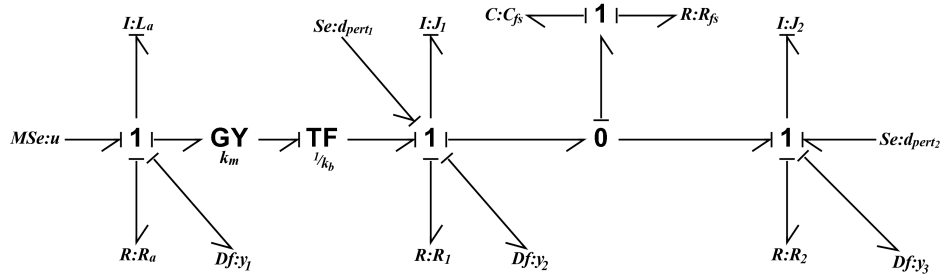
Figure 1.4 – Simplified Bond Graph of the Torsion-Bar system.
