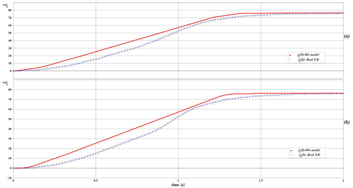
Figure 1.8 – Data from the outputs of real T-B system (blue) compared with outputs from BG model (red).
