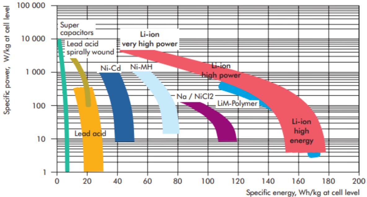
Figure 2.1: Ragone Plot (Specific Power vs Specific Energy) for Commercial Battery Storage Technologies [85].
