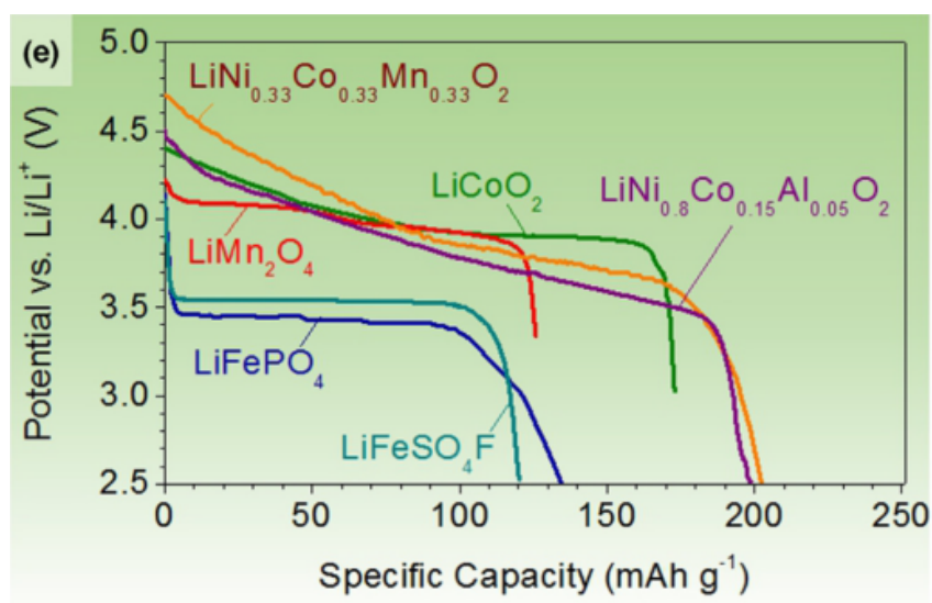
Figure 2.9: Lithium Ion Battery Discharge Profiles by Chemistry [109].
