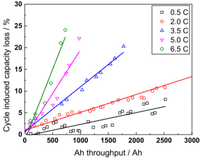
Figure 2.24: Cycle life loss is plotted as a function of Ah-throughput at 10 °C for 5 different charge rates: C/2 , 2C , 3.5C , 5C , and 6.5C rate. Linear fits (lines) were achieved, indicating the capacity loss follows linear trend with Ah throughput or time for the LMO-NMC chemistry [98].
