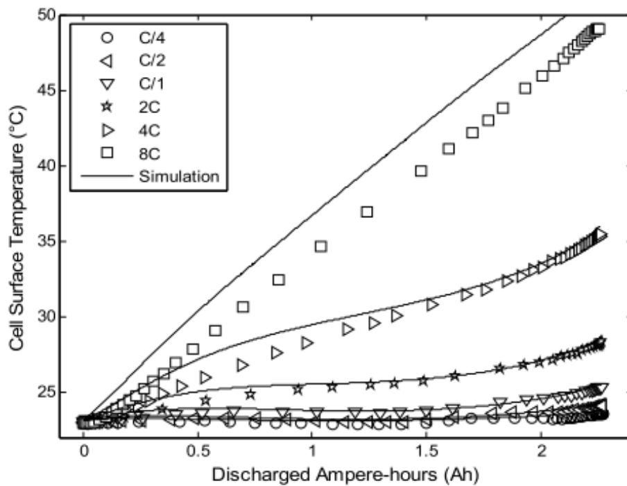
Figure 2.13: C-rate Effect on Cell Temperature (Discharge) [129].
