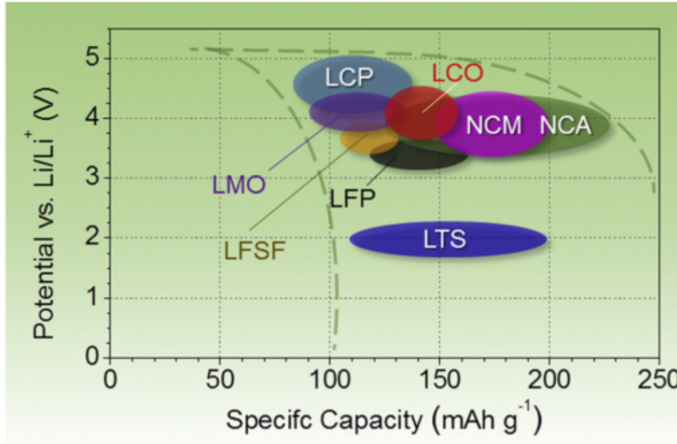
Figure 2.3: Specific Capacity vs Cell Potential of Intercalation Cathode Materials [109].
