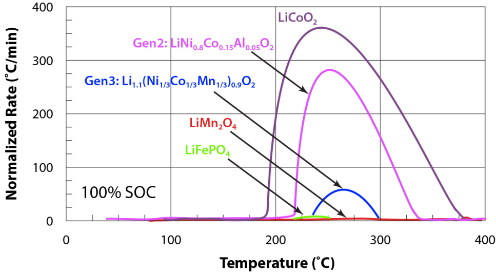
Figure 2.4: Thermal Runaway Characteristics of LCO (dark purple) NCA (light purple), NMC (blue), LMO (red), and LFP (green) chemistries [118].
