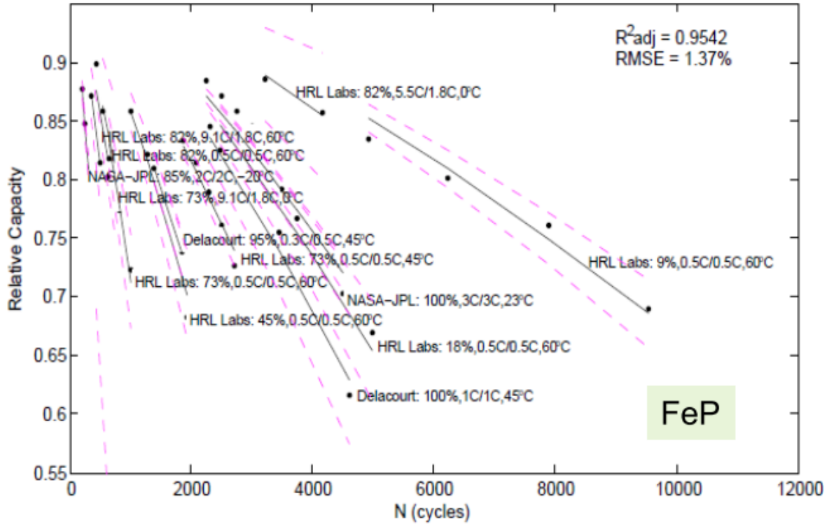
Figure 2.22: NREL Model Fit (Solid Black Lines) with Updated Knee Region Parameter ( C1 ) Compared to LFP Meta-Dataset (Points) [139].
