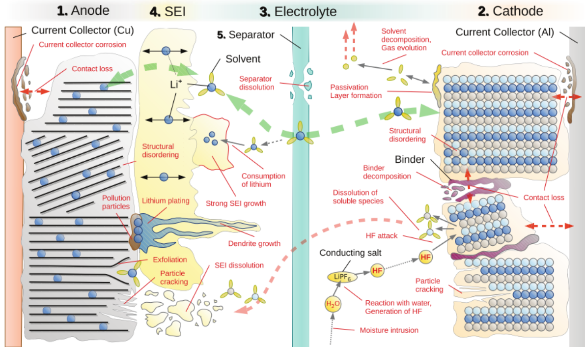
Figure 2.5: Lithium Ion Battery Aging Mechanisms and Battery Cell Structure [119].
