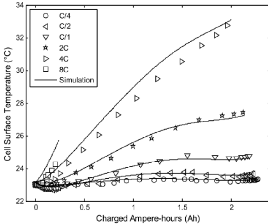
Figure 2.12: C-rate Effect on Cell Temperature (Charge) [129].
