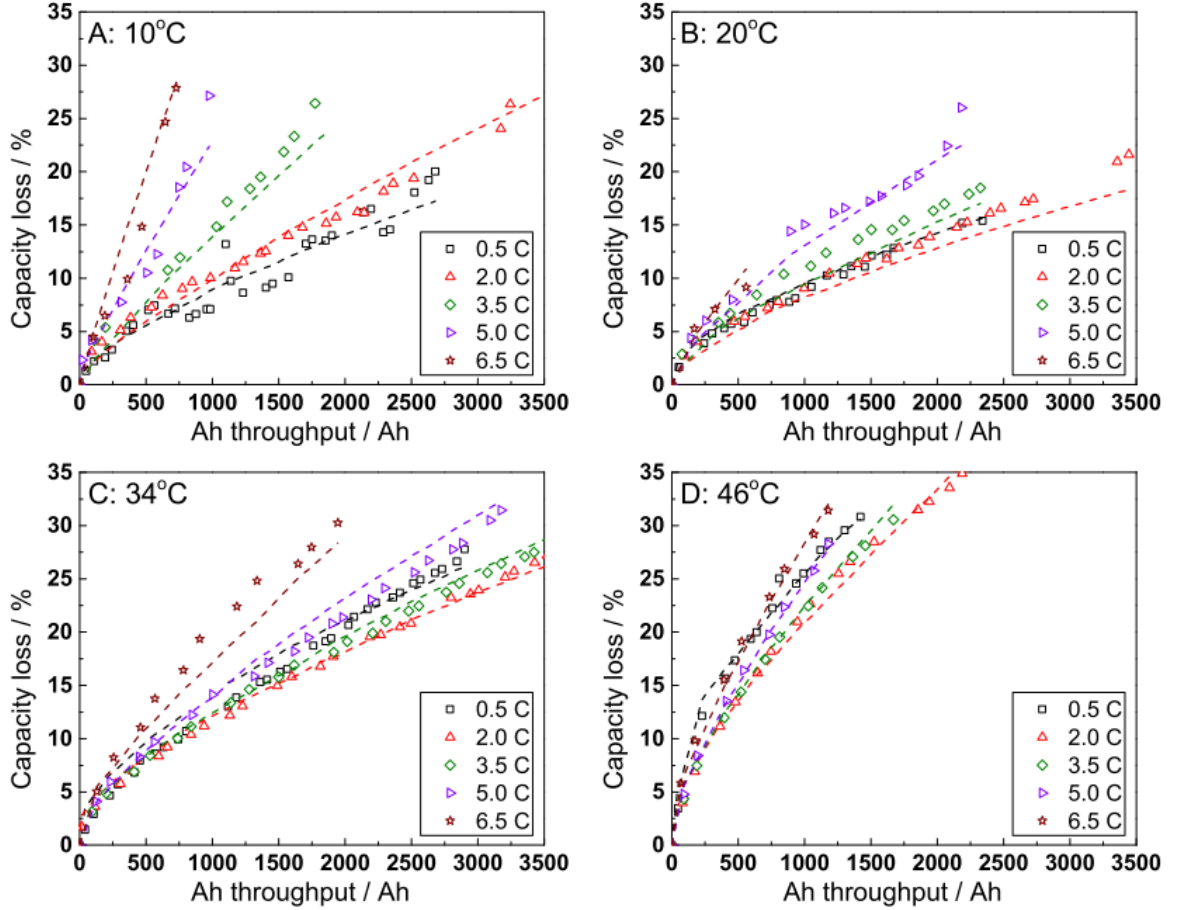
Figure 2.25: Simulations of combined Calendar Aging and Cycling Aging prediction model (line) are compared with experimental data (markers) for four temperatures (10, 20, 34, and 46 °C), five C-rates (C/2, 2C, 3.5C, 5C, and 6.5C) and at 50% DOD for LMO-NMC chemistry [98].
