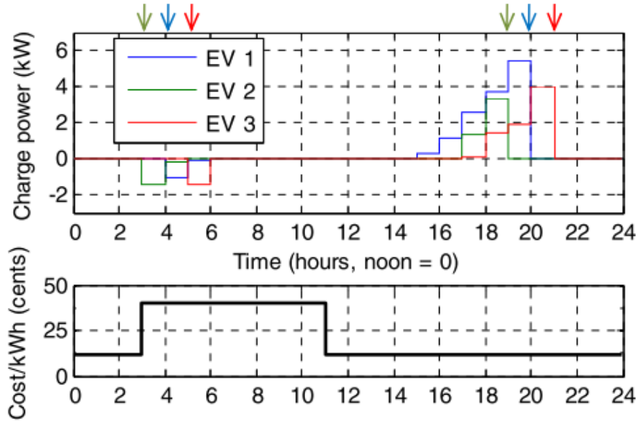
Fig. 9. Optimized charging of 3 EVs showing V2G operation
