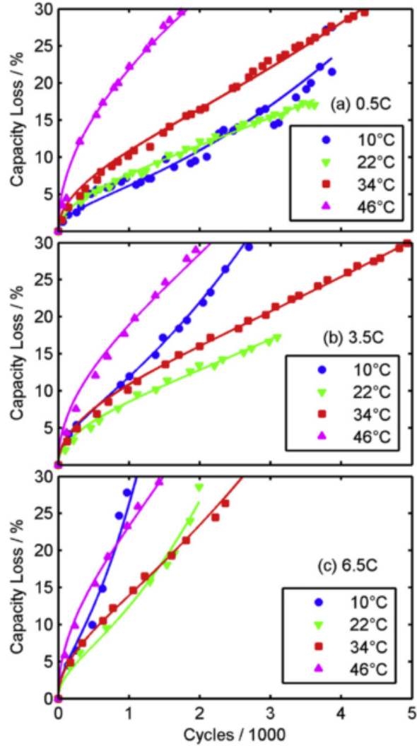
Figure 2.10: C-rate Effect on Capacity Fade at T = 10^\circ\text{C} , 22^\circ\text{C} , 34^\circ\text{C} , 46^\circ\text{C} . The panels each correspond to a single C-rate ( 0.5C , 3.5C , 6.5C , respectively). DoD is 50% for all data points [98].
