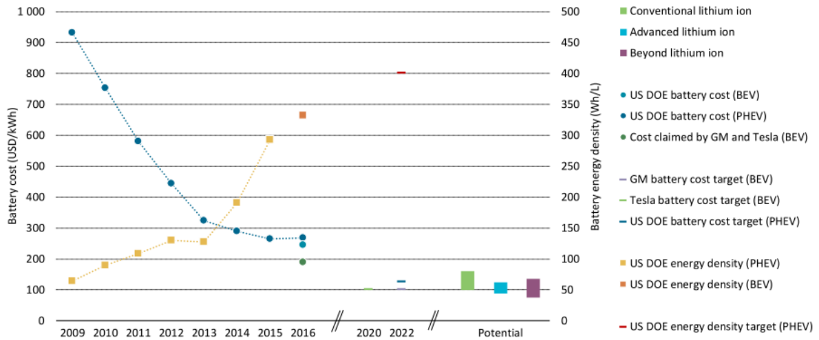
Figure 2.2: Observed Li-ion Battery Cost Trends (blue, left axis) and Energy Density Evolution (yellow, right axis) [2]. Note for 2018 that Tesla/Panasonic have claimed a battery cell cost of $111 per kWh, LG Chem cell cost $148 per kWh, and Audi cell cost $114 [84].
