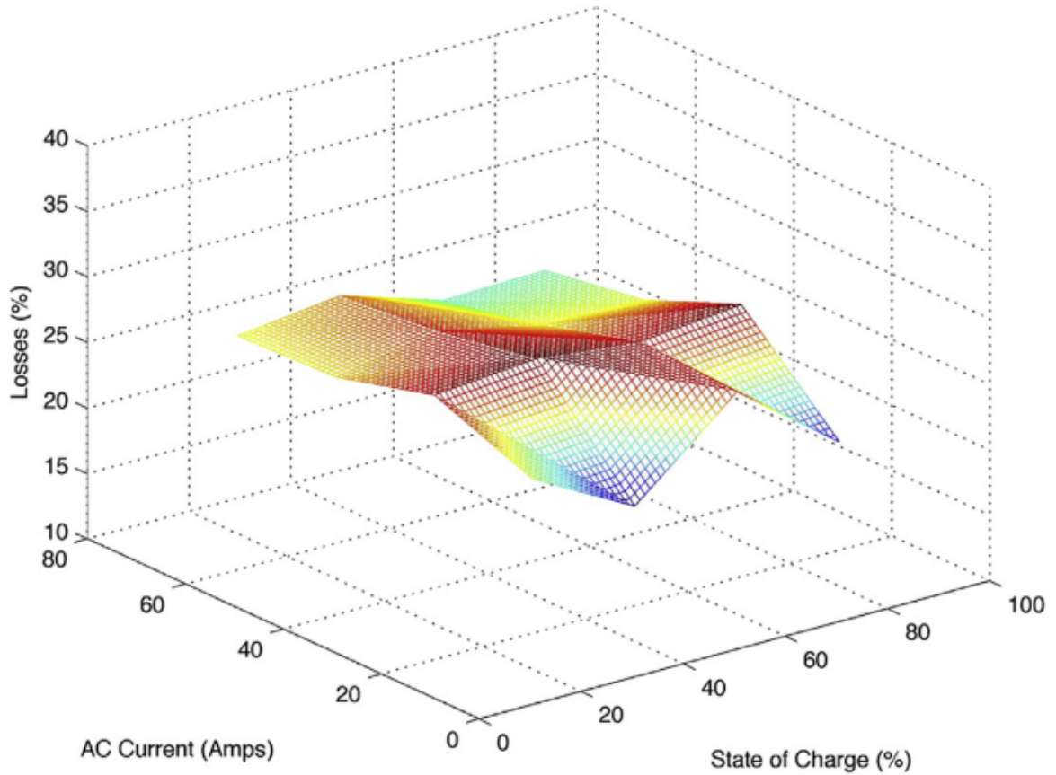
Figure 3.6: Charge Efficiency Dependency Map ( 1 - \eta_{(SOC,i)} )
