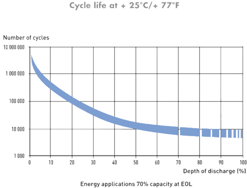
Figure 2.15: Cycle Life vs Depth of Discharge (DoD) from Saft Datasheet [136]
