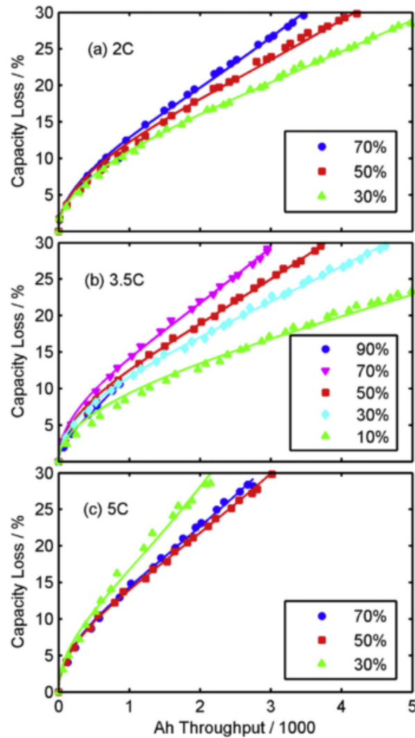
Figure 2.16: Depth of Discharge (DoD) Effect on Capacity Fade compared by Ah throughput [98]
