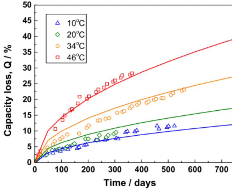
Figure 2.23: Simulations of Calendar Aging prediction model (line) are compared with experimental data (markers) for all four temperatures (10, 20, 34, and 46 °C) for LMO-NMC chemistry cell [98].
