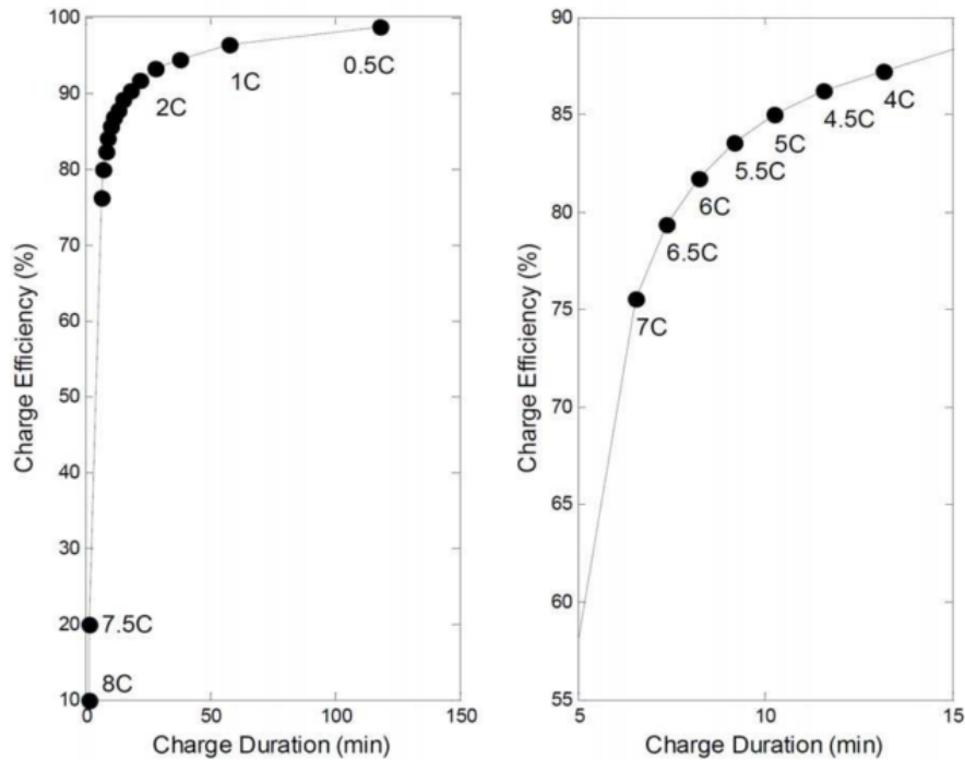
Figure 2.14: C-rate Effect on Charge Efficiency (magnified view in right panel) [129]
