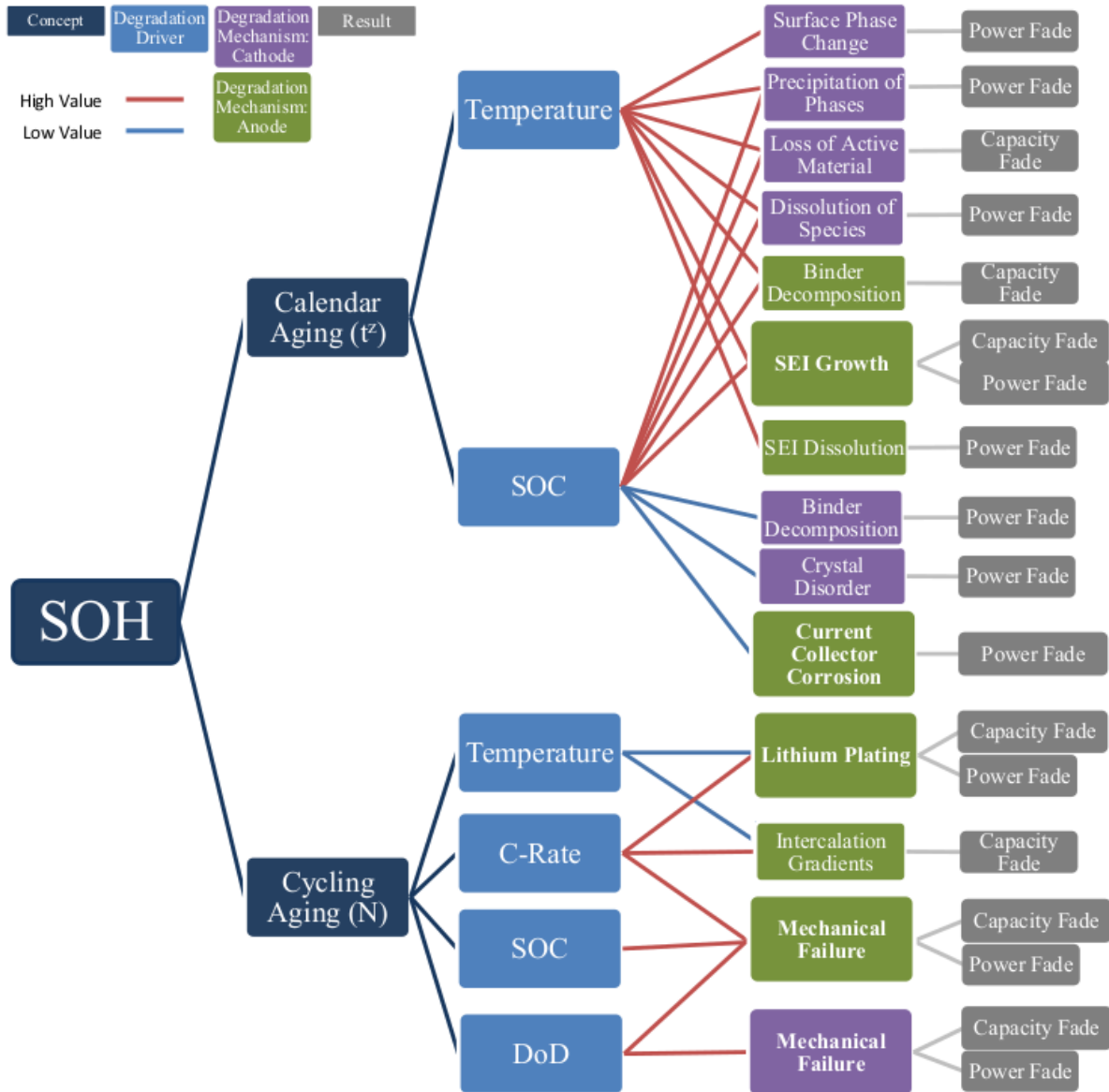
Figure 2.6: Battery Degradation Flowchart:
