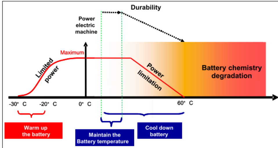
Figure 2.8: Generalized Thermal Management Strategy [93].
