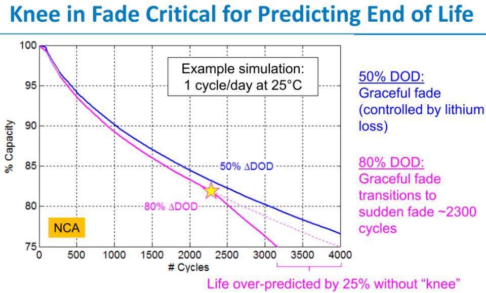
Figure 2.18: Knee Region Visualization for NCA Chemistry [139].
