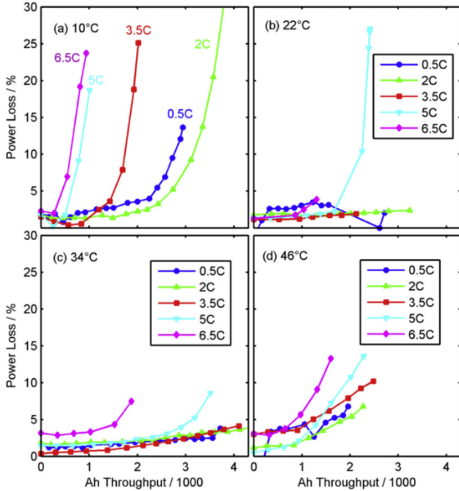
Figure 2.11: C-rate Effect on Power Fade [98]
