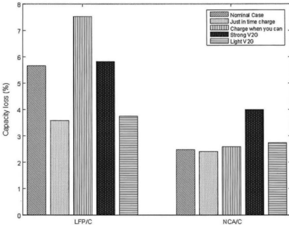
Figure 3.4: Comparison of Capacity Loss due to various charging and V2G profiles for LFP and NCA Battery Chemistries [159].
