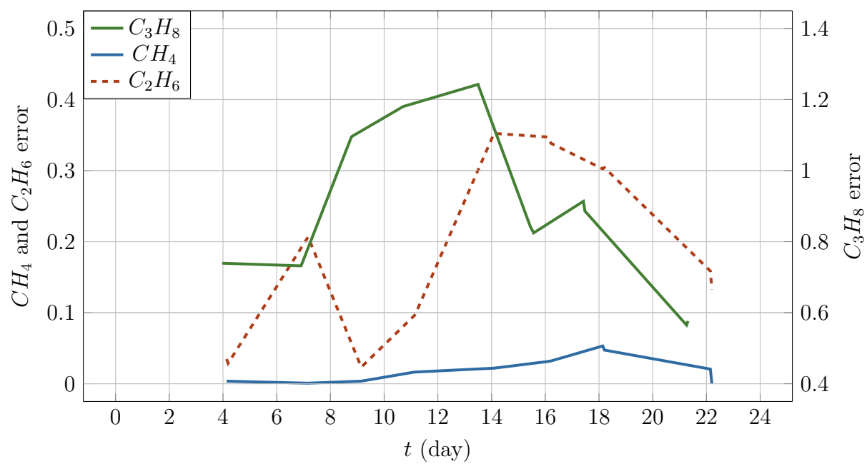
Figure 1.37: Error evolution 2
