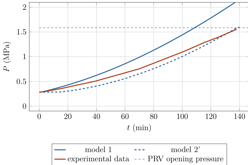
Figure 1.21: Pressure evolution
