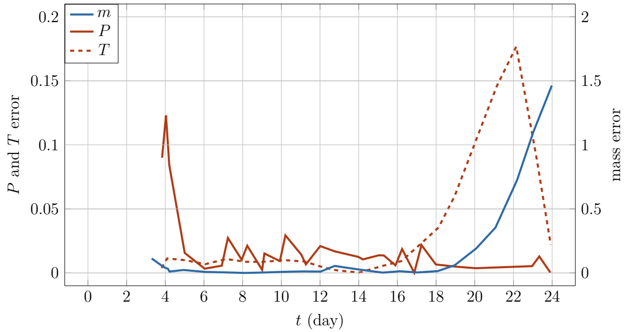
Figure 1.36: Error evolution 1
