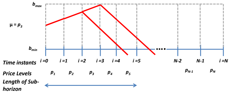
Figure 3.7: Battery charge level trajectory for \mu = p_3
