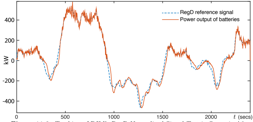
Figure 11.9: Tracking of PJM's RegD Normalized Signal Test in Scenario A2.
