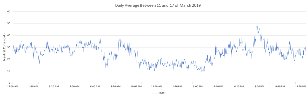
Figure 13.21: Neutral currents, averaged by minute between 11 and 17 of March 2019
