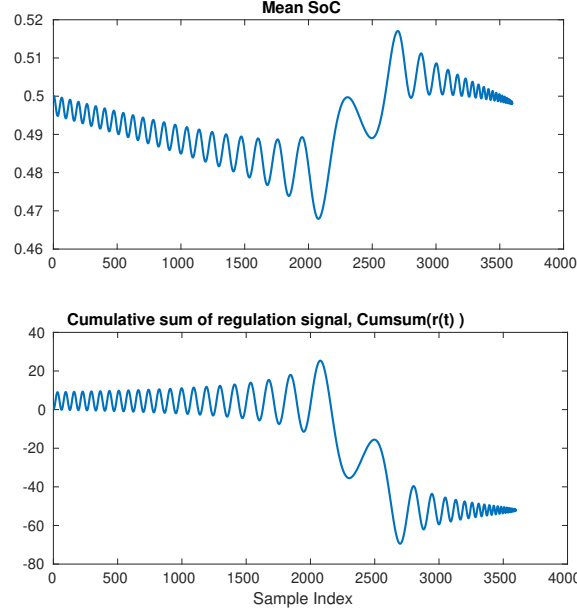
Figure 12.4: SoC recovery due to drift compensation
