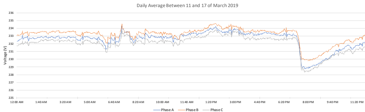
Figure 13.20: Voltage per phase, averaged by minute between 11 and 17 of March 2019
