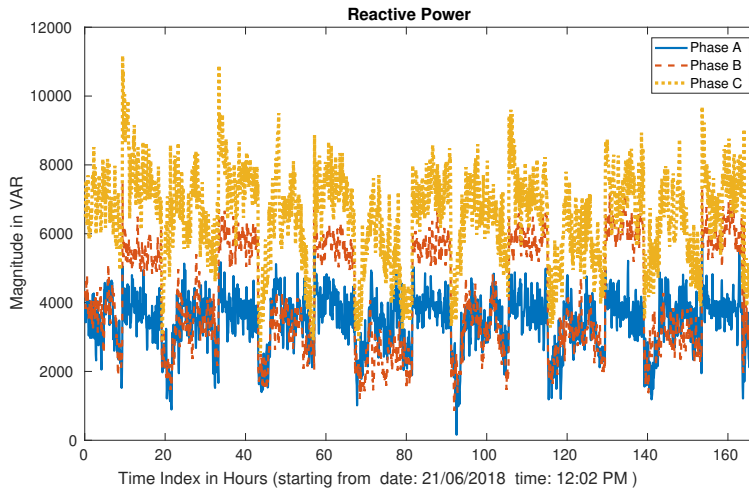
Figure 6.10: Reactive power seen from the substation
