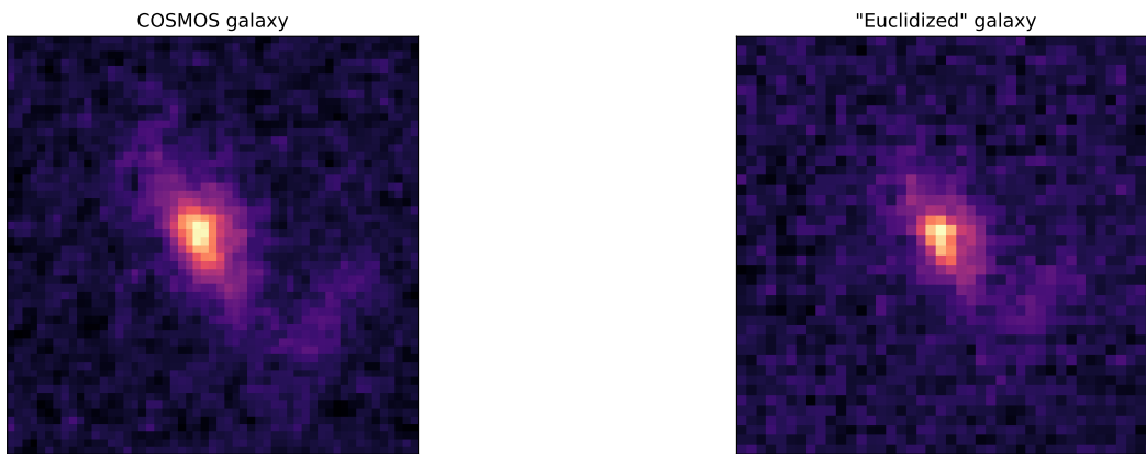
Figure 2.8: “Euclidization” of a COSmic evOLution Survey (COSMOS) galaxy. The galaxy, as observed by HST , is shown on the left; its reprocessed version, as it would appear if observed by VIS , on the right.
