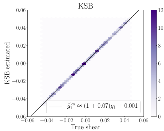
Figure 3.19: 2D density of true and measured shear; the colours correspond to the number of occurrences of measured shear values when using the “known” PSF, each from approximately 10 000 galaxies, for the corresponding input shear. The line shows the best fit linear regression, yielding the bias values. Shapes were measured with KSB.
