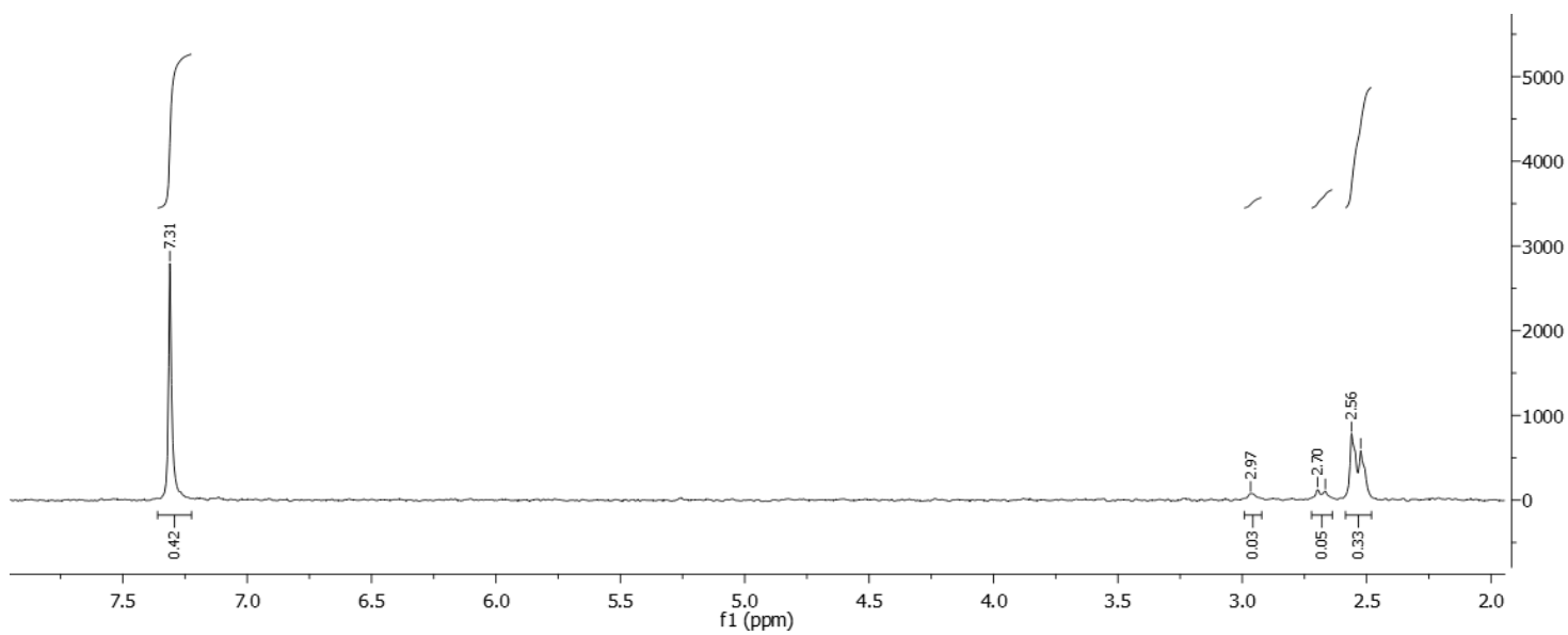
3 H-NMR spectrum of 27*
