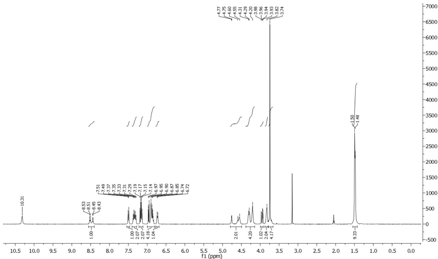
^1\text{H}\text{-NMR} spectrum of the non-deuterated starting material
