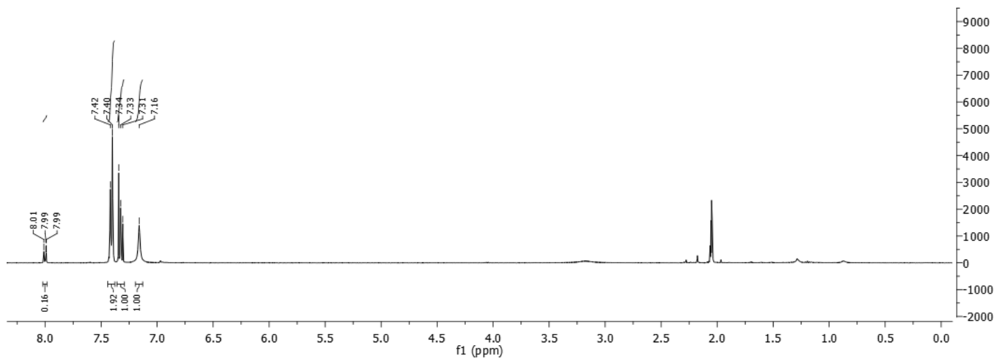
^1\text{H-NMR} spectrum of 33
