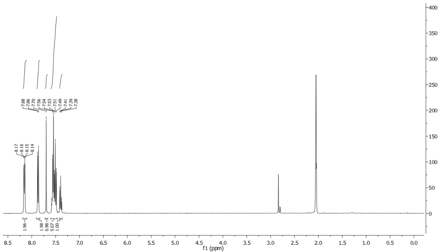
1 H-NMR spectrum of the non-deuterated starting material
