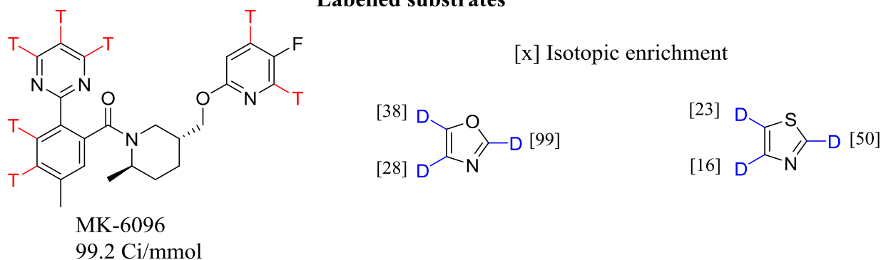
Figure 33. Dinuclear Ni(I)-complex with bulky substituents as HIE catalyst for the efficient tritiation of pharmaceuticals and the deuteration of oxazole and thiazole
