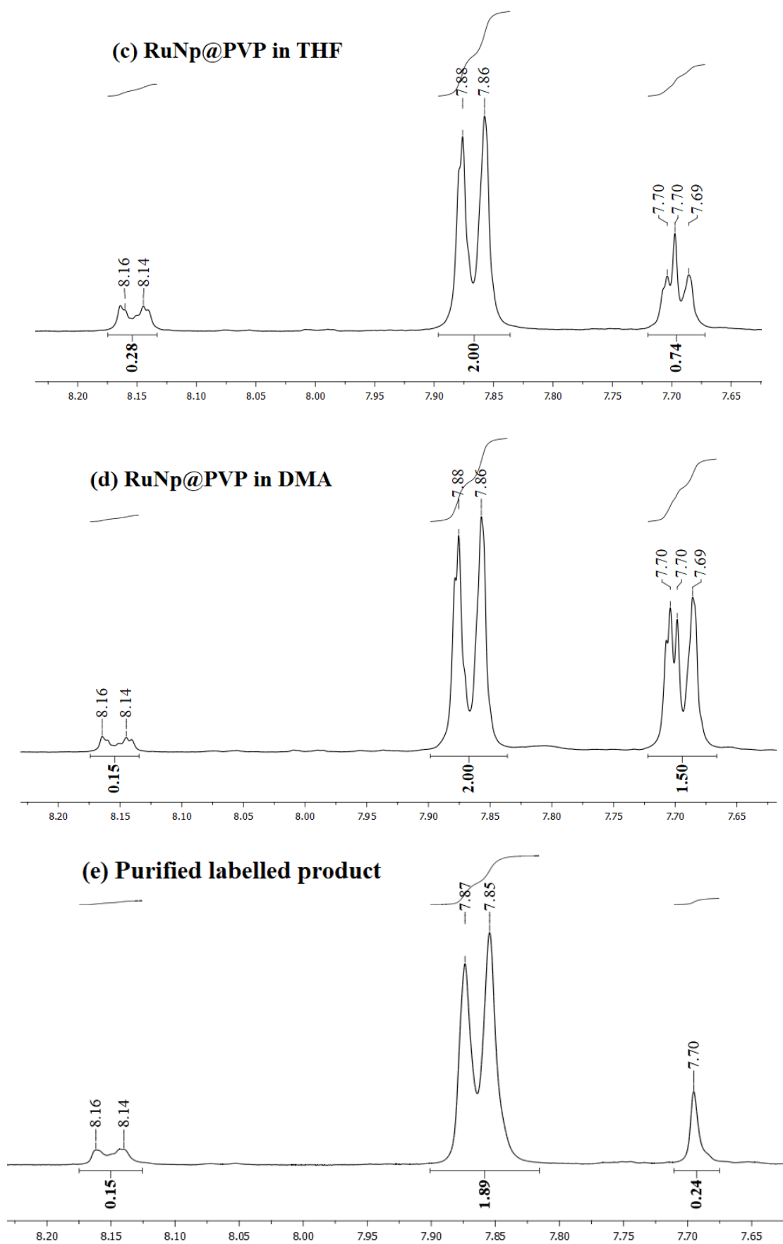
Figure 50. (a)-(d) ^1\text{H} -NMR spectra of the crude mixtures after HIE on 2,5-diphenyloxazole with different Ru catalysts (e) spectrum after HPLC-purification (chemical shifts in ppm)
