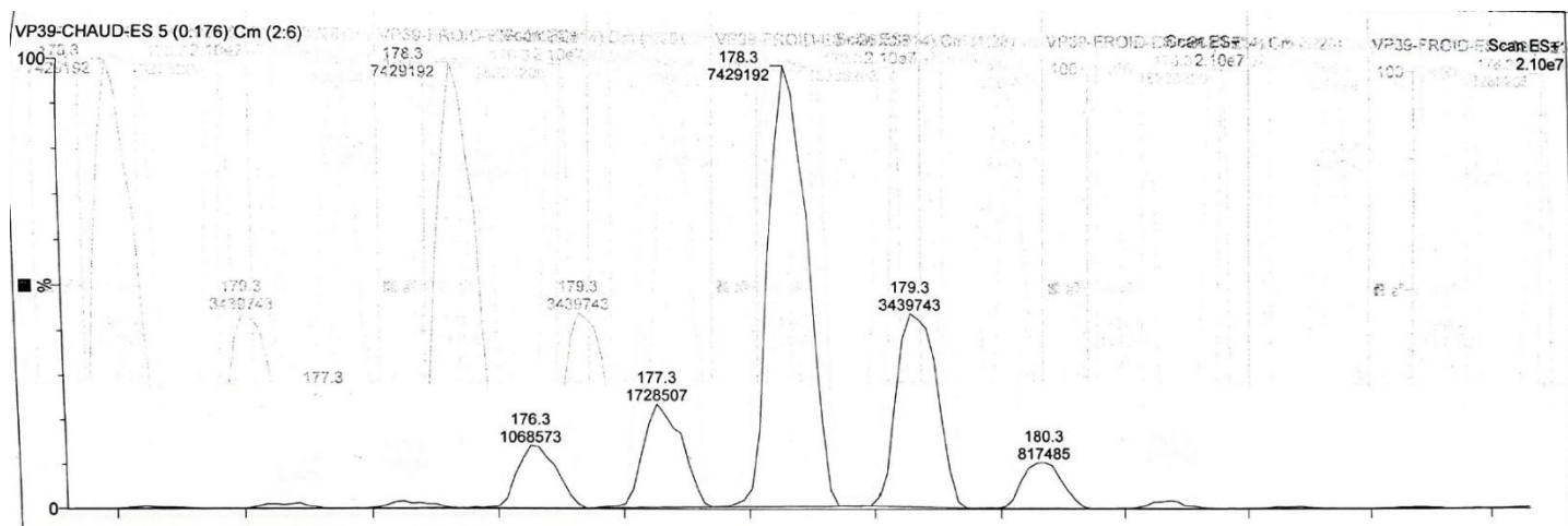
ESI-spectrum of 16
