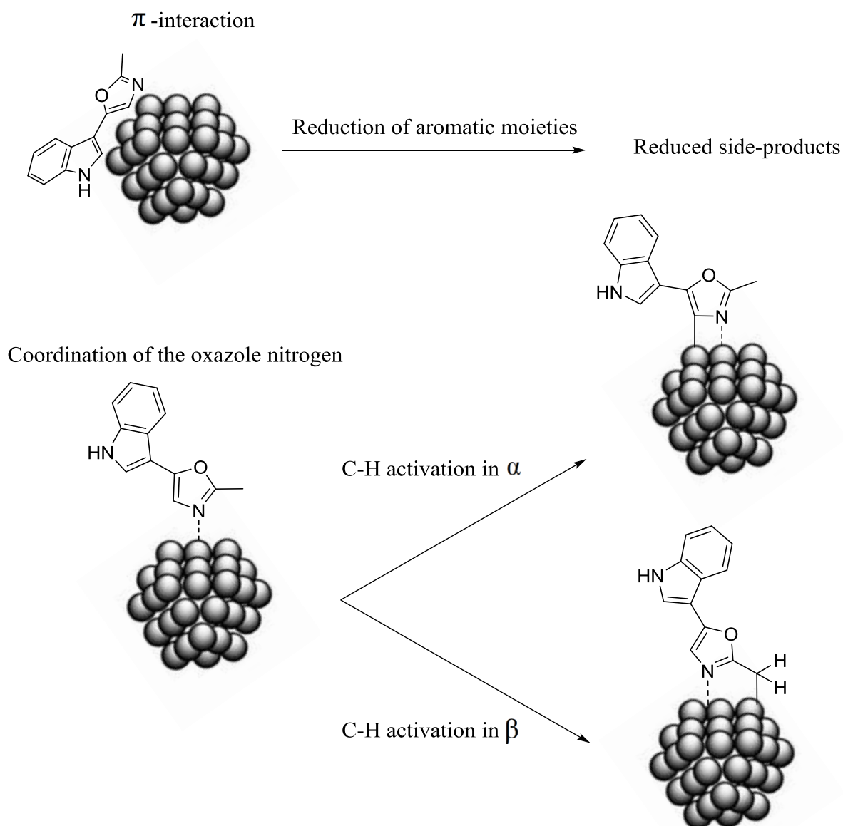
Figure 66. Propositions of favored key-intermediates for the RuNp@PVP catalyzed deuteration of pimprinine (a) without and (b) with \text{Cs}_2\text{CO}_3
