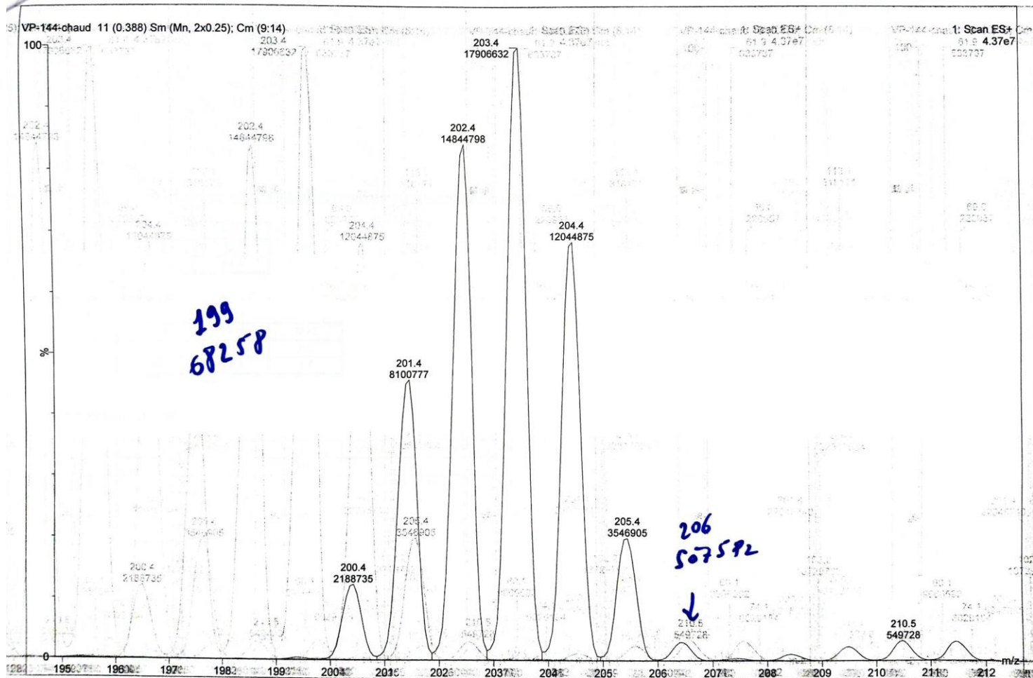
ESI-spectrum of 25I
