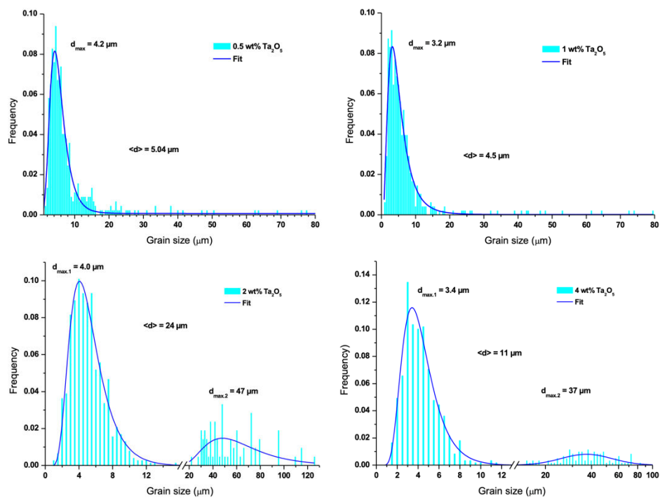
Figure 71. Grain size distributions of the commercial spinel doped with 0.5, 1, 2 and 4 wt% of \text{Ta}_2\text{O}_5 .
