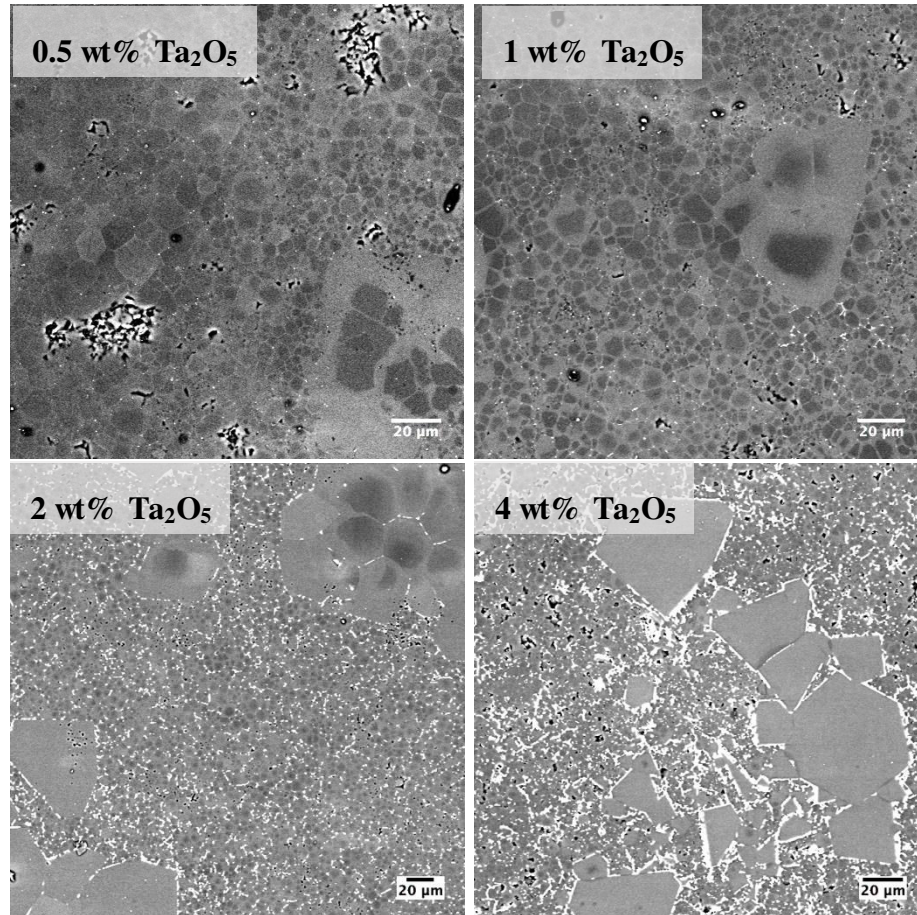
Figure 70. Microstructures of the commercial spinel doped with 0.5, 1, 2 and 4 wt% of \text{Ta}_2\text{O}_5 .
