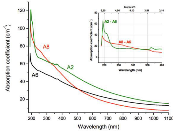
Figure 47. Absorption coefficient for samples A2 (0.8 mm), A6 (1.1 mm) and A8 (0.8 mm).
