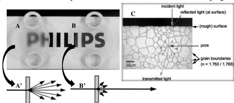
Figure 12. Translucent (A and A') and transparent (B and B') alumina. Path of light in a polycrystalline material (C). [111]
