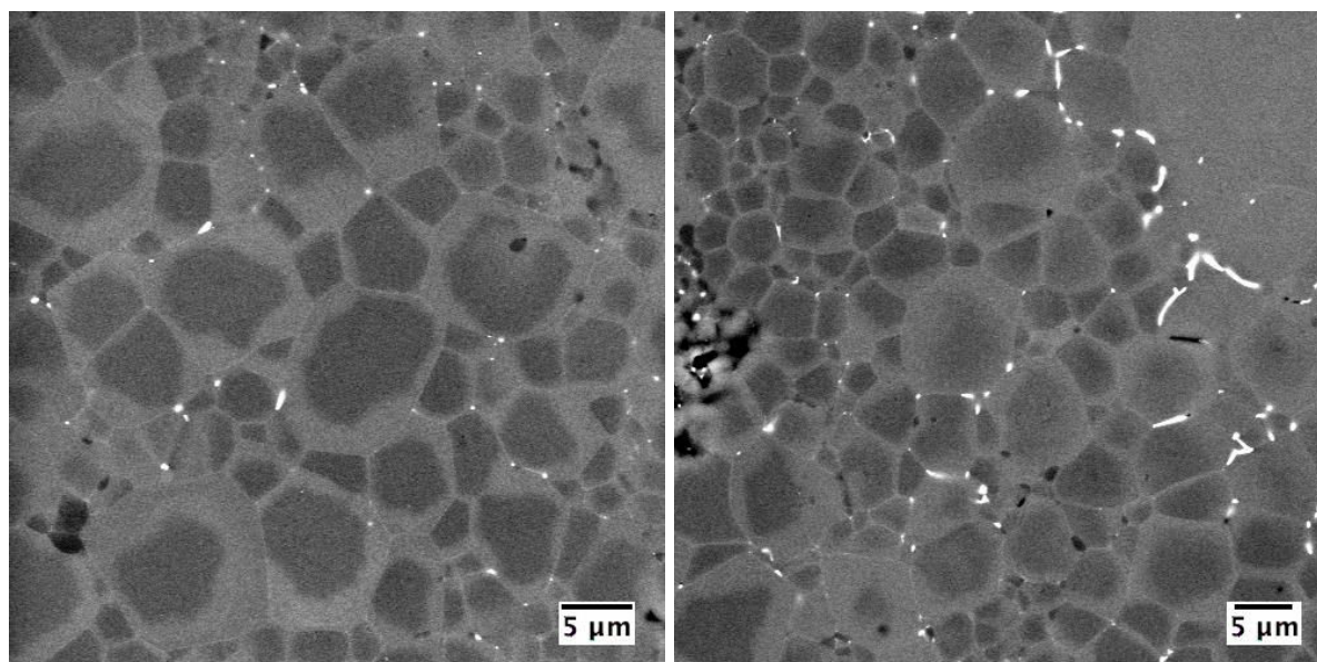
Figure 72. SEM micrographs of spinel doped by 0.5 wt% (left) and 1 wt% (right) \text{Ta}_2\text{O}_5 .
