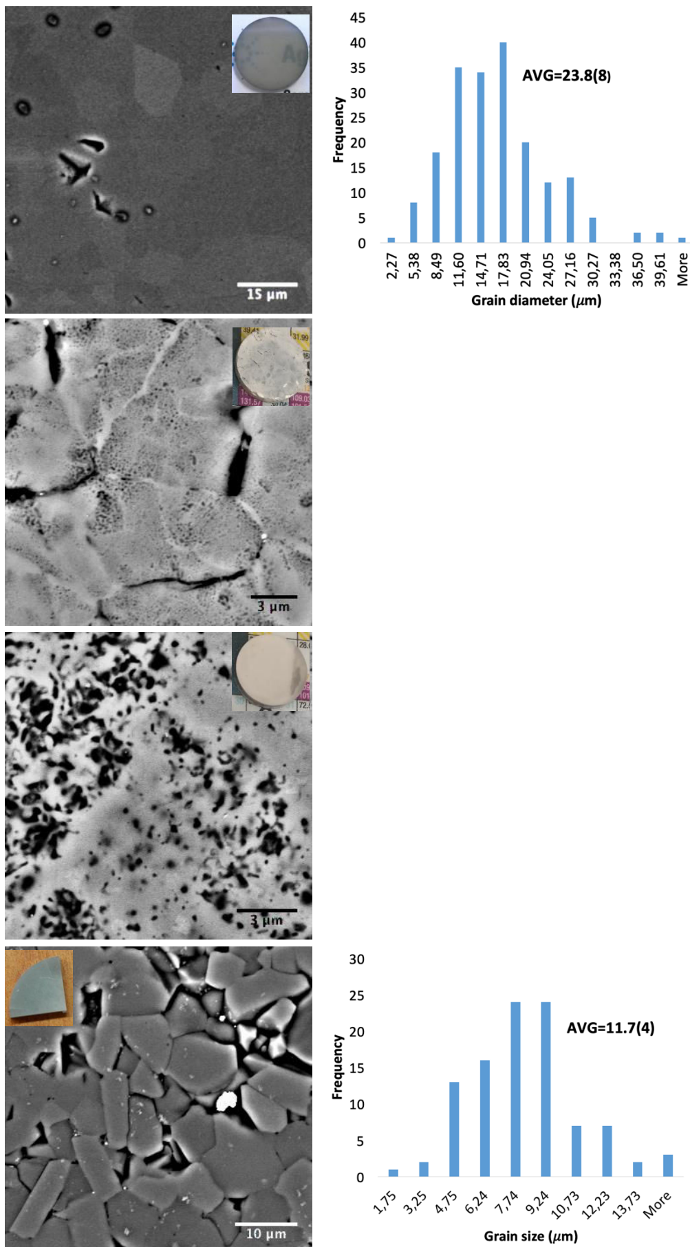
Figure 36. Morphology and grain size distribution of A9 - A12.
