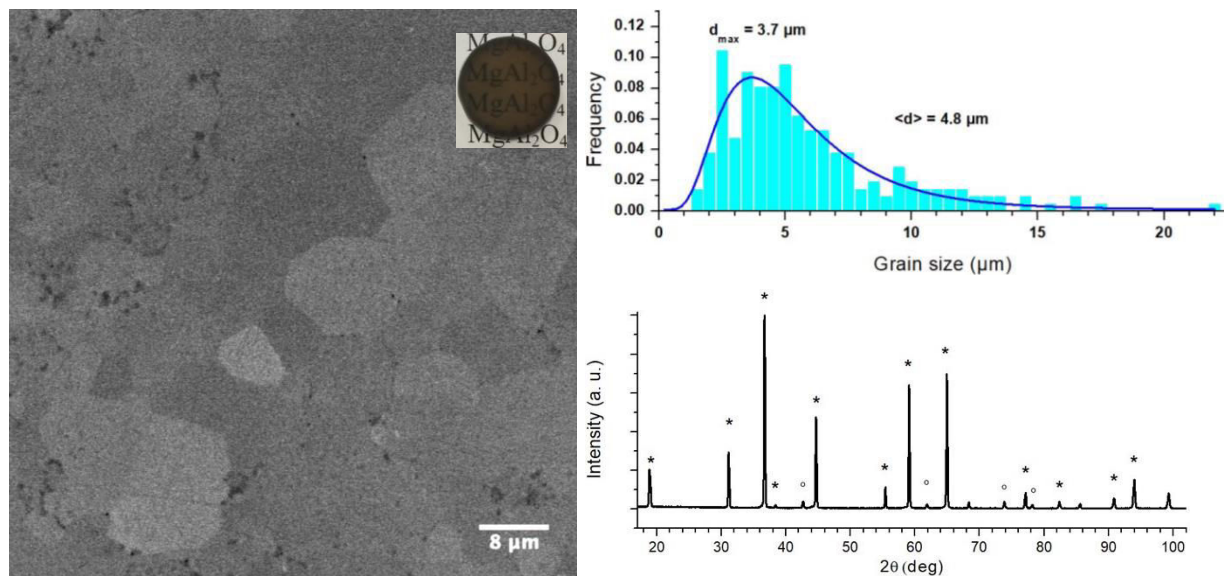
Figure 51. Results of the dilatometric study: SEM micrograph, grain size distribution and XRD profile (* denotes spinel and ° MgO (periclase)).
