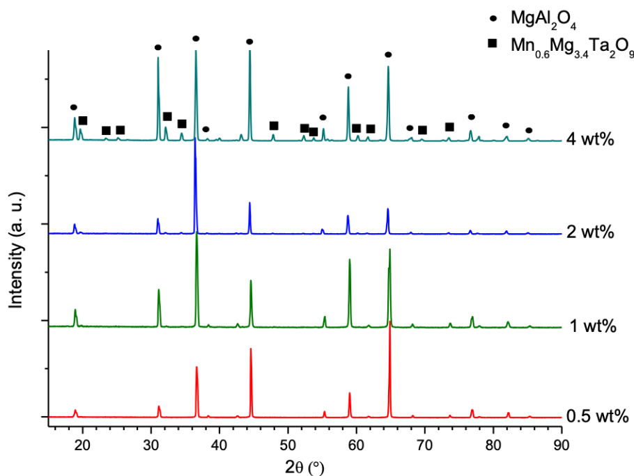
Figure 75. XRD patterns of commercial spinels sintered with 0.5, 1, 2 and 4 wt% of \text{Ta}_2\text{O}_5 .
