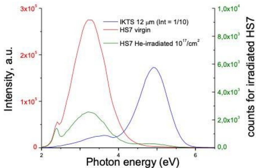
Figure 76. CL spectra of virgin and irradiated commercial spinel sintered with added 1 wt% \text{Ta}_2\text{O}_5 .
