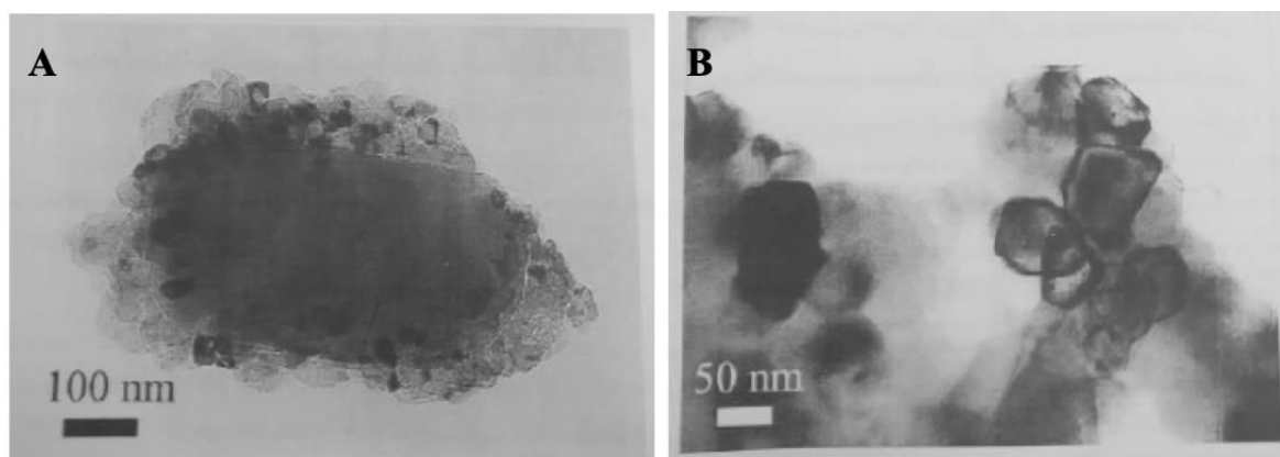
Figure 19. A: A big \alpha -alumina crystallite covered by forming small magnesia crystallites after calcination at 800^\circ\text{C} for 4h. B: Spinel crystallites formed after 7 days at 1000^\circ\text{C} . [54]
