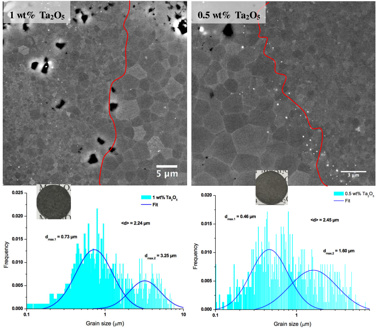
Figure 77. Ceramics sintered from stoichiometric powder at 1370^\circ\text{C} by the long cycle with 1 wt% and 0.5 wt% added \text{Ta}_2\text{O}_5 and their grain size distributions. The red lines separate smaller and bigger grains.
