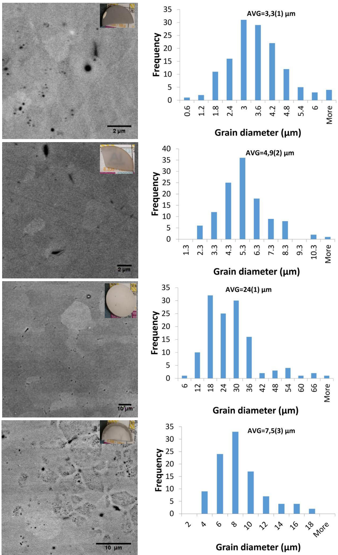
Figure 32. SEM micrographs of Al-A4 (top to bottom) with the grain size distributions and optical images.
