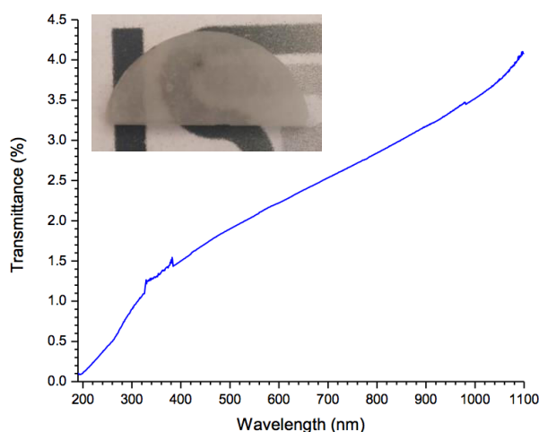
Figure 69. Transmittance of impregnation sample sintered at 1450°C via the long cycle.
