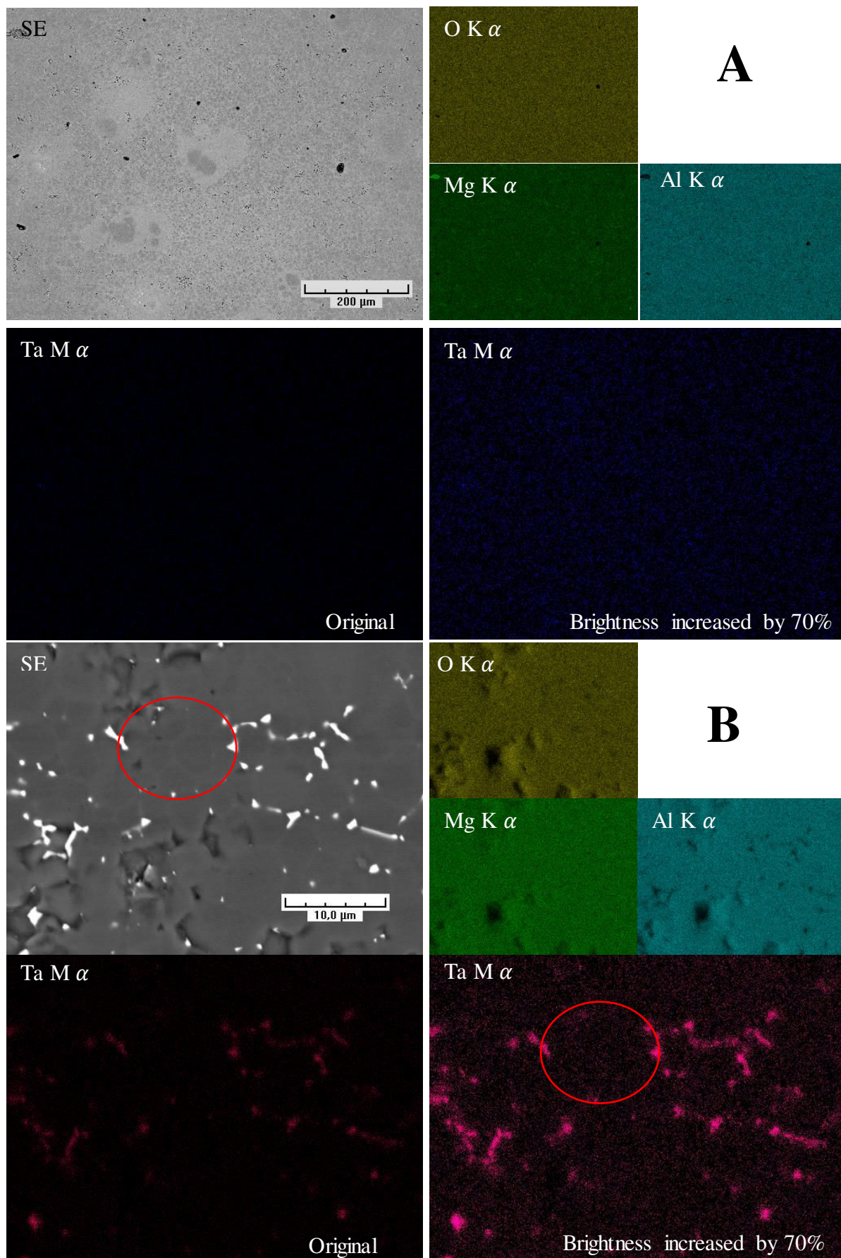
Figure 74. EDX analysis of spinel doped by 0.5 wt % (A) and 1 wt% (B) \text{Ta}_2\text{O}_5 .
