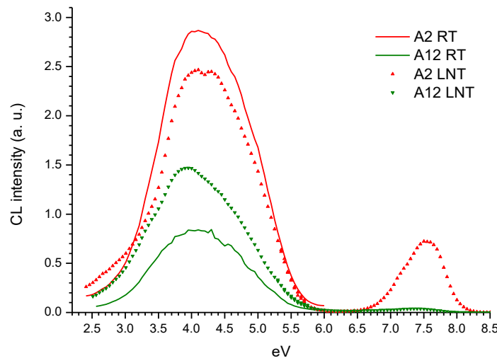
Figure 48. CL spectra of A2 and A12 at room temperature (RT) and liquid nitrogen temperature (LNT).
